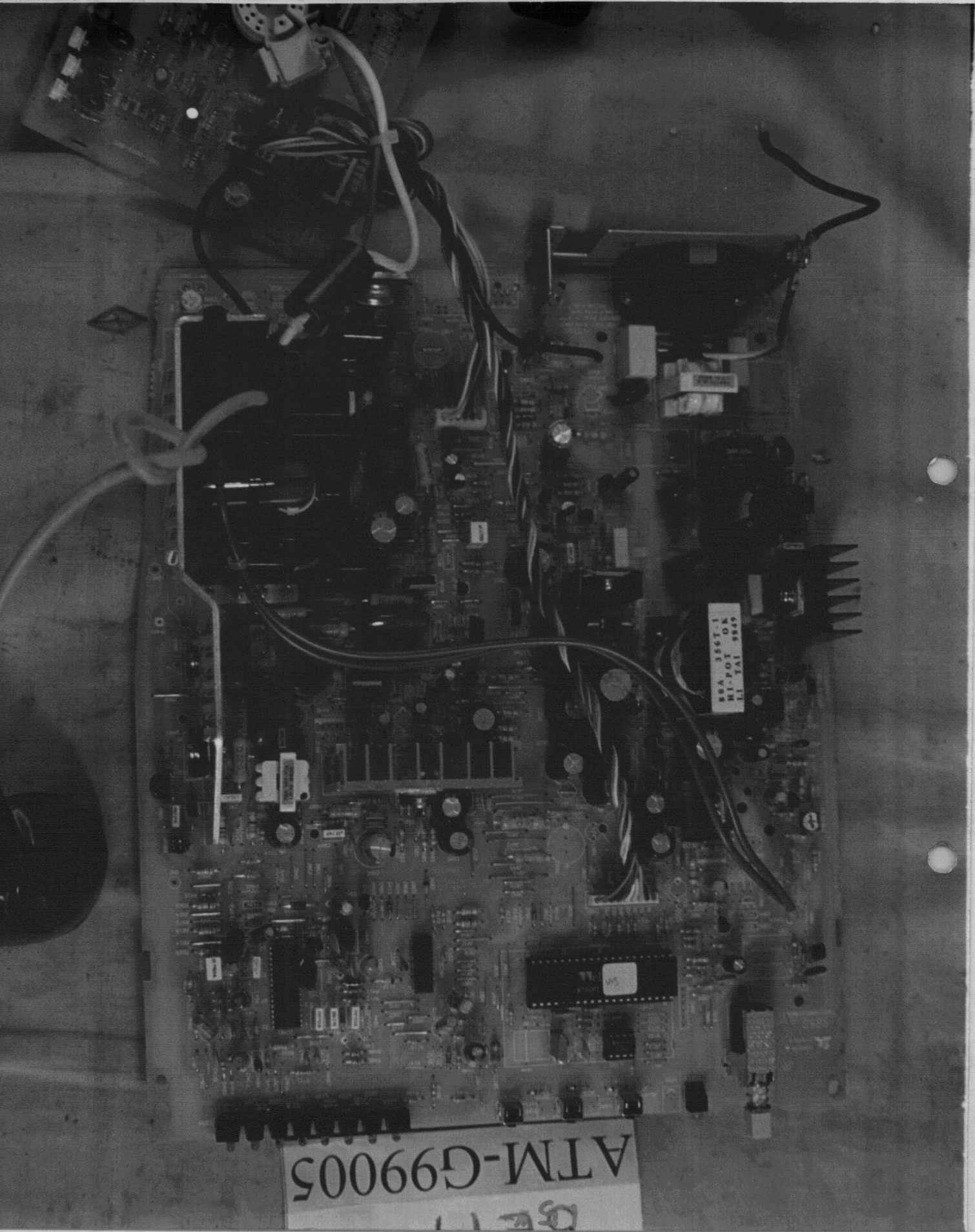
Figure 4 Main Board (Component Side)
