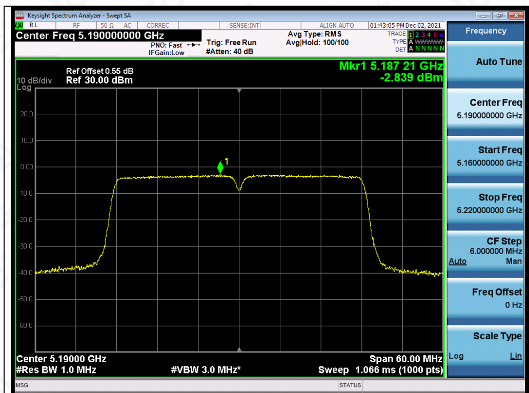
Test Graph 802.11n40 ANT1 5190 MCS0 PSD
