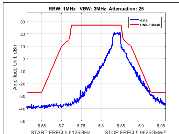
Plot 420. Undesirable Emissions, UNII-3 Emissions Mask, 10M, 5840MHz, 2Para
