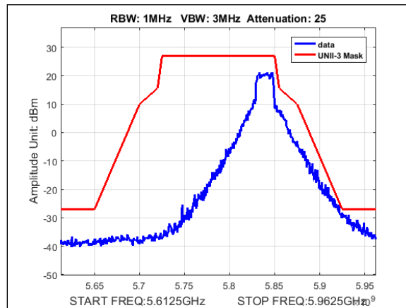
Plot 419. Undesirable Emissions, UNII-3 Emissions Mask, 10M, 5840MHz, 2Panel
