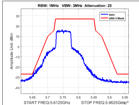
Plot 436. Undesirable Emissions, UNII-3 Emissions Mask, 40M, 5750MHz, 2Para
