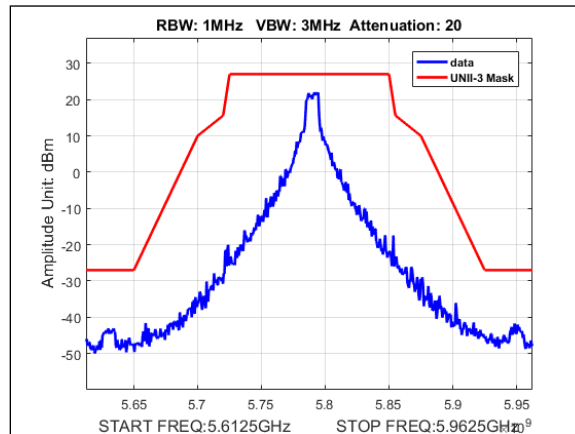
Plot 402. Undesirable Emissions, UNII-3 Emissions Mask, 5M, 5785MHz, 80Omni
