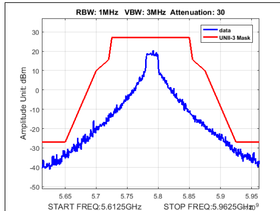
Plot 413. Undesirable Emissions, UNII-3 Emissions Mask, 10M, 5785MHz, 8Omni
