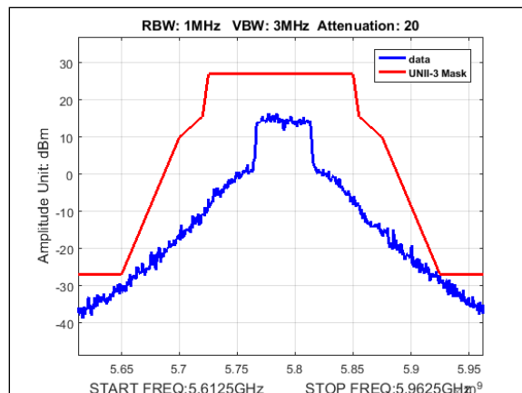
Plot 438. Undesirable Emissions, UNII-3 Emissions Mask, 40M, 5785MHz, 90Sector
