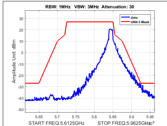
Plot 406. Undesirable Emissions, UNII-3 Emissions Mask, 5M, 5845MHz, 90Sector
