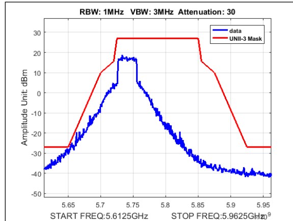
Plot 421. Undesirable Emissions, UNII-3 Emissions Mask, 20M, 5740MHz, 8Omni
