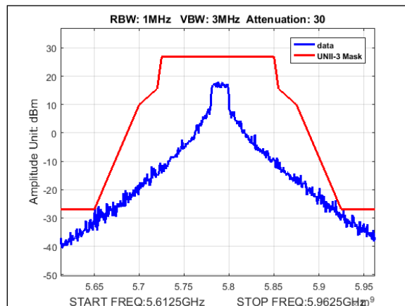
Plot 414. Undesirable Emissions, UNII-3 Emissions Mask, 10M, 5785MHz, 90Sector
