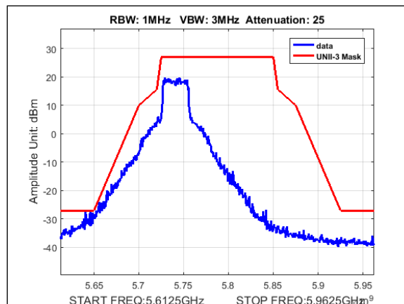
Plot 423. Undesirable Emissions, UNII-3 Emissions Mask, 20M, 5740MHz, 2Panel
