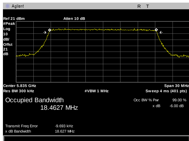
Plot 457. 6 dB Occupied Bandwidth, BW 20MHz, 5835MHz
