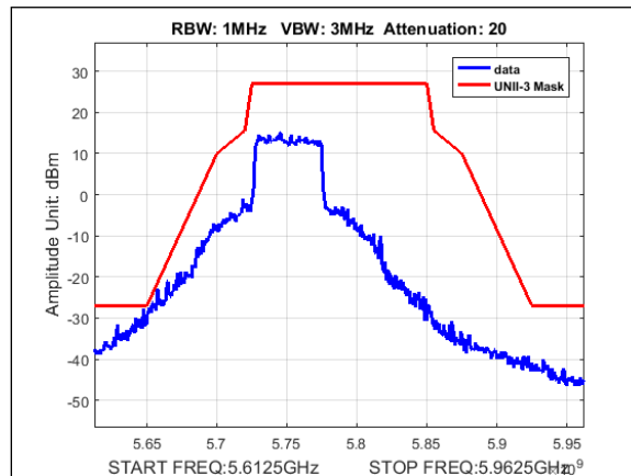
Plot 434. Undesirable Emissions, UNII-3 Emissions Mask, 40M, 5750MHz, 90Sector
