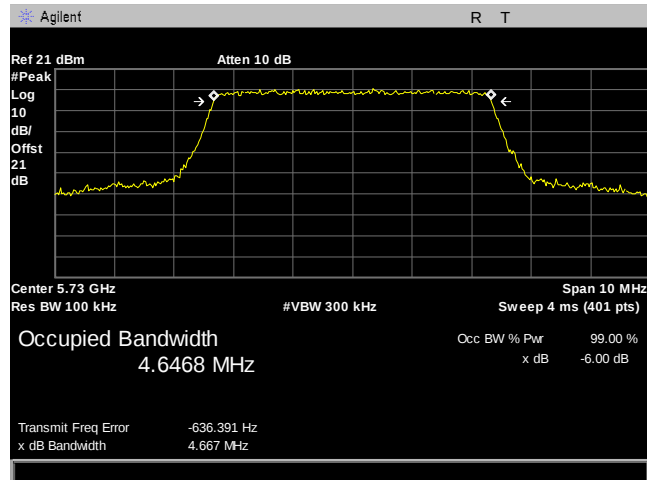
Plot 449. 6 dB Occupied Bandwidth, BW 5MHz, 5730MHz
