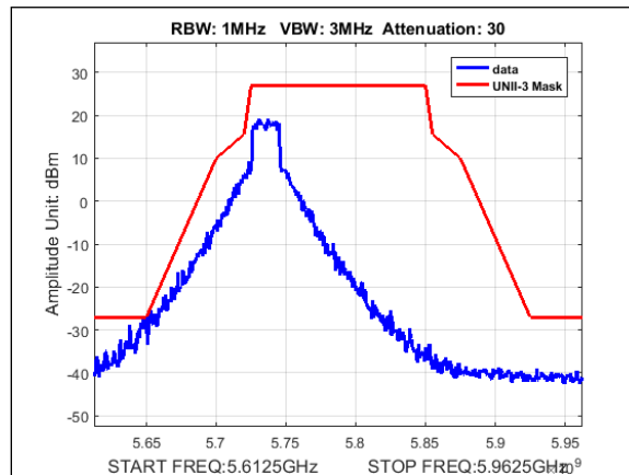
Plot 410. Undesirable Emissions, UNII-3 Emissions Mask, 10M, 5735MHz, 90Sector
