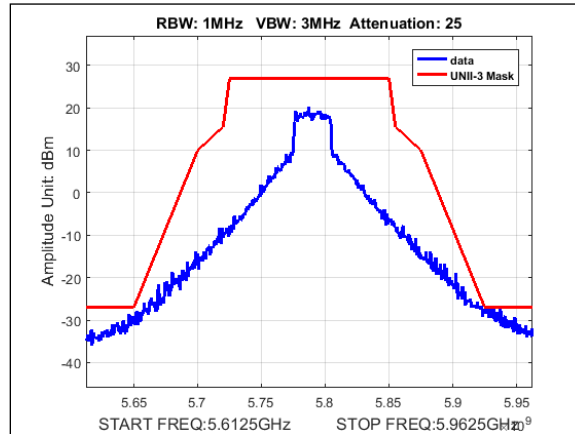
Plot 427. Undesirable Emissions, UNII-3 Emissions Mask, 20M, 5785MHz, 2Panel
