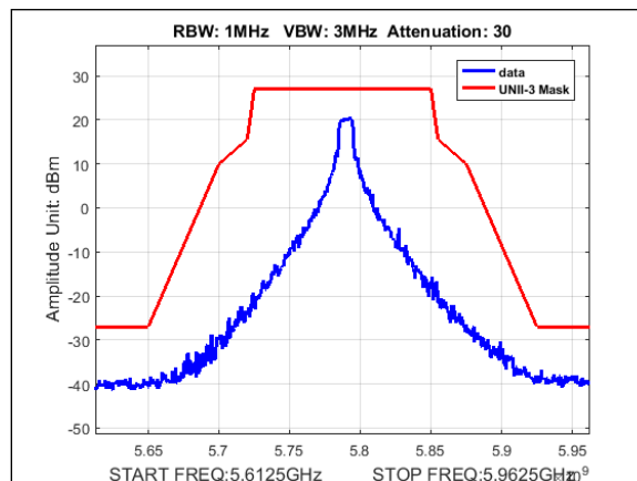
Plot 403. Undesirable Emissions, UNII-3 Emissions Mask, 5M, 5785MHz, 90Sector
