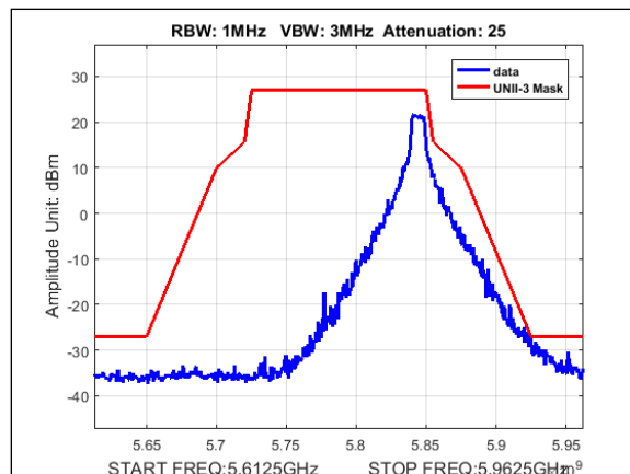
Plot 408. Undesirable Emissions, UNII-3 Emissions Mask, 5M, 5845MHz, 2Para
