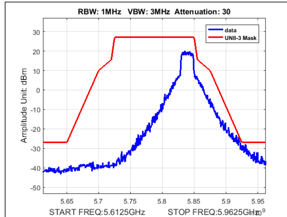
Plot 418. Undesirable Emissions, UNII-3 Emissions Mask, 10M, 5840MHz, 90Sector
