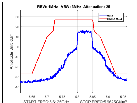
Plot 444. Undesirable Emissions, UNII-3 Emissions Mask, 40M, 5825MHz, 2Para
