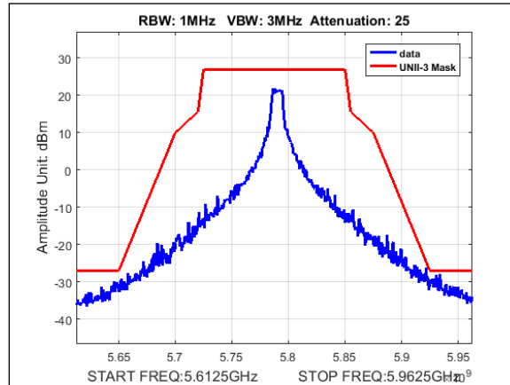
Plot 404. Undesirable Emissions, UNII-3 Emissions Mask, 5M, 5785MHz, 2Panel
