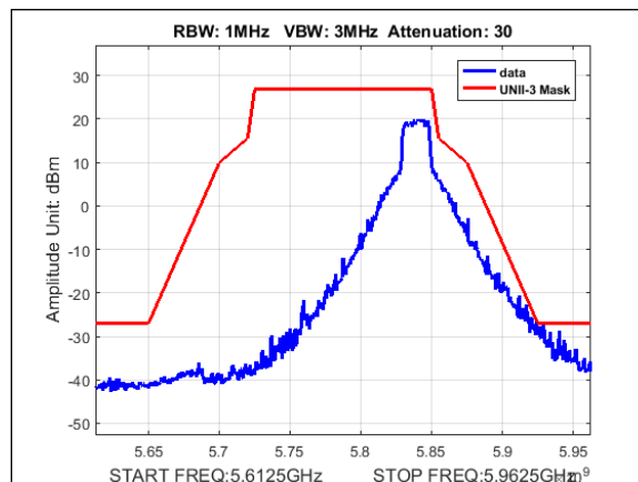
Plot 417. Undesirable Emissions, UNII-3 Emissions Mask, 10M, 5840MHz, 8Omni
