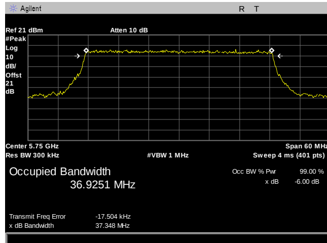
Plot 458. 6 dB Occupied Bandwidth, BW 40MHz, 5750MHz
