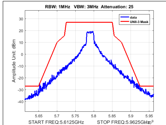
Plot 415. Undesirable Emissions, UNII-3 Emissions Mask, 10M, 5785MHz, 2Panel
