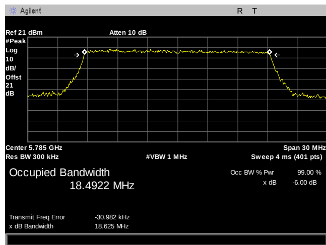
Plot 456. 6 dB Occupied Bandwidth, BW 20MHz, 5785MHz
