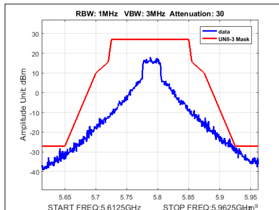
Plot 426. Undesirable Emissions, UNII-3 Emissions Mask, 20M, 5785MHz, 90Sector
