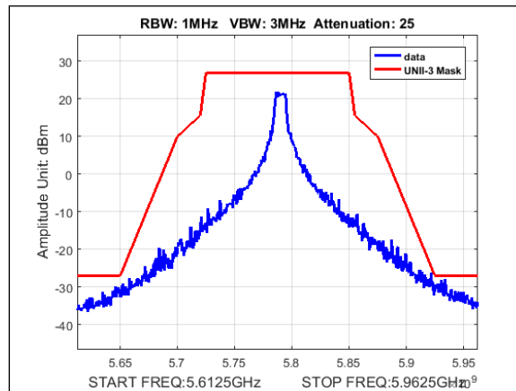
Plot 404. Undesirable Emissions, UNII-3 Emissions Mask, 5M, 5785MHz, 2Para
