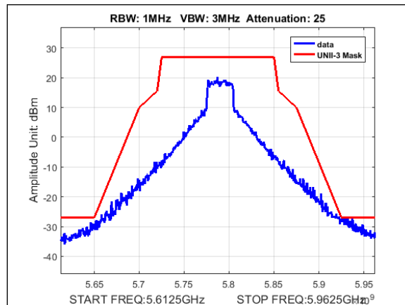
Plot 428. Undesirable Emissions, UNII-3 Emissions Mask, 20M, 5785MHz, 2Para
