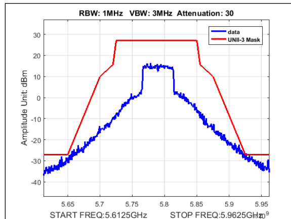
Plot 437. Undesirable Emissions, UNII-3 Emissions Mask, 40M, 5785MHz, 8Omni
