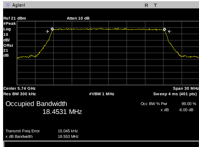
Plot 455. 6 dB Occupied Bandwidth, BW 20MHz, 5740MHz
