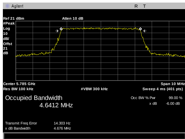
Plot 450. 6 dB Occupied Bandwidth, BW 5MHz, 5785MHz
