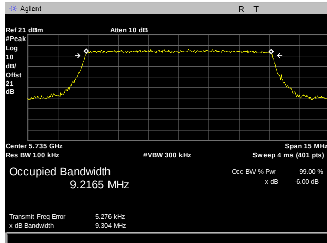
Plot 452. 6 dB Occupied Bandwidth, BW 10MHz, 5735MHz
