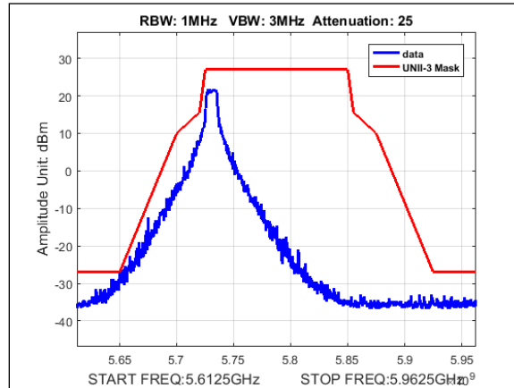
Plot 401. Undesirable Emissions, UNII-3 Emissions Mask, 5M, 5730MHz, 2Para
