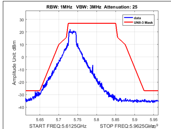
Plot 412. Undesirable Emissions, UNII-3 Emissions Mask, 10M, 5735MHz, 2Para
