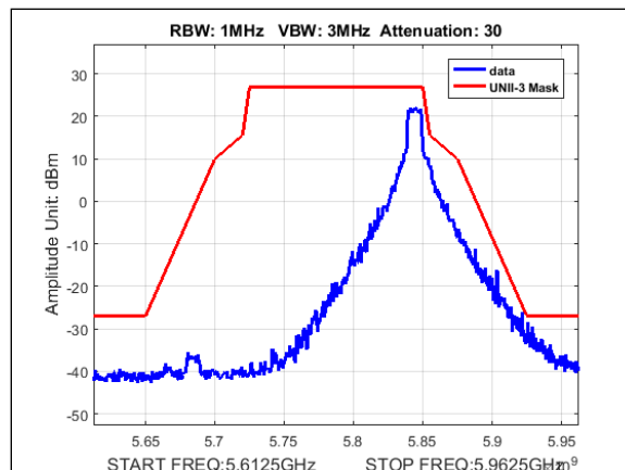
Plot 405. Undesirable Emissions, UNII-3 Emissions Mask, 5M, 5845MHz, 80mni
