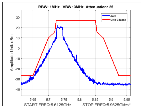
Plot 411. Undesirable Emissions, UNII-3 Emissions Mask, 10M, 5735MHz, 2Panel
