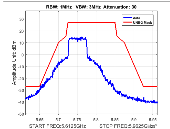
Plot 433. Undesirable Emissions, UNII-3 Emissions Mask, 40M, 5750MHz, 8Omni
