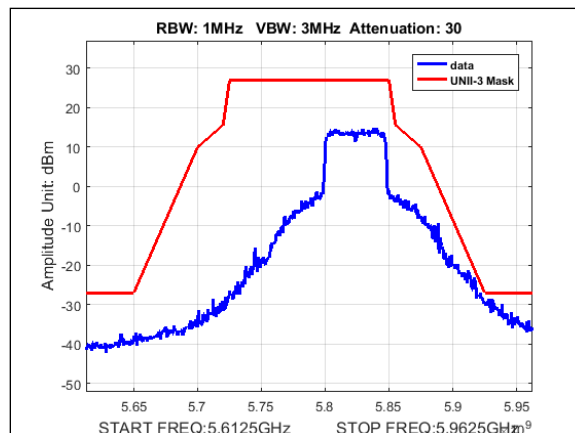
Plot 441. Undesirable Emissions, UNII-3 Emissions Mask, 40M, 5825MHz, 8Omni
