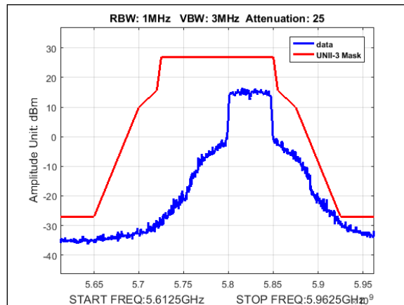
Plot 443. Undesirable Emissions, UNII-3 Emissions Mask, 40M, 5825MHz, 2Panel
