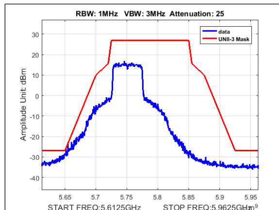
Plot 435. Undesirable Emissions, UNII-3 Emissions Mask, 40M, 5750MHz, 2Panel
