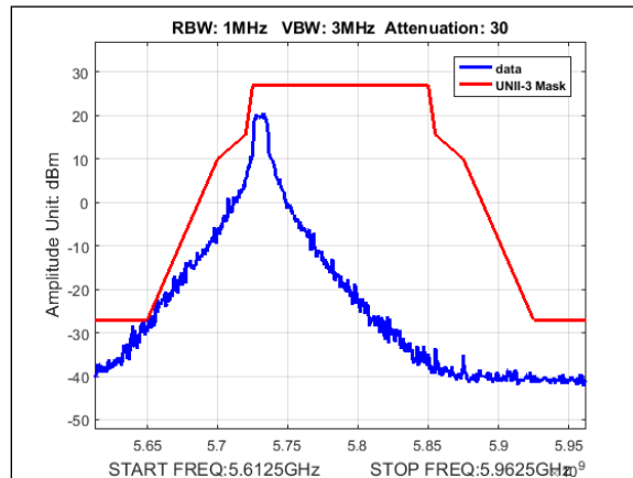
Plot 399. Undesirable Emissions, UNII-3 Emissions Mask, 5M, 5730MHz, 90Sector
