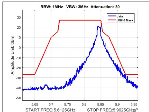
Plot 407. Undesirable Emissions, UNII-3 Emissions Mask, 5M, 5845MHz, 2Panel
