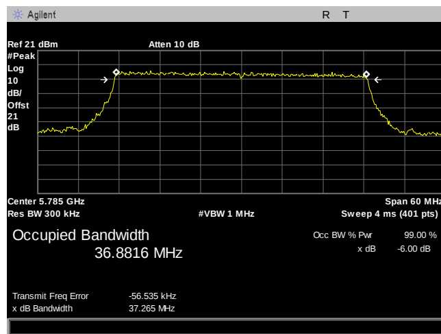
Plot 459. 6 dB Occupied Bandwidth, BW 40MHz, 5785MHz
