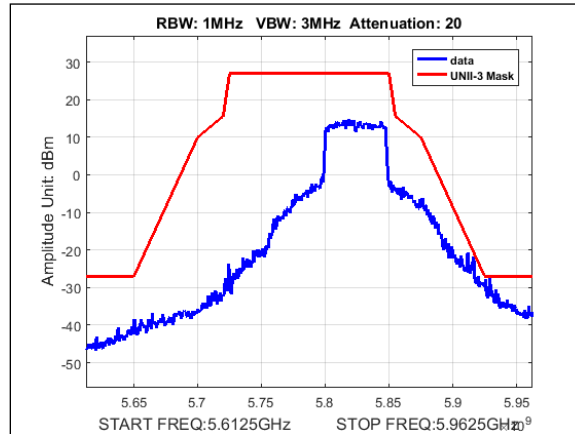
Plot 442. Undesirable Emissions, UNII-3 Emissions Mask, 40M, 5825MHz, 90Sector
