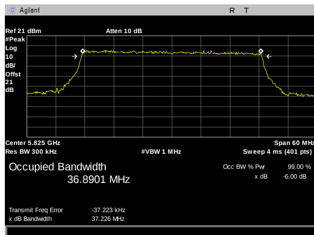
Plot 460. 6 dB Occupied Bandwidth, BW 40MHz, 5825MHz
