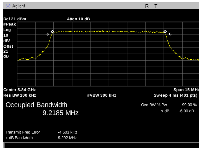
Plot 454. 6 dB Occupied Bandwidth, BW 10MHz, 5840MHz
