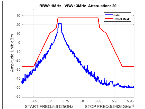
Plot 398. Undesirable Emissions, UNII-3 Emissions Mask, 5M, 5730MHz, 8Omni
