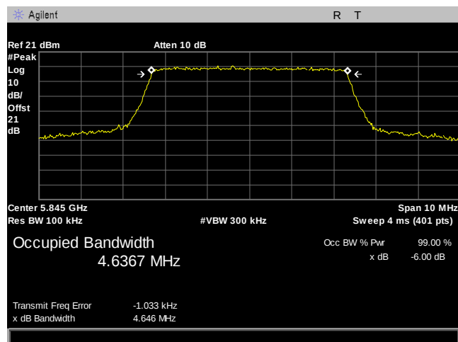
Plot 451. 6 dB Occupied Bandwidth, BW 5MHz, 5845MHz
