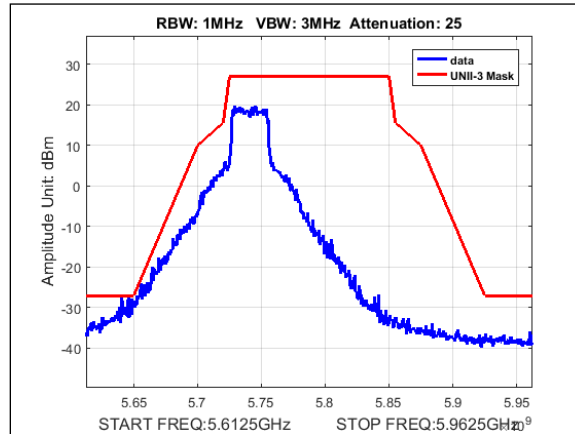
Plot 424. Undesirable Emissions, UNII-3 Emissions Mask, 20M, 5740MHz, 2Para
