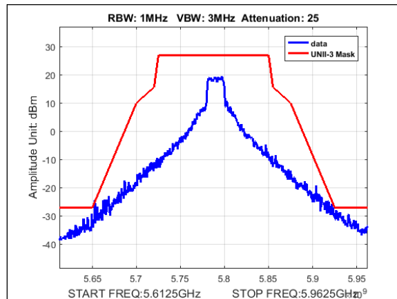
Plot 416. Undesirable Emissions, UNII-3 Emissions Mask, 10M, 5785MHz, 2Para
