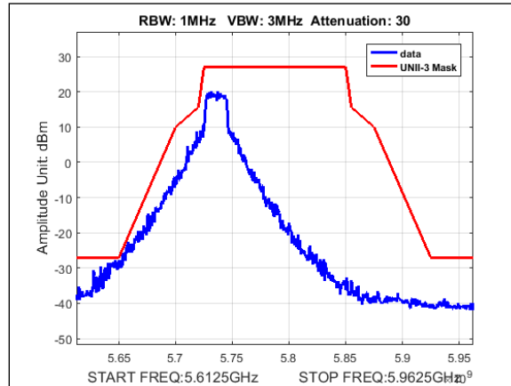
Plot 409. Undesirable Emissions, UNII-3 Emissions Mask, 10M, 5735MHz, 8Omni
