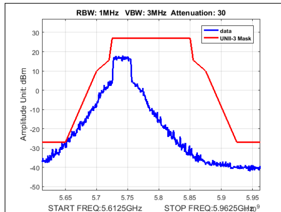
Plot 422. Undesirable Emissions, UNII-3 Emissions Mask, 20M, 5740MHz, 90Sector
