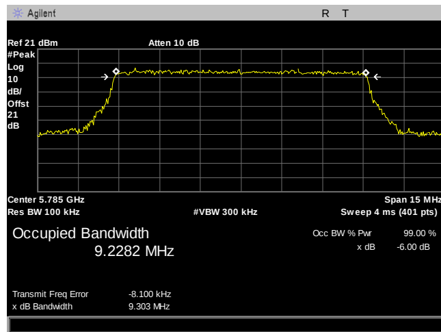
Plot 453. 6 dB Occupied Bandwidth, BW 10MHz, 5785MHz
