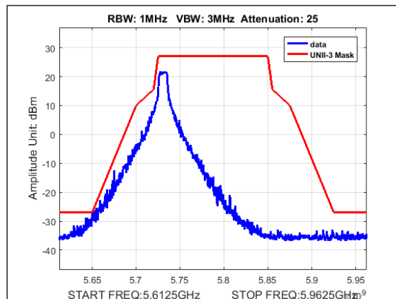
Plot 400. Undesirable Emissions, UNII-3 Emissions Mask, 5M, 5730MHz, 2Panel
