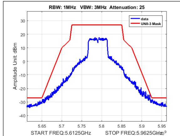
Plot 439. Undesirable Emissions, UNII-3 Emissions Mask, 40M, 5785MHz, 2Panel
