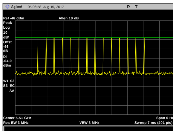
Plot 19. Radar Waveform Calibration, Type 4 Calibration 5510 MHz
