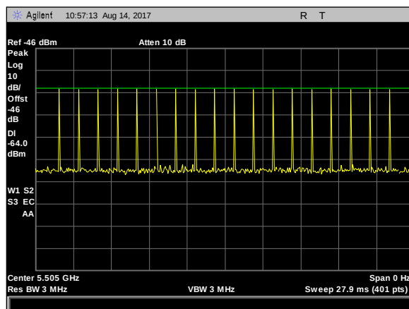
Plot 2. Radar Waveform Calibration, Type 0 Calibration 5505 MHz
