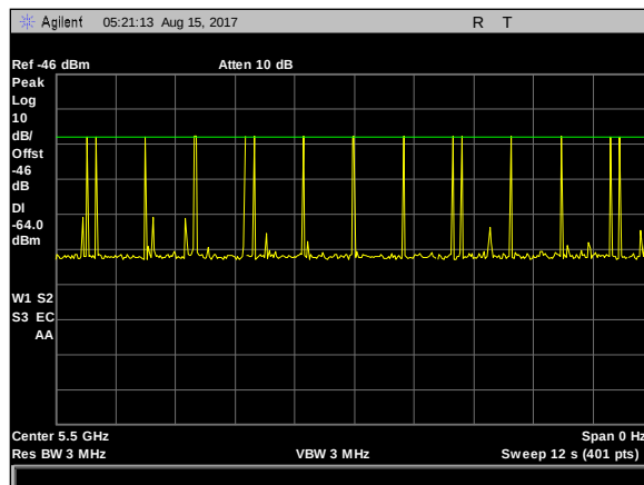
Plot 21. Radar Waveform Calibration, Type 5 Calibration 5500 MHz
