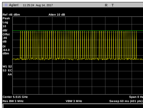
Plot 8. Radar Waveform Calibration, Type 1 Calibration 5515 MHz
