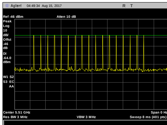
Plot 15. Radar Waveform Calibration, Type 3 Calibration 5510 MHz
