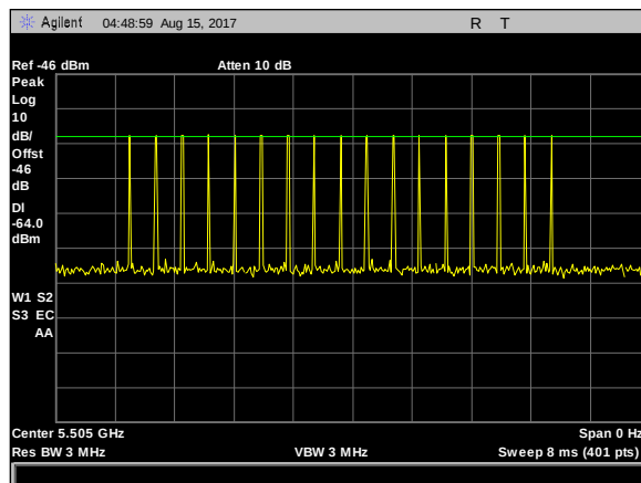
Plot 14. Radar Waveform Calibration, Type 3 Calibration 5505 MHz
