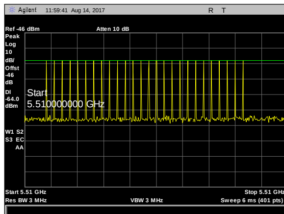
Plot 11. Radar Waveform Calibration, Type 2 Calibration 5510 MHz
