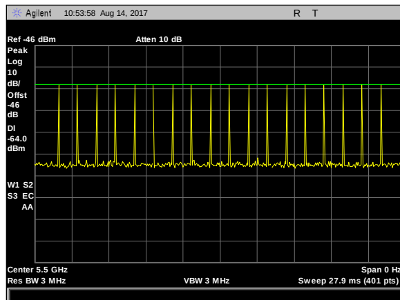
Plot 1. Radar Waveform Calibration, Type 0 Calibration 5500 MHz
