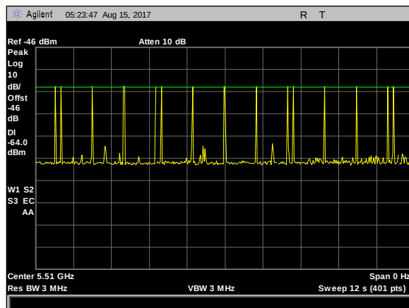
Plot 23. Radar Waveform Calibration, Type 5 Calibration 5510 MHz
