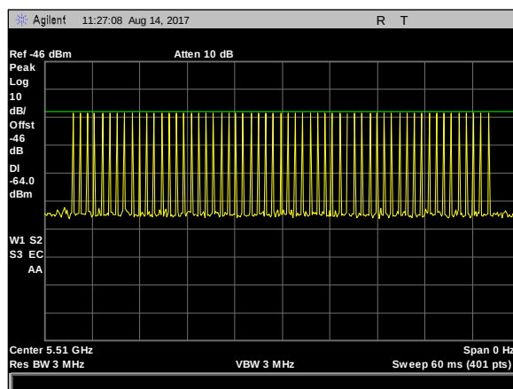
Plot 7. Radar Waveform Calibration, Type 1 Calibration 5510 MHz
