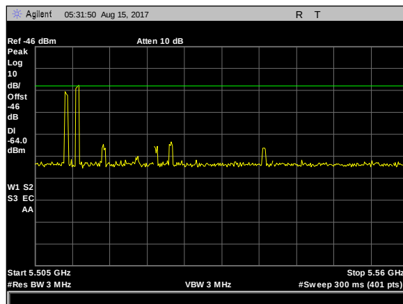
Plot 26. Radar Waveform Calibration, Type 6 Calibration 5505 MHz
