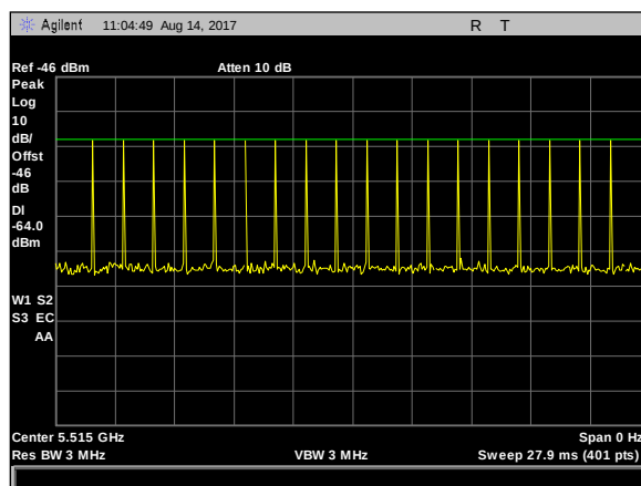
Plot 4. Radar Waveform Calibration, Type 0 Calibration 5515 MHz
