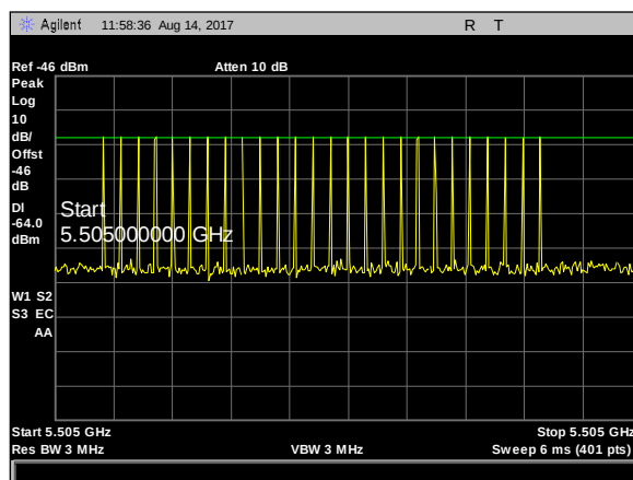
Plot 10. Radar Waveform Calibration, Type 2 Calibration 5505 MHz
