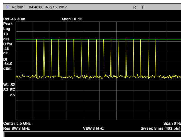
Plot 13. Radar Waveform Calibration, Type 3 Calibration 5500 MHz
