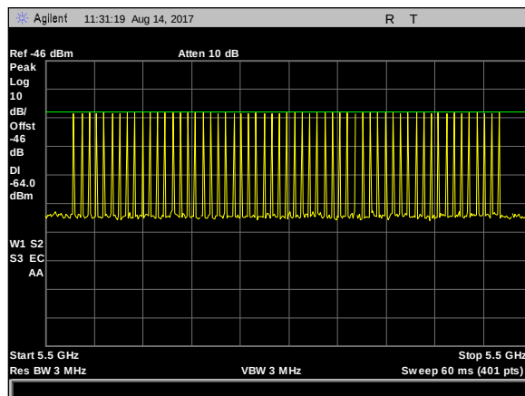
Plot 5. Radar Waveform Calibration, Type 1 Calibration 5500 MHz
