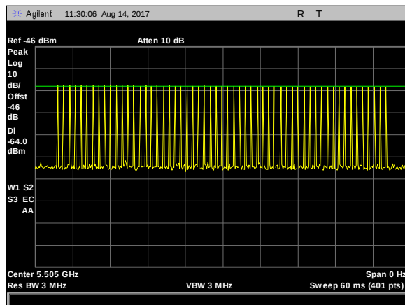
Plot 6. Radar Waveform Calibration, Type 1 Calibration 5505 MHz
