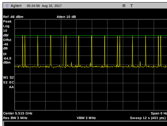
Plot 24. Radar Waveform Calibration, Type 5 Calibration 5515 MHz
