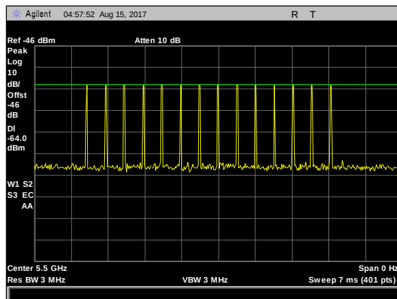
Plot 17. Radar Waveform Calibration, Type 4 Calibration 5500 MHz
