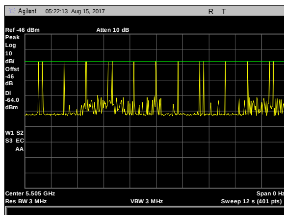
Plot 22. Radar Waveform Calibration, Type 5 Calibration 5505 MHz
