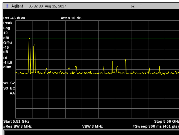
Plot 27. Radar Waveform Calibration, Type 6 Calibration 5510 MHz
