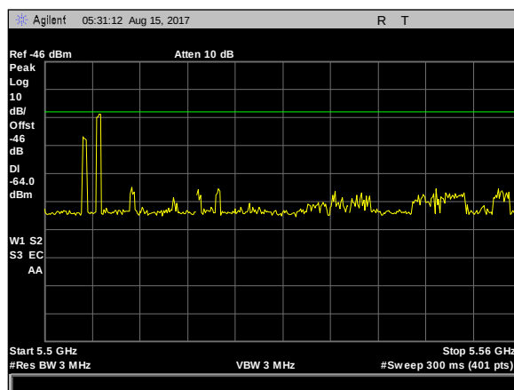
Plot 25. Radar Waveform Calibration, Type 6 Calibration 5500 MHz
