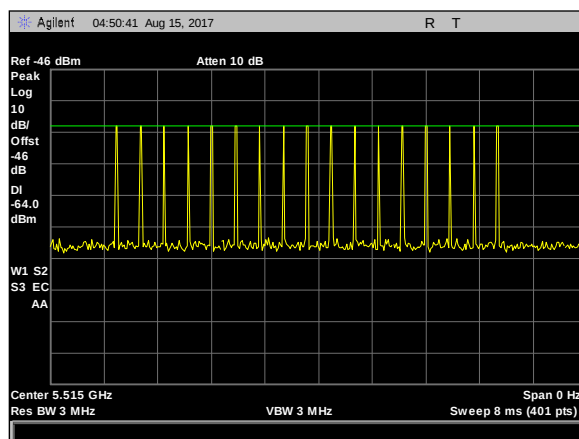
Plot 16. Radar Waveform Calibration, Type 3 Calibration 5515 MHz
