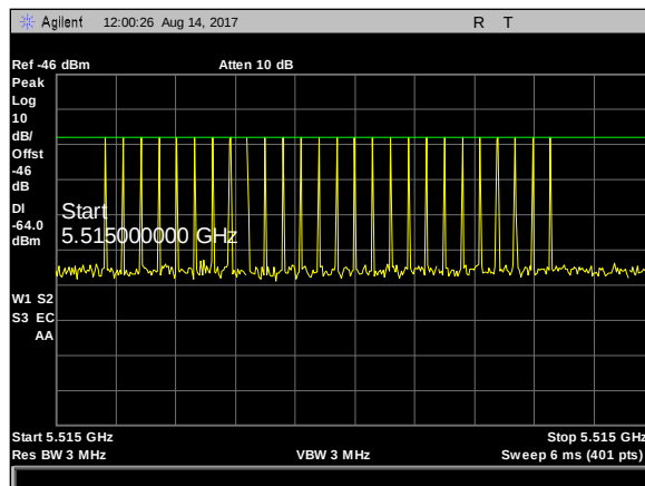
Plot 12. Radar Waveform Calibration, Type 2 Calibration 5515 MHz
