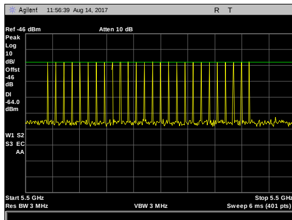
Plot 9. Radar Waveform Calibration, Type 2 Calibration 5500 MHz
