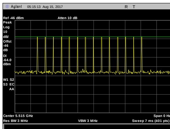
Plot 20. Radar Waveform Calibration, Type 4 Calibration 5515 MHz
