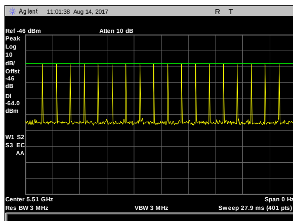
Plot 3. Radar Waveform Calibration, Type 0 Calibration 5510 MHz
