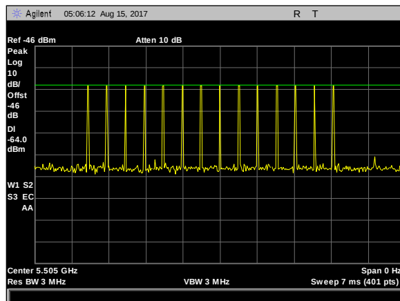
Plot 18. Radar Waveform Calibration, Type 4 Calibration 5505 MHz
