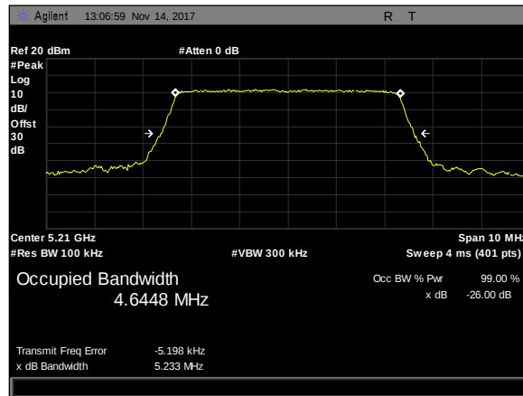
Plot 38. 26 dB Occupied Bandwidth, 5M, 5210, 90Sector, rf2
