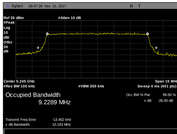
Plot 66. 26 dB Occupied Bandwidth, 10M, 5245, 50Omni, rf2
