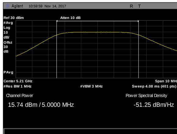
Plot 149. Maximum Conducted Output Power, 5M, 5210, 50Omni, rf1
