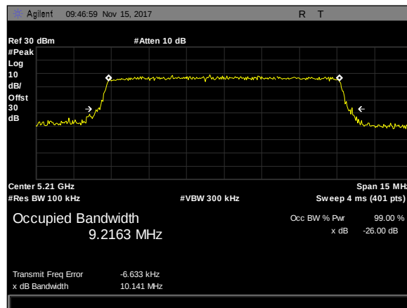
Plot 65. 26 dB Occupied Bandwidth, 10M, 5210, 50Omni, rf2
