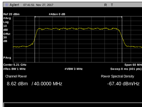
Plot 95. Maximum Conducted Output Power, 40M, 5210, 1Panel, rf2
