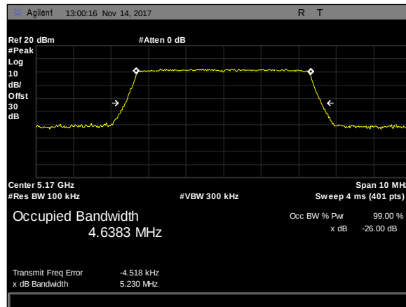
Plot 37. 26 dB Occupied Bandwidth, 5M, 5170, 90Sector, rf2
