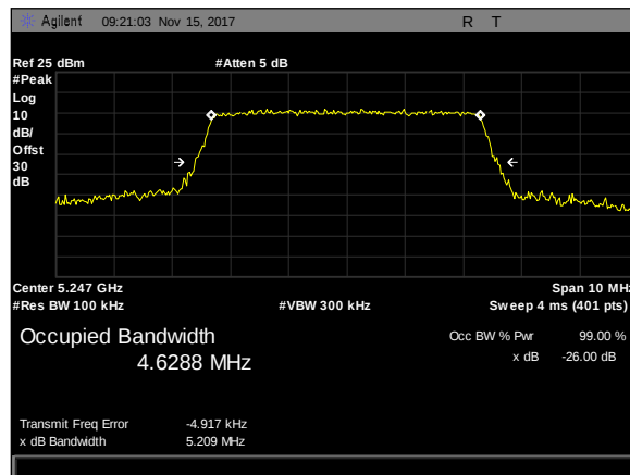
Plot 51. 26 dB Occupied Bandwidth, 5M, 5247.5, Omni8, rf2
