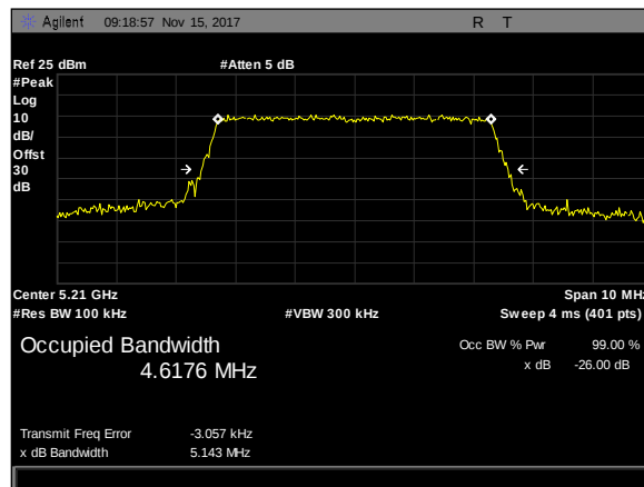
Plot 50. 26 dB Occupied Bandwidth, 5M, 5210, Omni8, rf2
