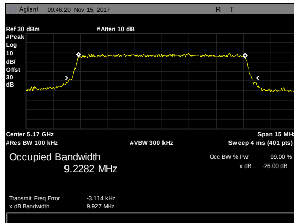
Plot 64. 26 dB Occupied Bandwidth, 10M, 5170, 50Omni, rf2
