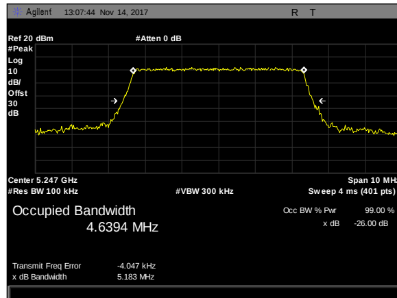
Plot 39. 26 dB Occupied Bandwidth, 5M, 5247.5, 90Sector, rf2
