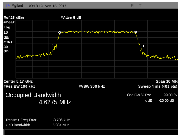
Plot 49. 26 dB Occupied Bandwidth, 5M, 5170, Omni8, rf2
