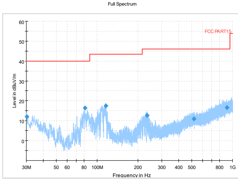
Frequency Range: 30MHz-1GHz Detector: QP mode Modulation type: Coded 500K
