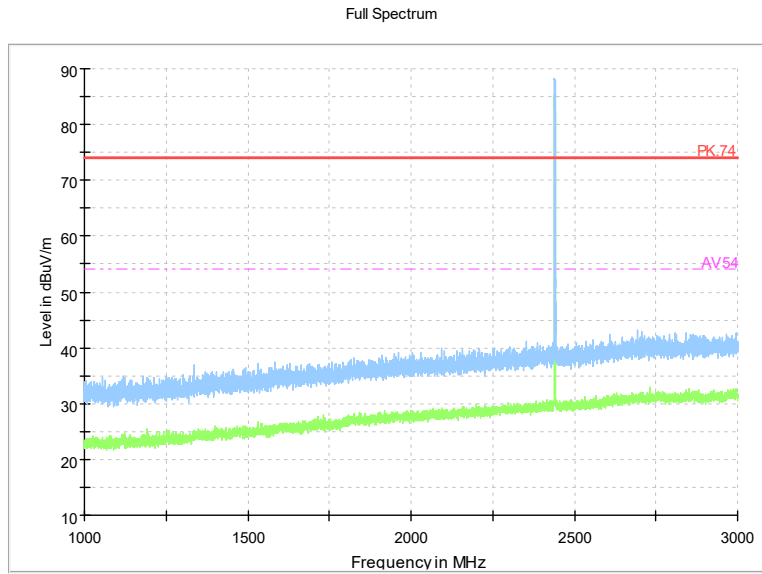
Frequency Range: 1GHz-3GHz Detector: Av mode and PK mode Modulation type: Coded 500K
