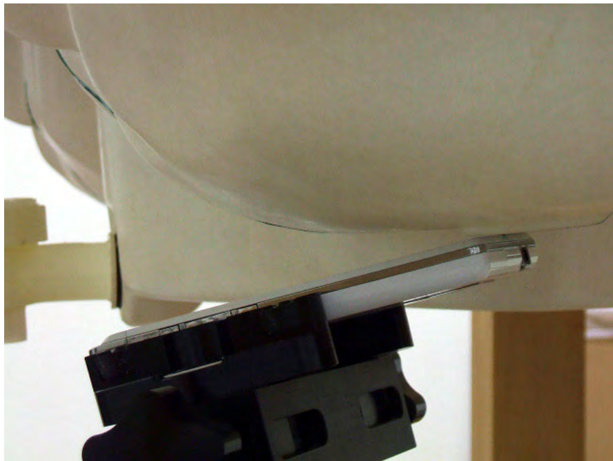
– Ear/Tilt Position –
