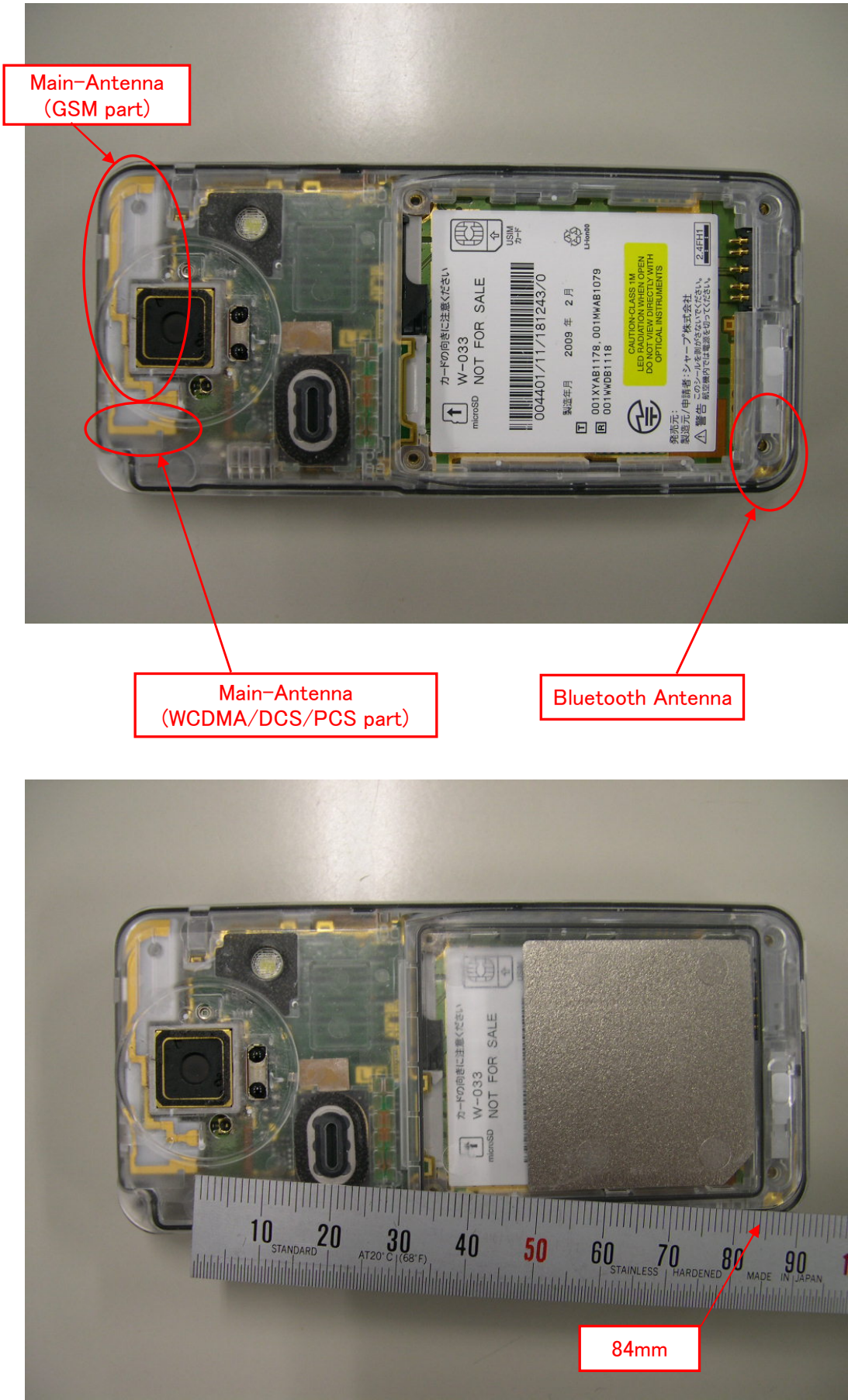
Distance between PCS antenna and Bluetooth antenna
