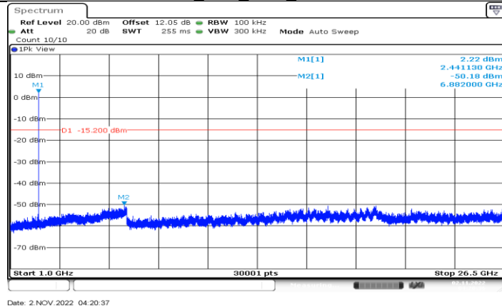
3DH5_Ant1_2441_1000~26500
