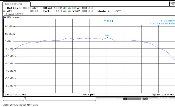
3DH5_Ant1_2402_0~Reference
