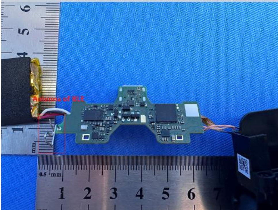
Antenna Location:
