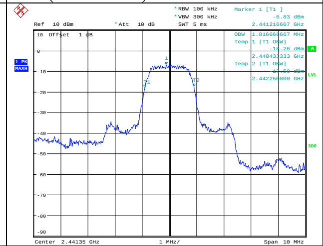
MCH (99% bandwidth)
