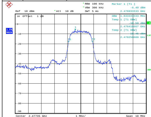
HCH (99% bandwidth)
