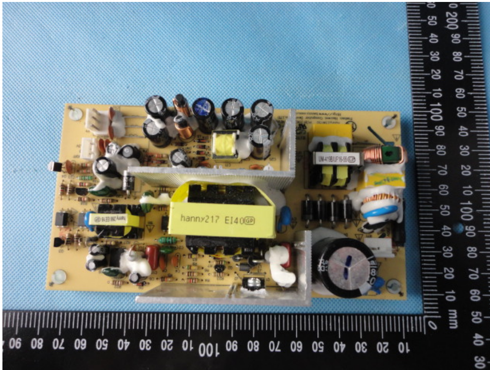
Power supply board of subwoofer (Hanwei, type: Hanny23w150)
