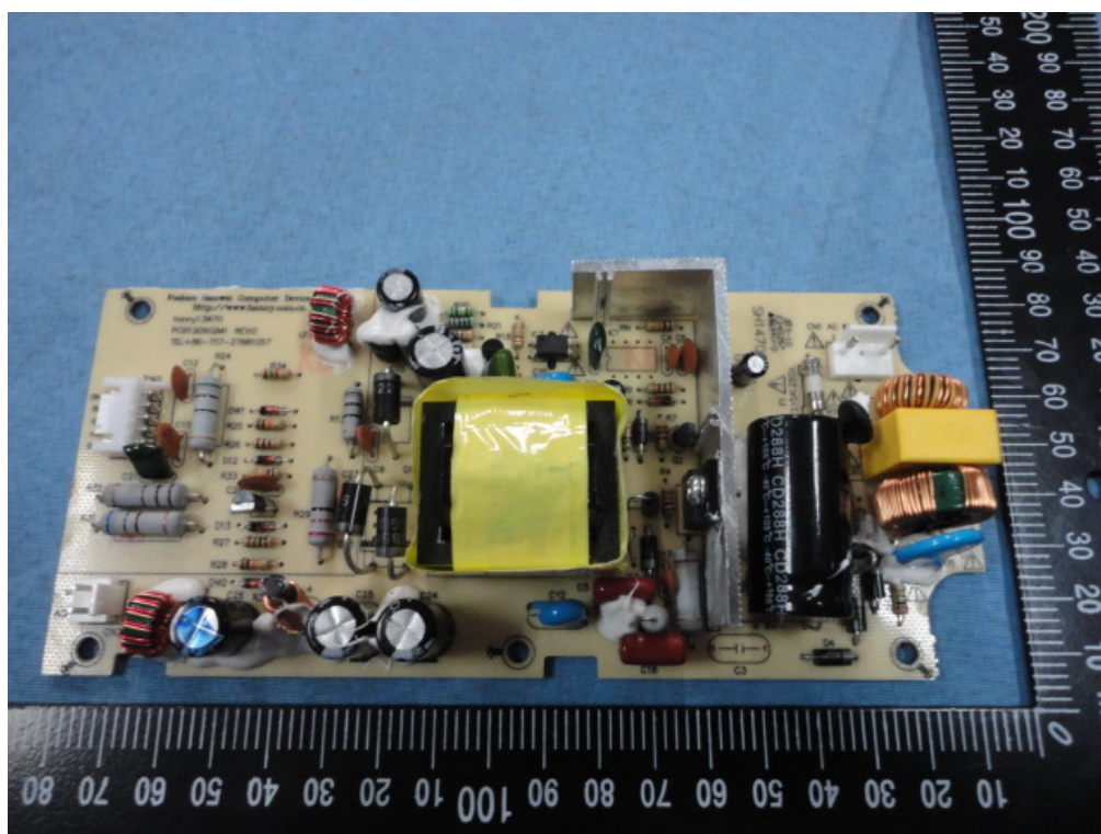
Power supply board of soundbar (Hanwei, type: Hanny13w70)
