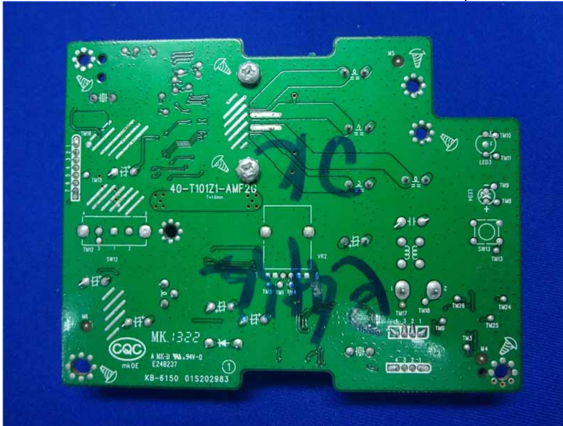
Figure 11 Components Side of the PCB
