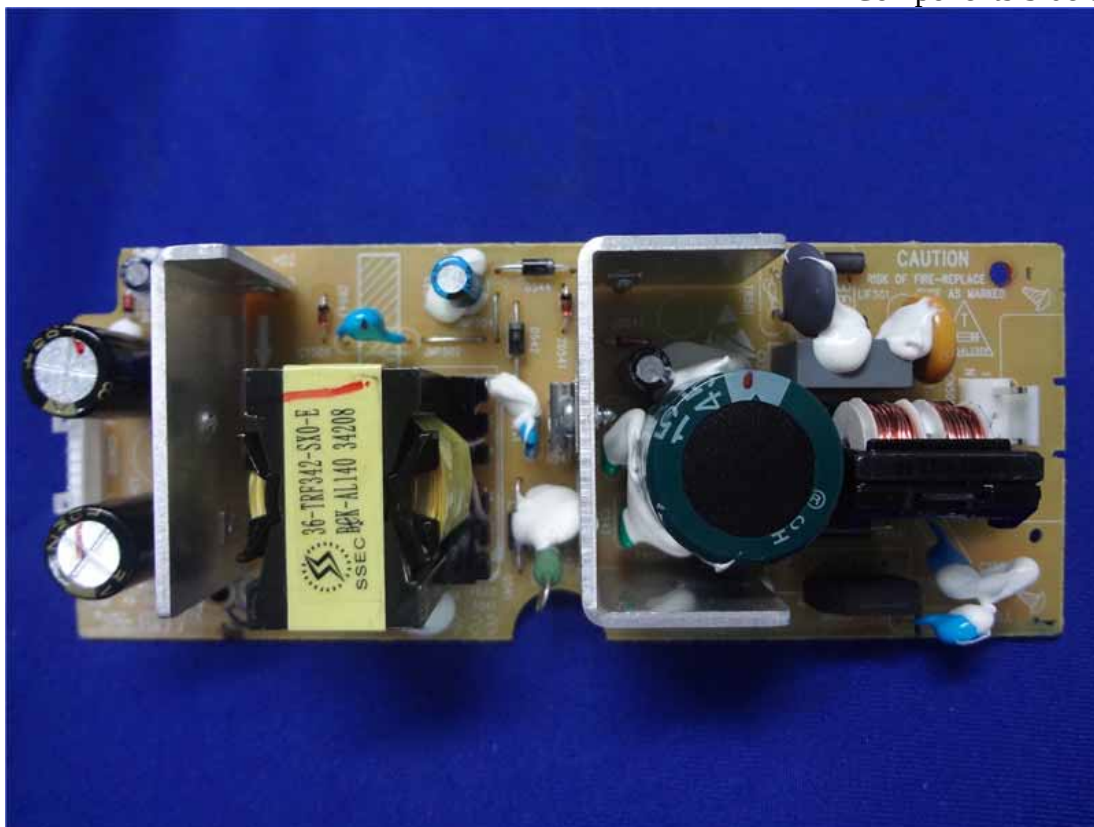
Figure 16 Components Side of the PCB
