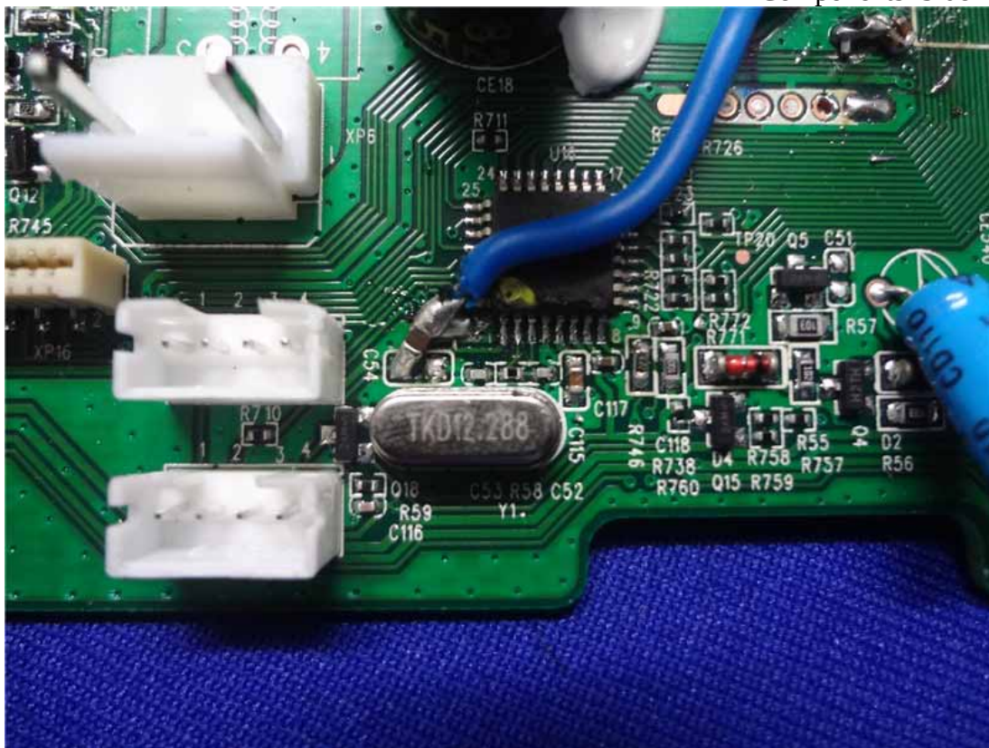
Figure 12 Components Side of the PCB
