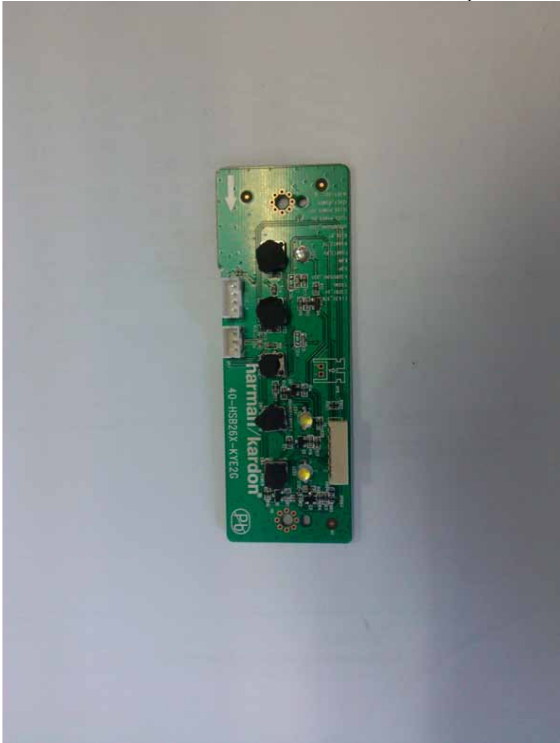
Figure 20 Components Side of the PCB
