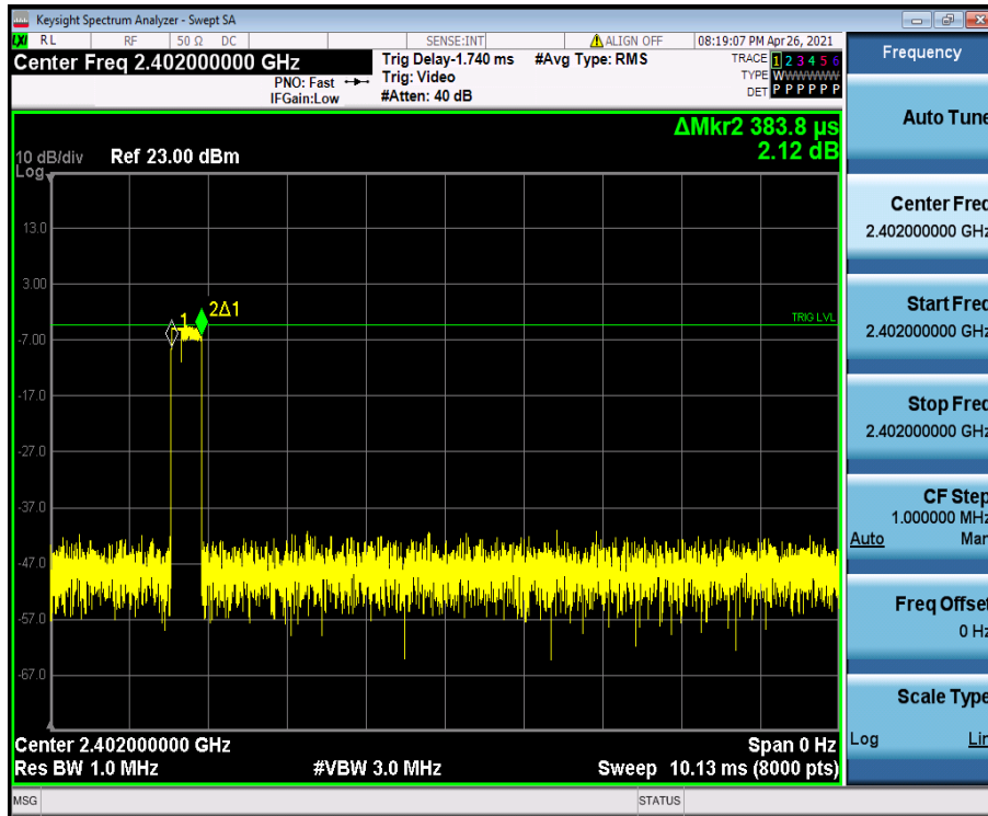
2DH1_Ant1_Hop_2402
