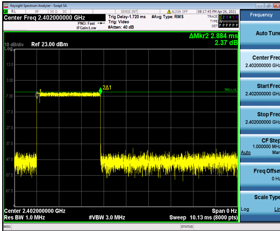
2DH5_Ant1_Hop_2402
