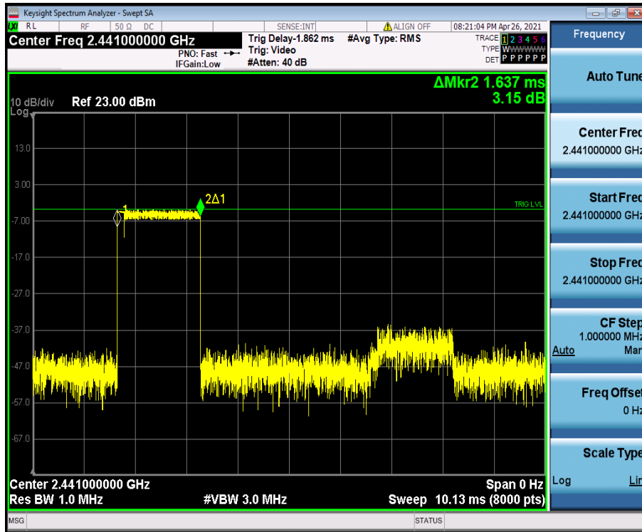
2DH3_Ant1_Hop_2441
