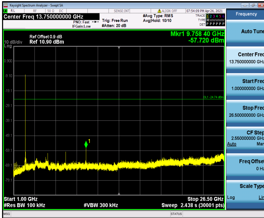
2DH5_Ant1_2480_0~Reference
