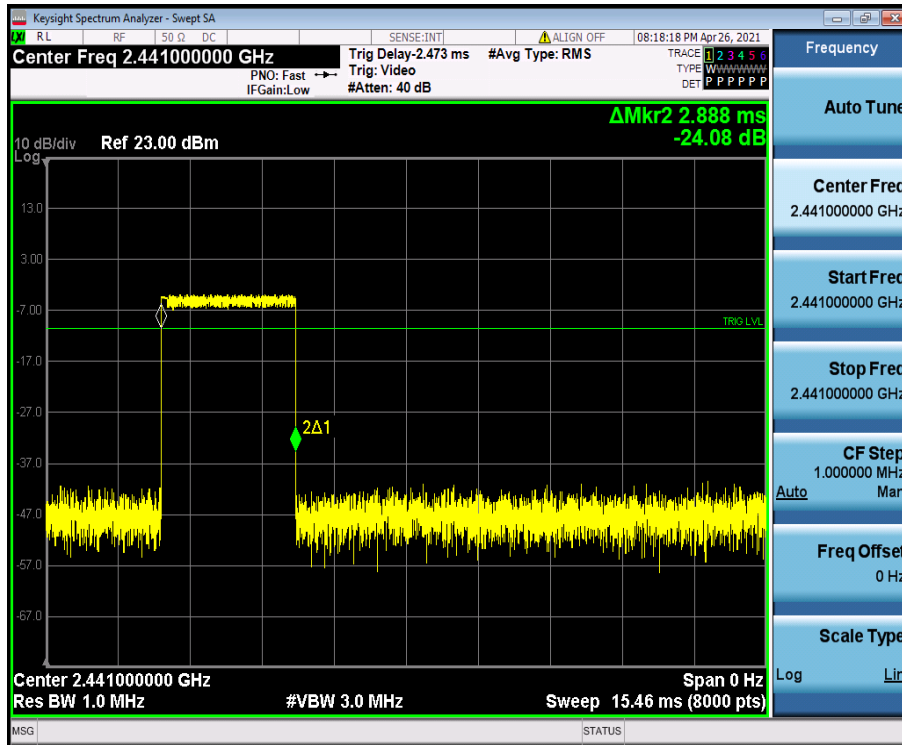
2DH5_Ant1_Hop_2441
