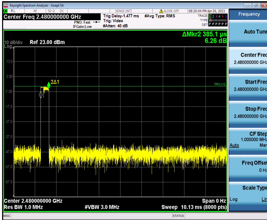
2DH1_Ant1_Hop_2480
