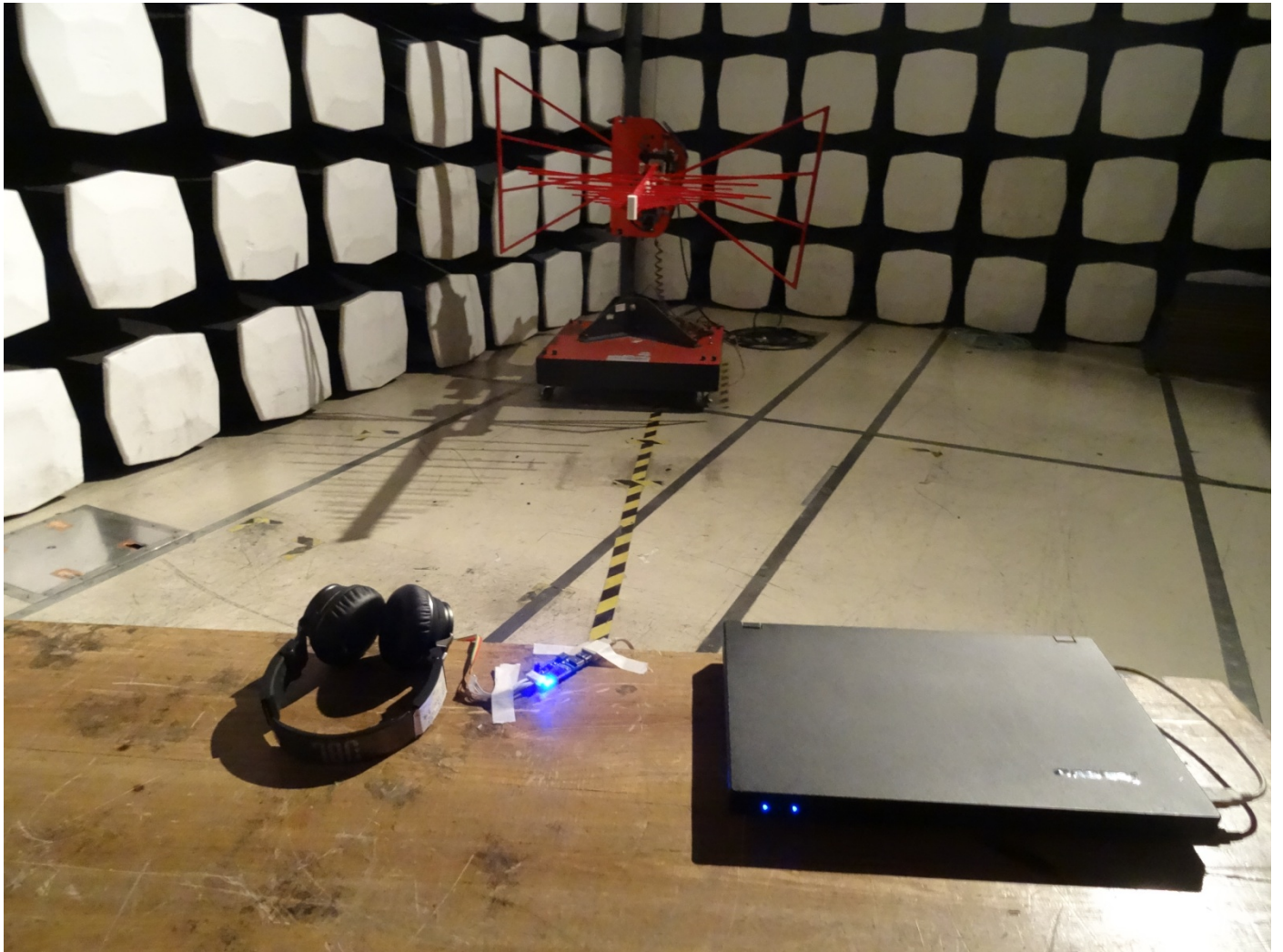
Test Setup photos
