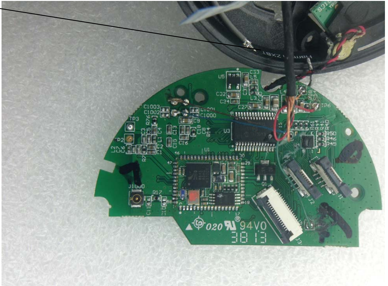
Antenna Location
