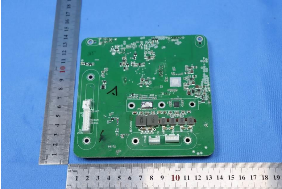
Antenna location: 2.4G property antenna
