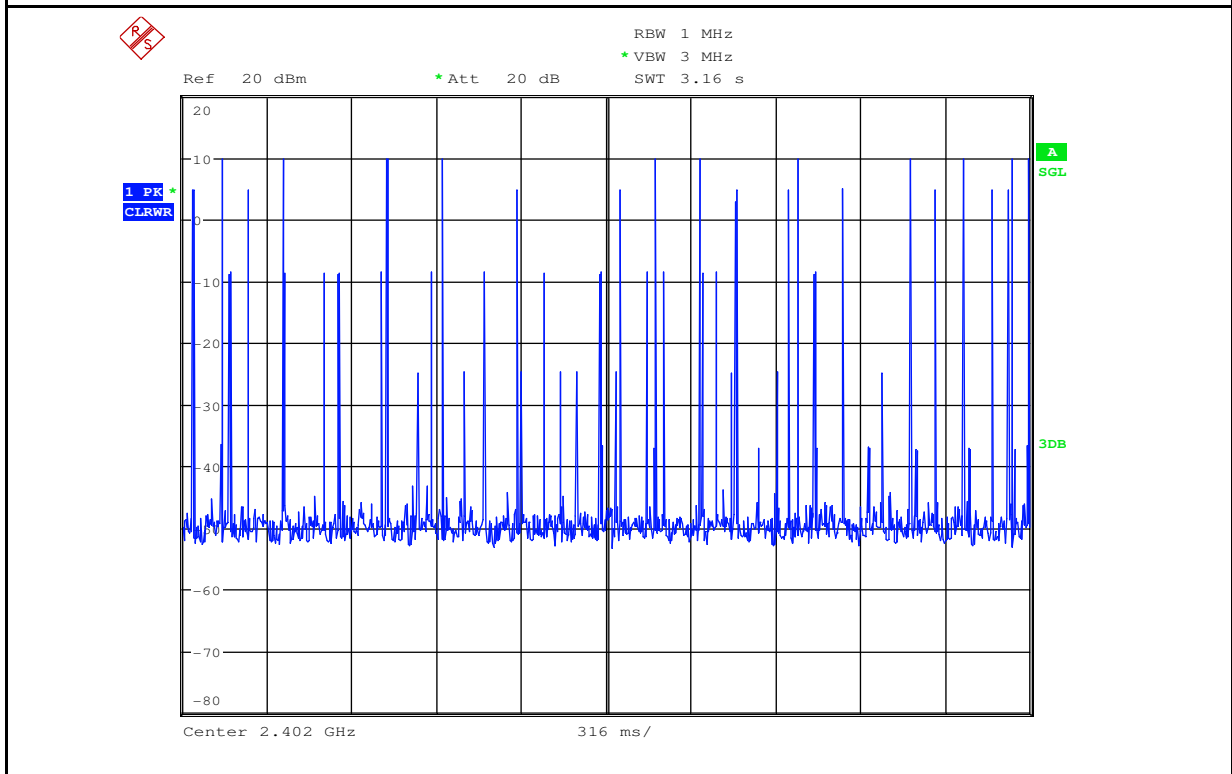
Dwell Time_2DH5_2402
