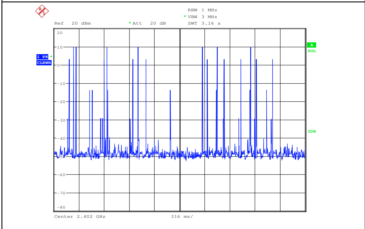
Dwell Time_2DH1_2402
