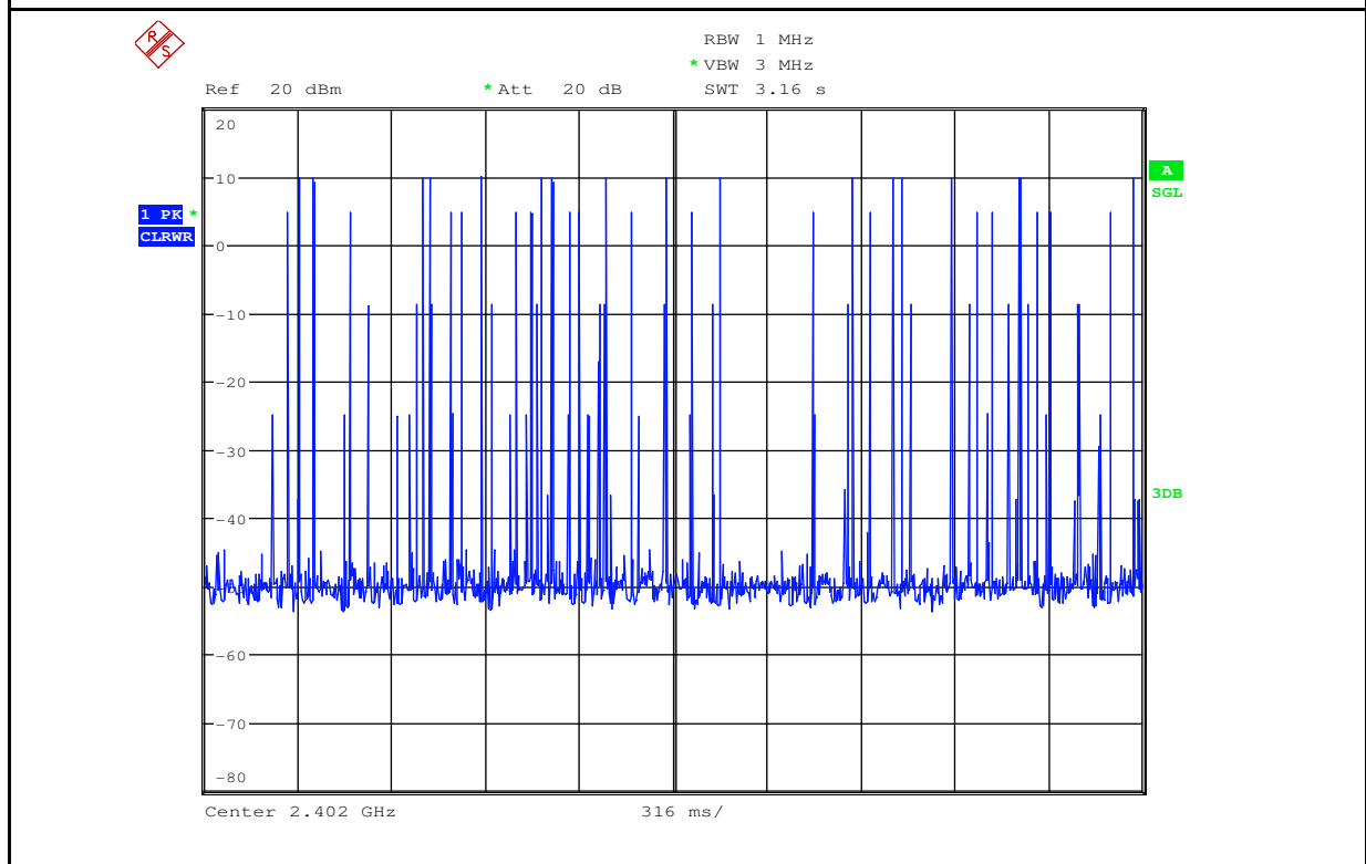
Dwell Time_2DH3_2402
