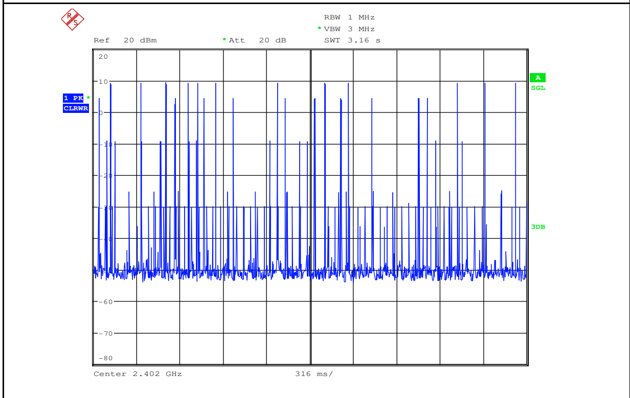
Dwell Time_3DH5_2402
