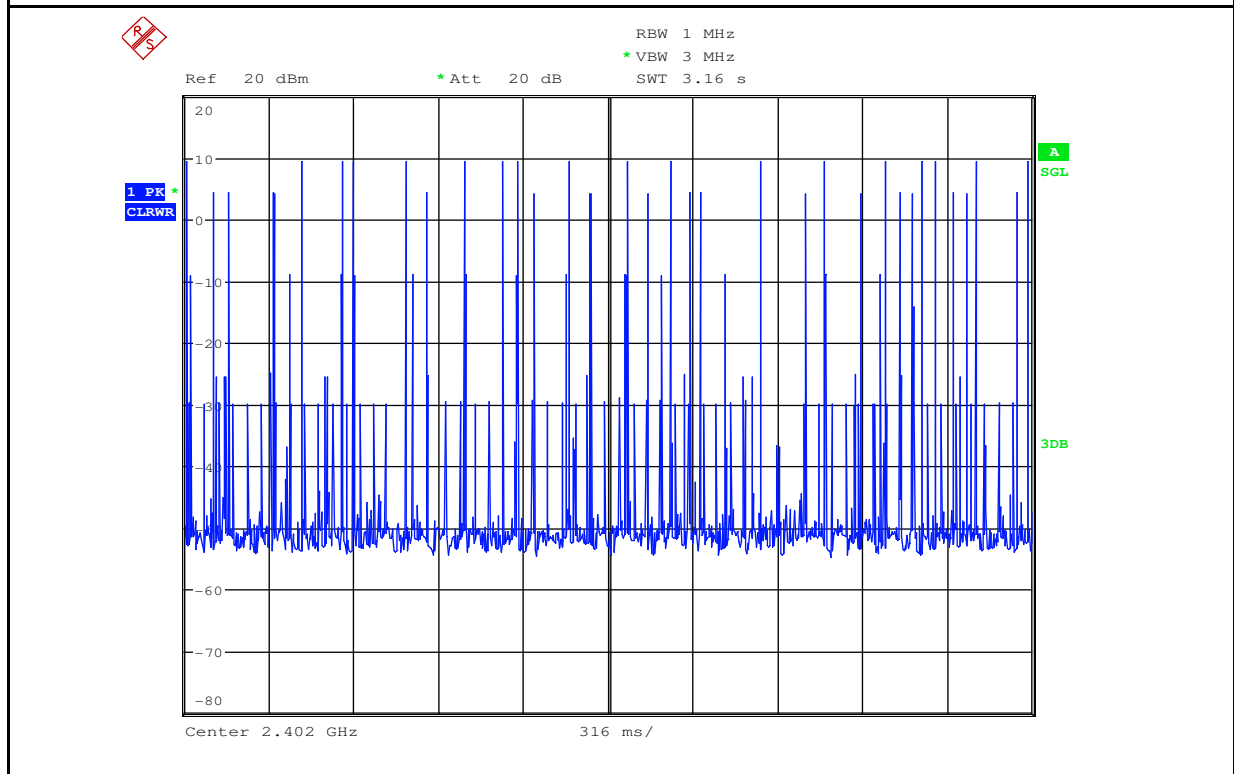
Dwell Time_2DH3_2402
