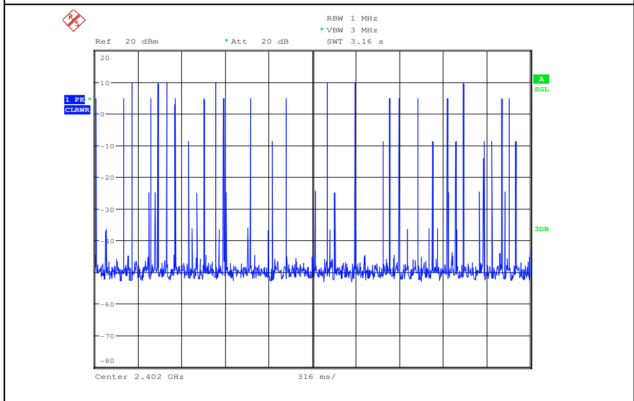
Dwell Time_3DH5_2402
