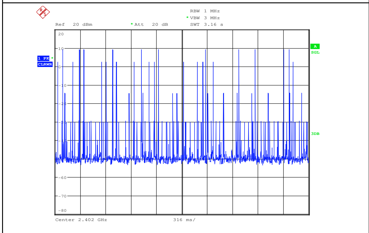
Dwell Time_DH5_2402
