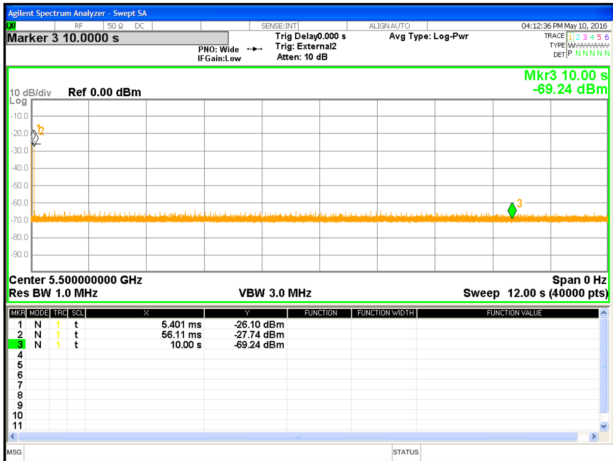
Figure 5: Channel Move Time and Channel Closing Transmission Time at 5500 MHz
