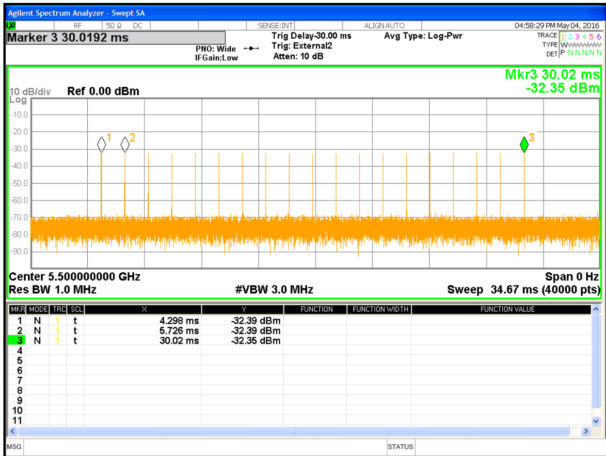
Figure 2: 5500 MHz Radar Pulse Type 0 at Master (Cisco AP)
