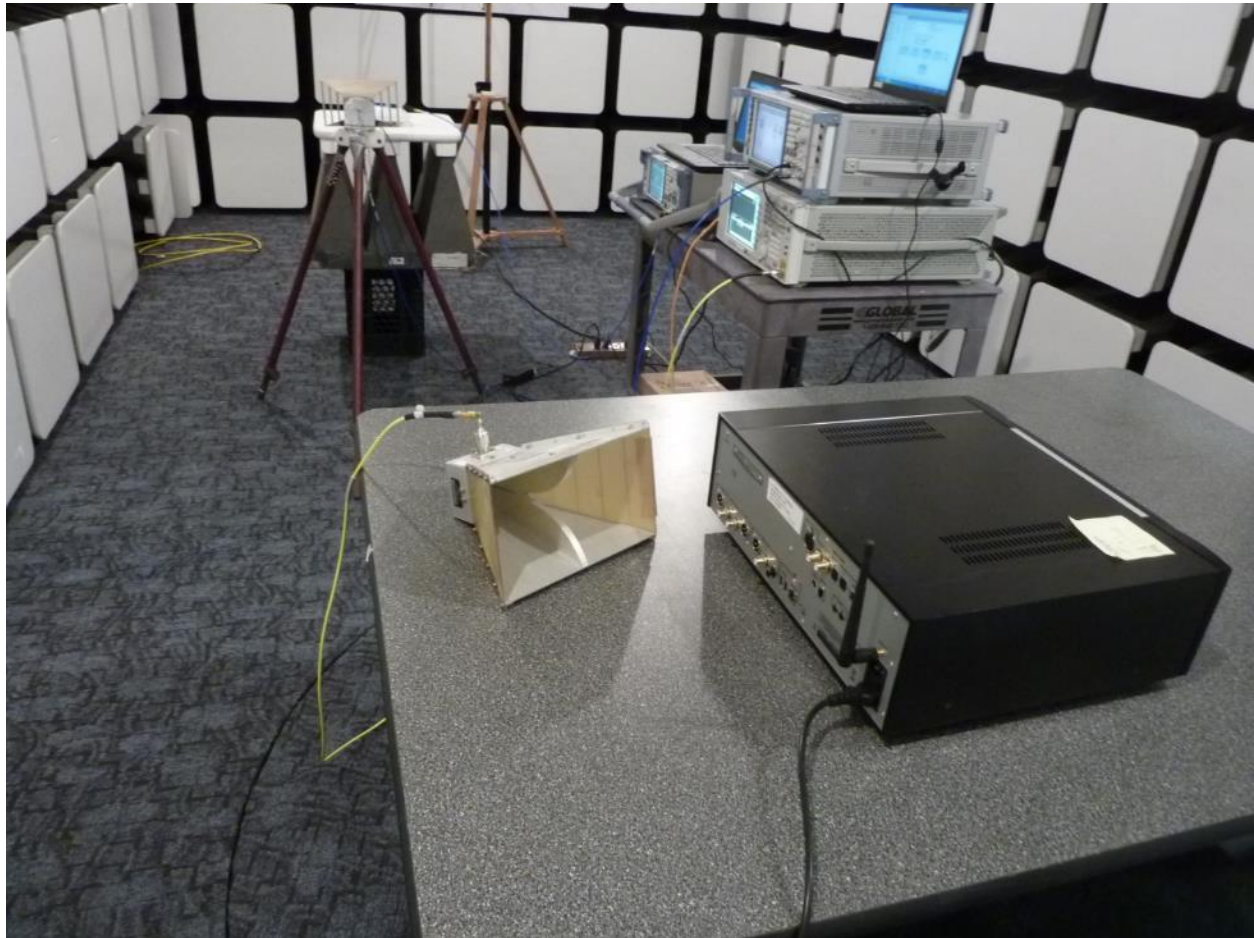
Figure 11: DFS Test Setup (View 1)
