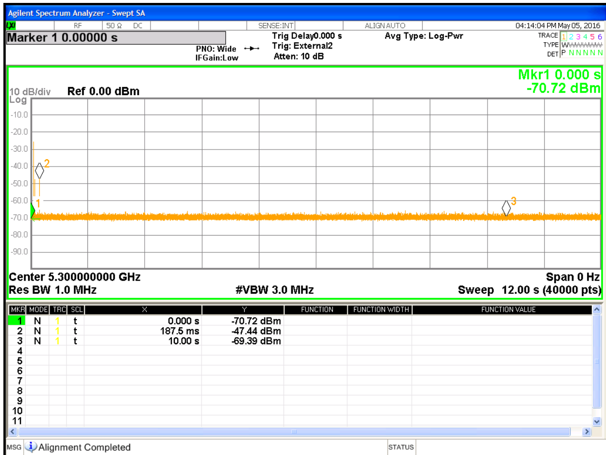
Figure 3: Channel Move Time and Channel Closing Transmission Time at 5300 MHz
