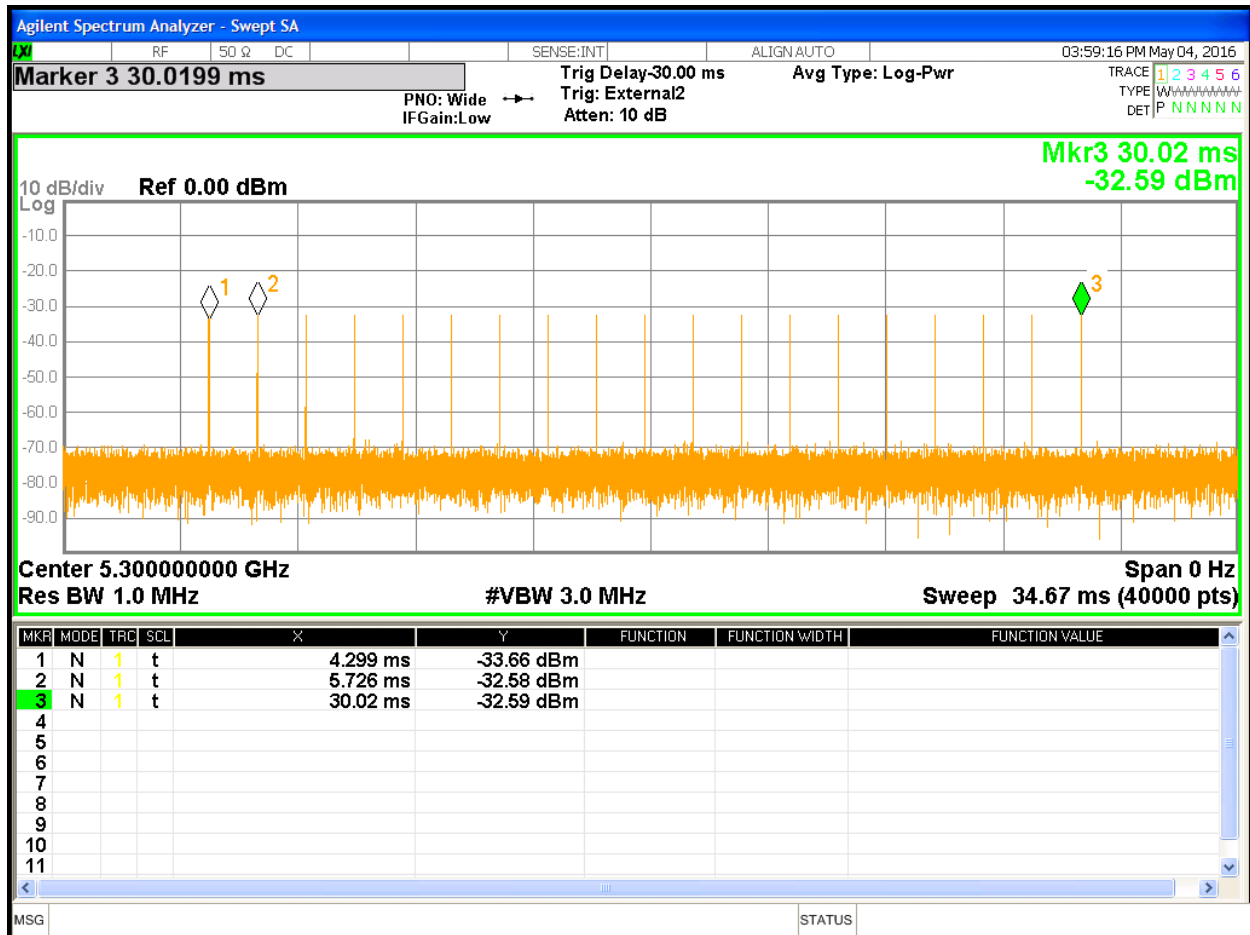
Figure 1: 5300 MHz Radar Pulse Type 0 at Master (Cisco AP)
