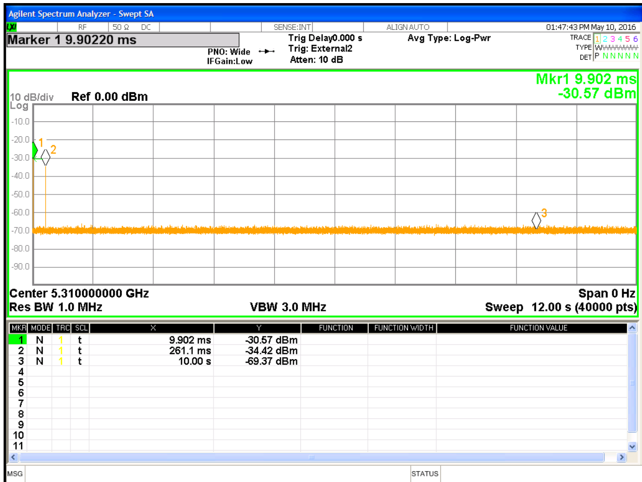
Figure 4: Channel Move Time and Channel Closing Transmission Time at 5310 MHz
