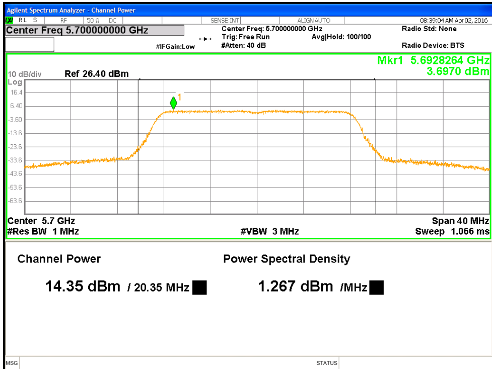
Figure 1: Maximum Transmitted Power, 5700 MHz at 802.11a 6Mbps
