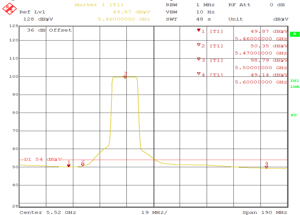
Figure 31: Radiated Emission 5470 MHz Edge for HT20 5500 MHz – Vert. (Pk)
