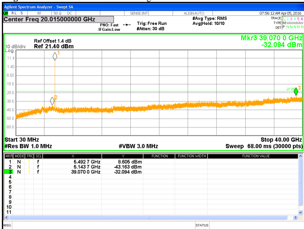
Figure 16: Undesirable Emission for HT20-MCS0 at 5500 MHz
