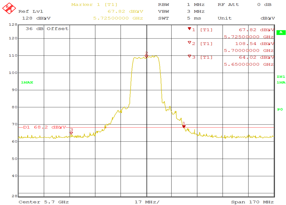
Figure 35: Radiated Emission 5725 MHz Edge for HT20 5700 MHz – Vert. (Pk)
