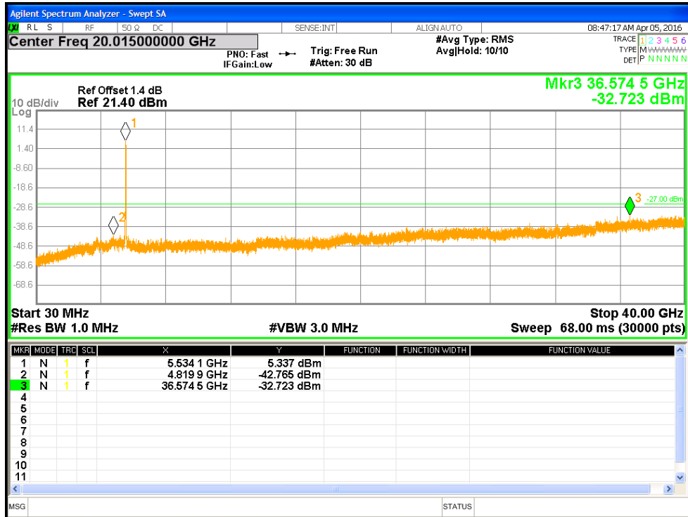
Figure 22: Undesirable Emission for HT40-MCS0 at 5550 MHz
