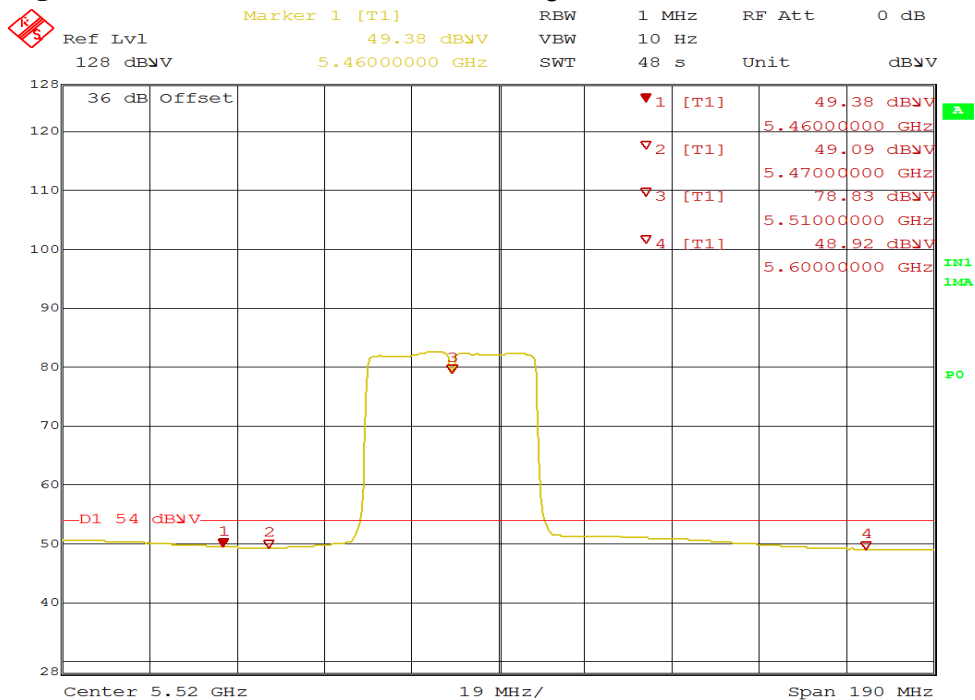
Figure 39: Radiated Emission 5470 MHz Edge for HT40 5510 MHz – Horz. (Pk)
