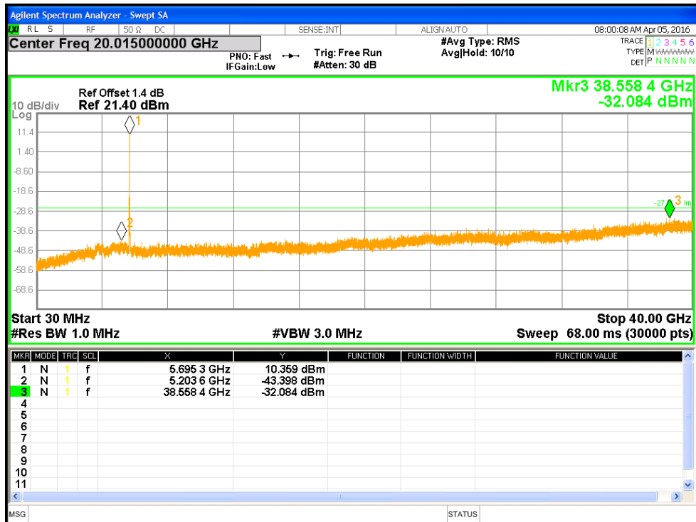
Figure 19: Undesirable Emission for HT20-MCS0 at 5700 MHz
