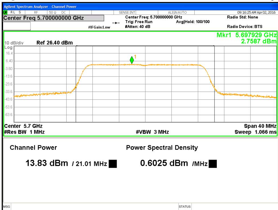
Figure 2: Maximum Transmitted Power, 5700 MHz at HT20 MCS0
