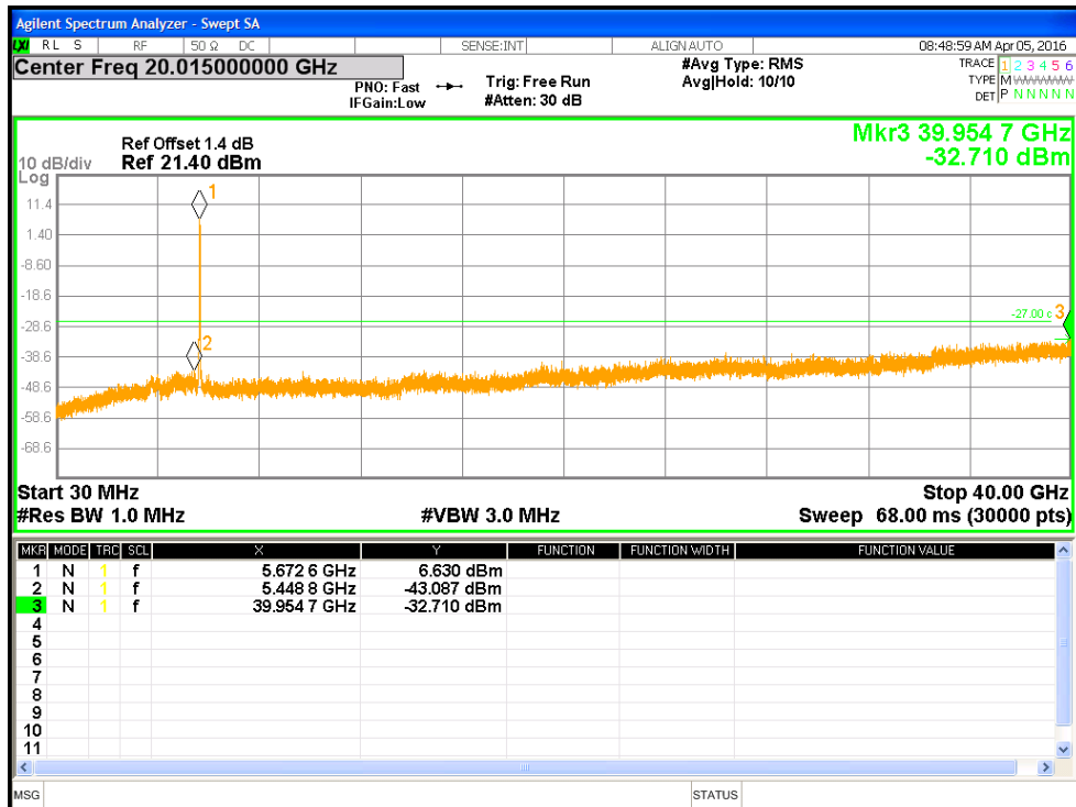
Figure 24: Undesirable Emission for HT40-MCS0 at 5670 MHz
