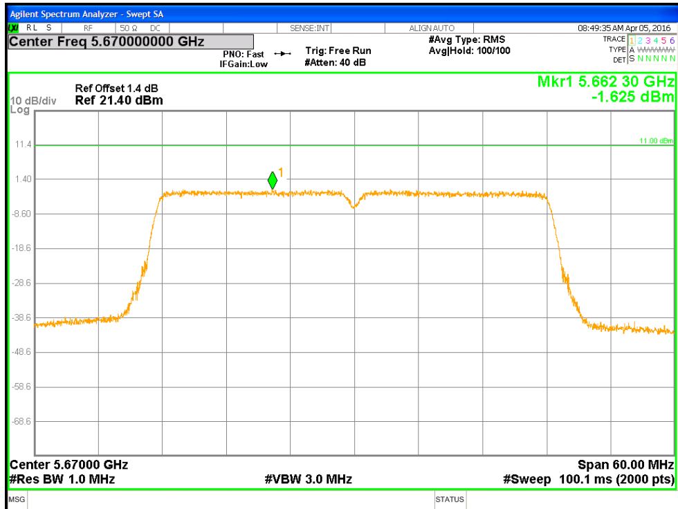
Figure 9: Power Spectral Density (FCC & RSS), 5670 MHz at HT40 MCS0
