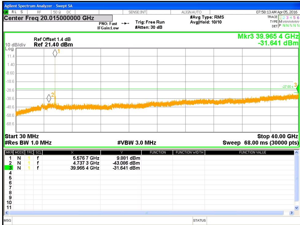
Figure 17: Undesirable Emission for HT20-MCS0 at 5580 MHz
