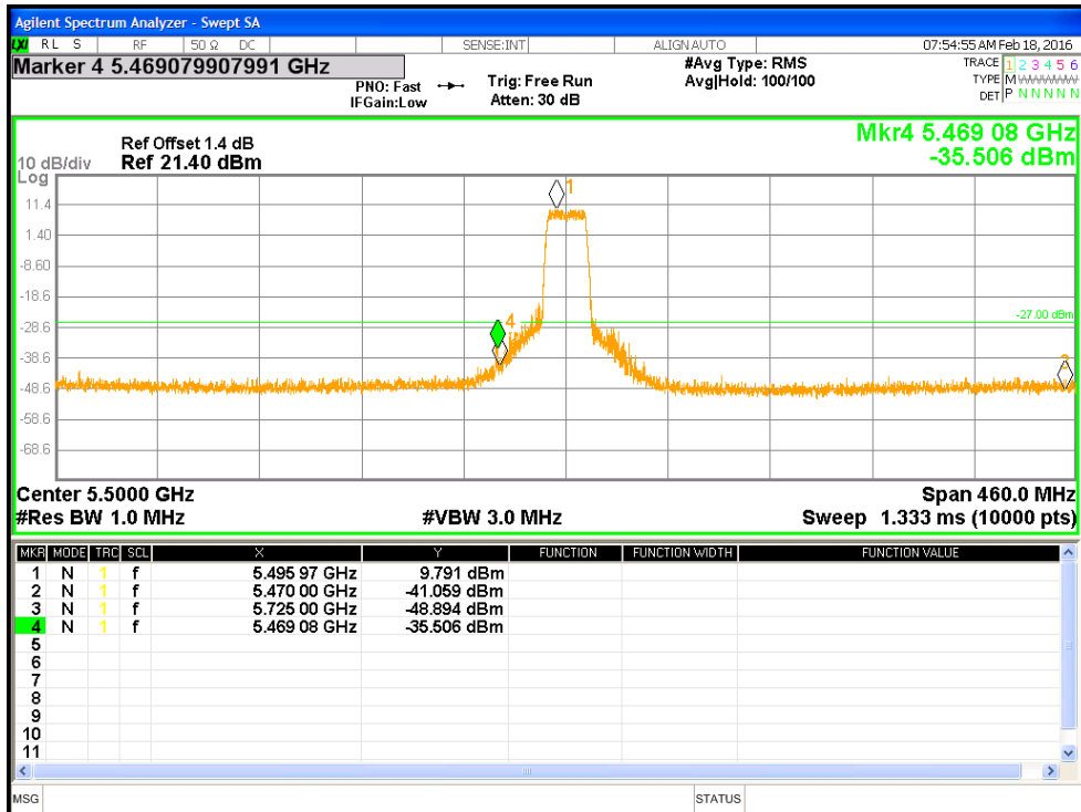
Figure 15: Measured Bandedge for HT20-MCS0 at 5500 MHz
