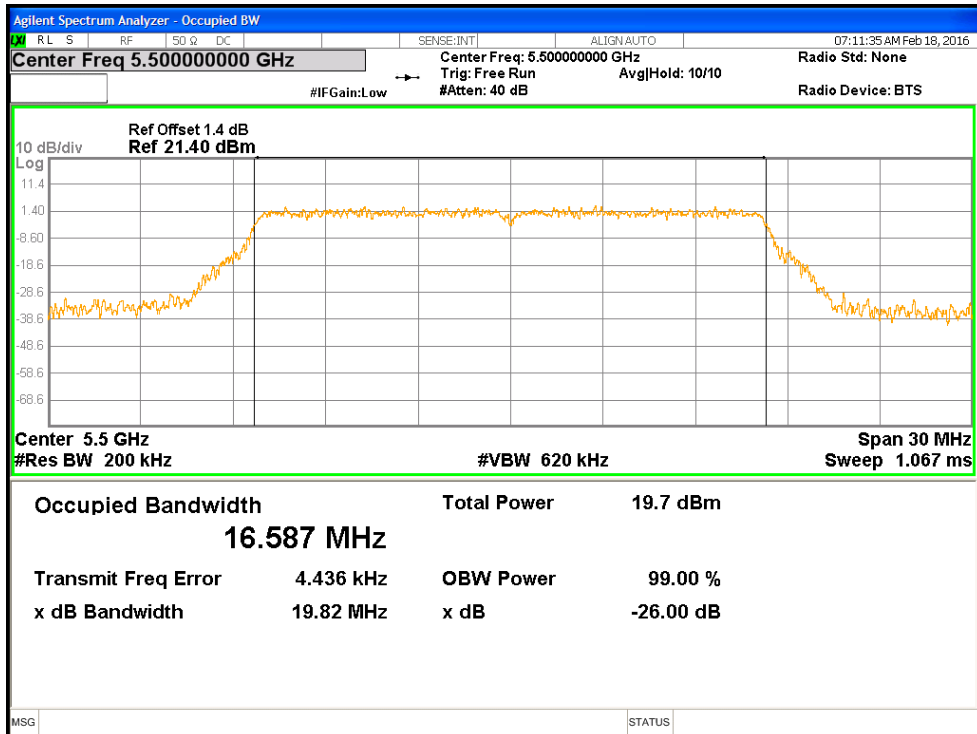
Figure 4: 26dB & 99% Occupied Bandwidth, 5500 MHz at 802.11a 6Mbps
