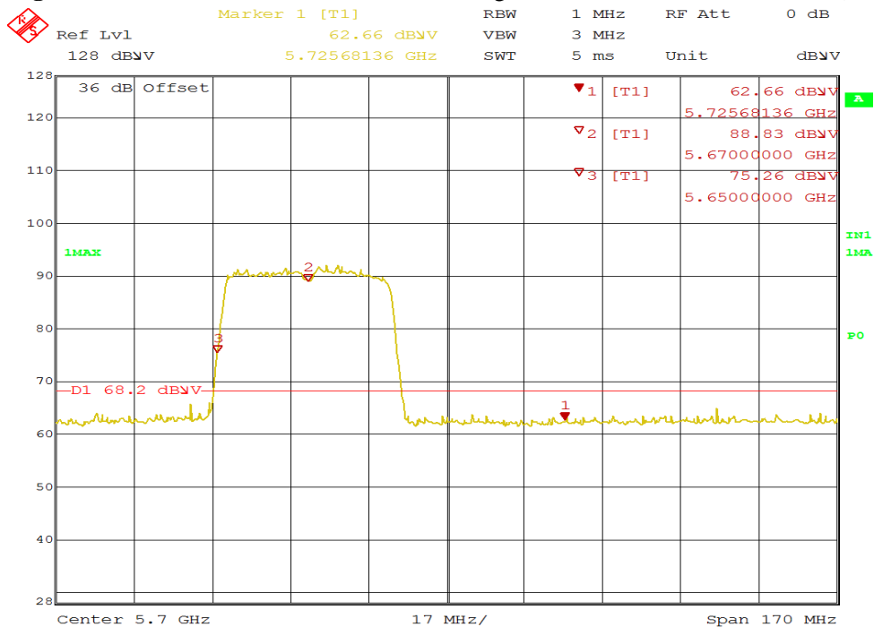
Figure 41: Radiated Emission 5725 MHz Edge for HT40 5670 MHz – Vert. (Pk)
