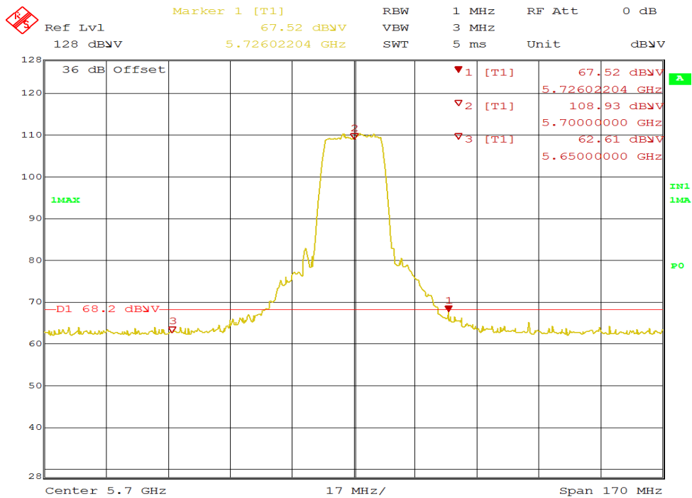
Figure 29: Radiated Emission 5725 MHz Edge for 11a 5700 MHz – Vert. (Pk)
