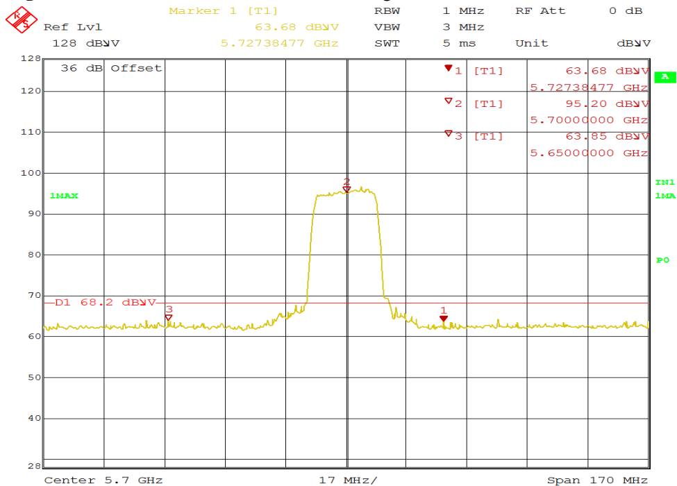
Figure 36: Radiated Emission 5725 MHz Edge for HT20 5700 MHz – Horz. (Pk)
