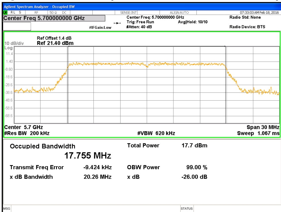
Figure 5: 26dB & 99% Occupied Bandwidth, 5700 MHz at HT20 MCS0
