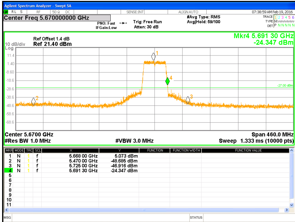
Figure 23: Measured Bandedge for HT40-MCS0 at 5670 MHz
