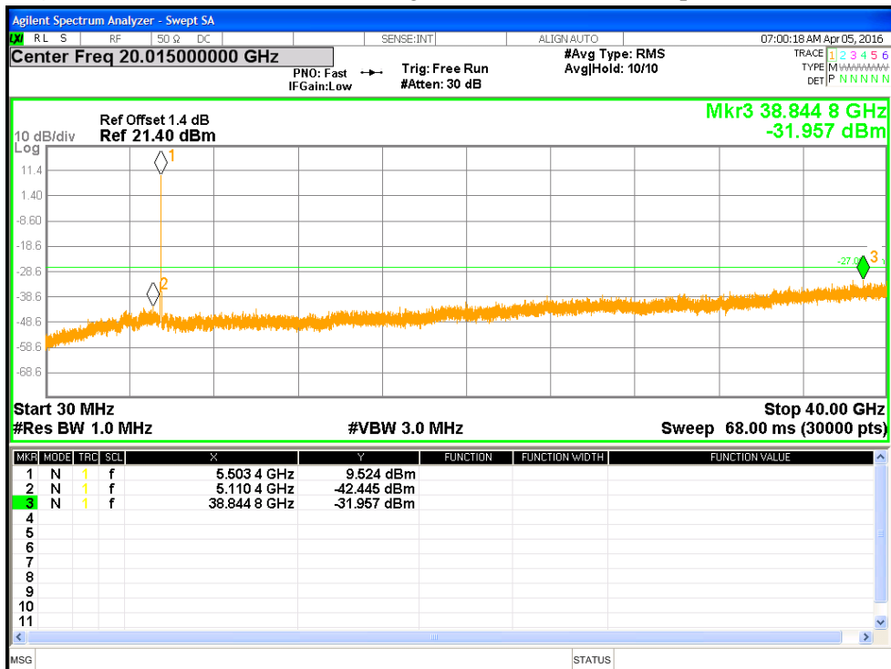
Figure 11: Undesirable Emission for 802.11a-6Mbps at 5500 MHz
