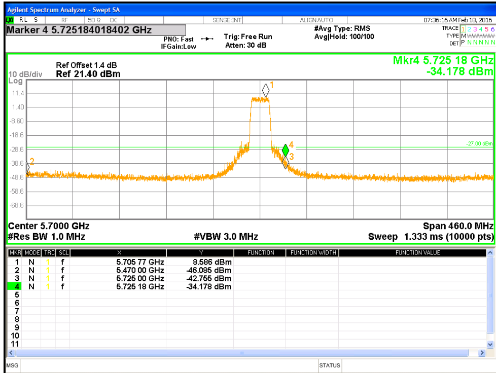
Figure 18: Measured Bandedge for HT20-MCS0 at 5700 MHz
