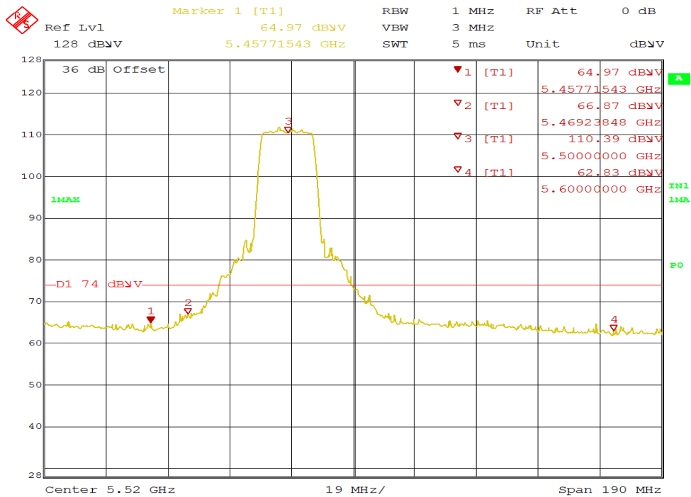
Figure 25: Radiated Emission 5470 MHz Edge for 11a 5500 MHz – Vert. (Pk)
