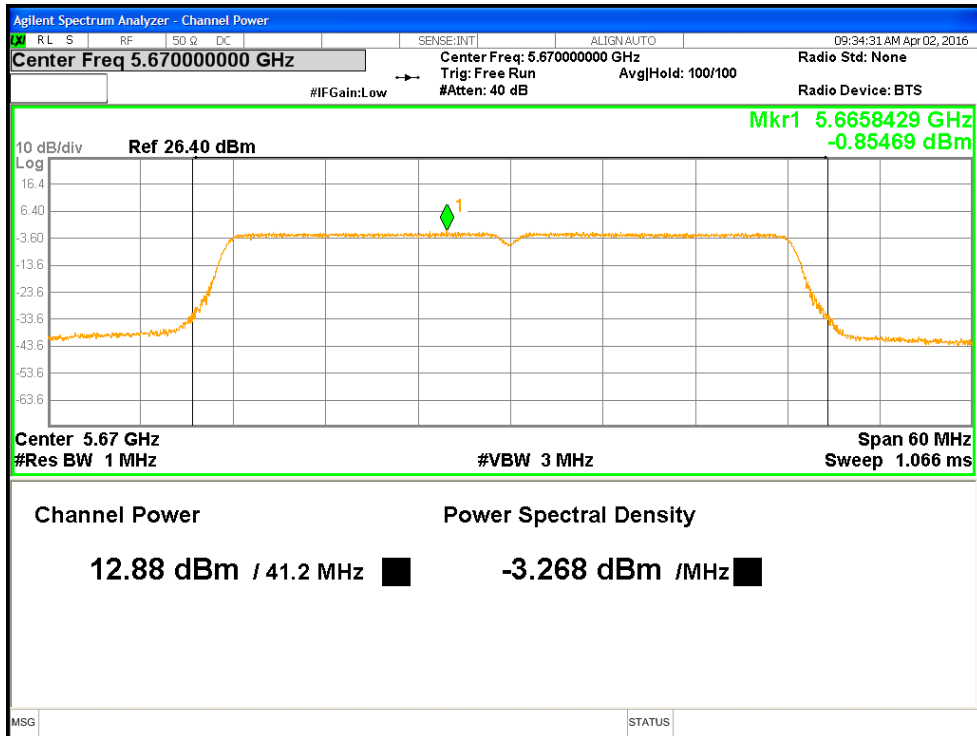
Figure 3: Maximum Transmitted Power, 5670 MHz at HT40 MCS0
