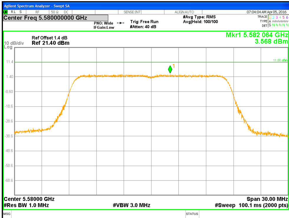
Figure 7: Power Spectral Density (FCC & RSS), 5580 MHz at 802.11a 6Mbps
