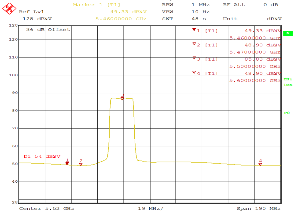
Figure 27: Radiated Emission 5470 MHz Edge for 11a 5500 MHz – Horz. (Pk)
