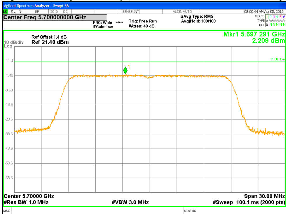
Figure 8: Power Spectral Density (FCC & RSS), 5700 MHz at HT20 MCS0
