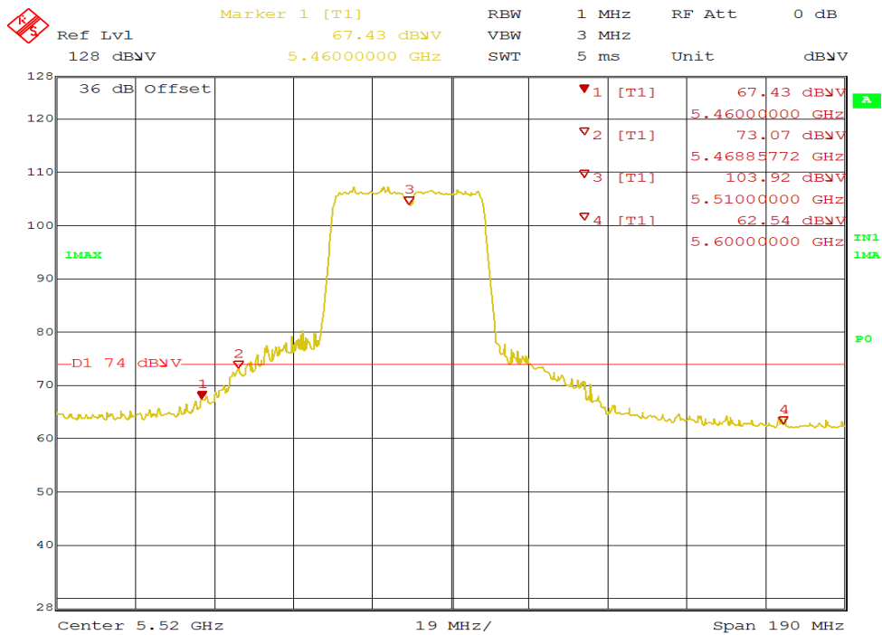
Figure 37: Radiated Emission 5470 MHz Edge for HT40 5510 MHz – Vert. (Pk)
