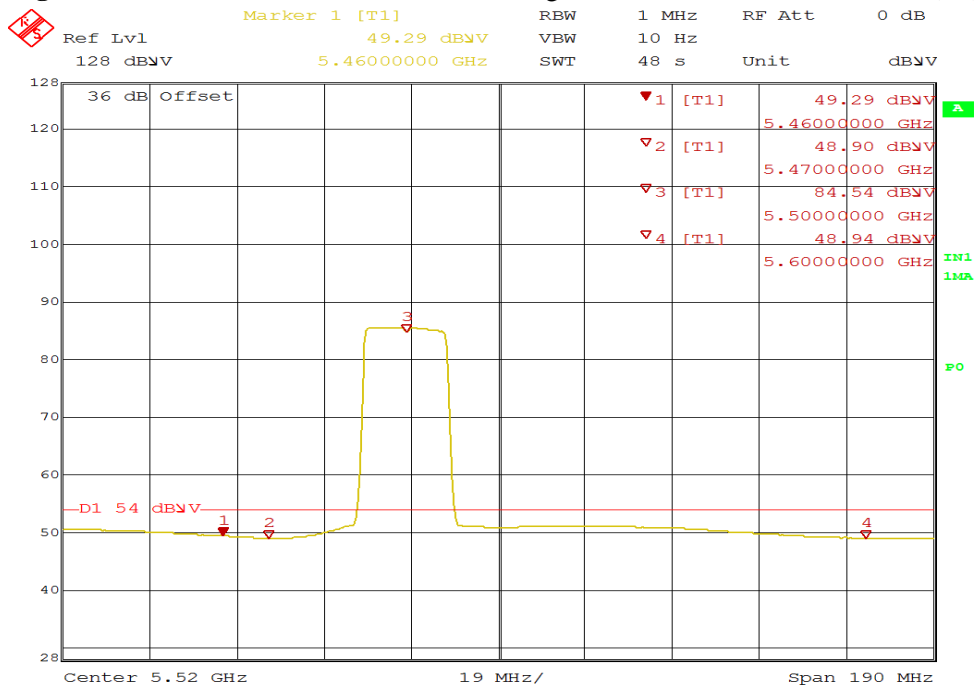
Figure 33: Radiated Emission 5470 MHz Edge for HT20 5500 MHz – Horz. (Pk)
