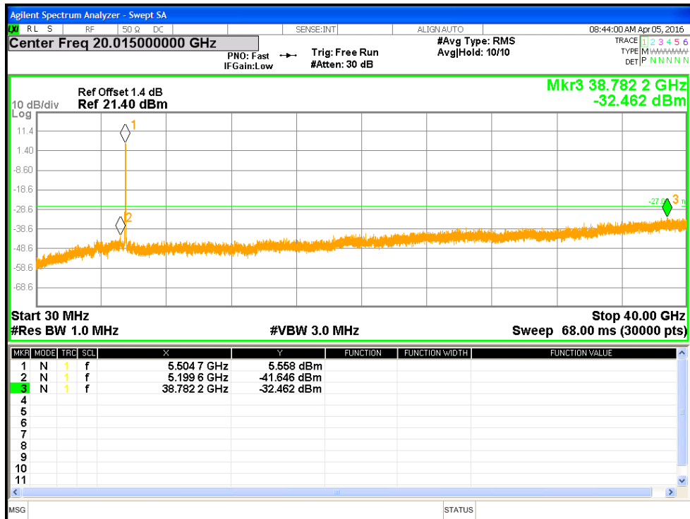
Figure 21: Undesirable Emission for HT40-MCS0 at 5510 MHz
