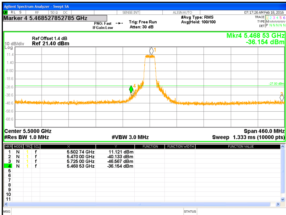
Figure 10: Measured Bandedge for 802.11a-6Mbps at 5500 MHz
