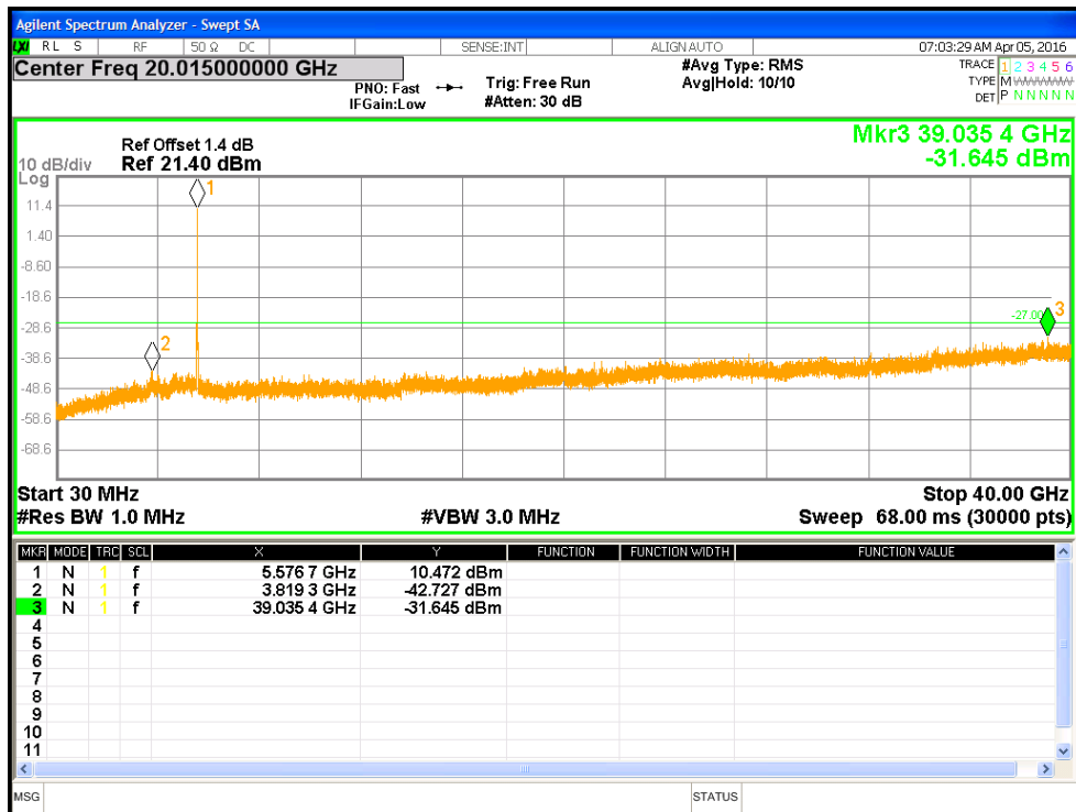
Figure 12: Undesirable Emission for 802.11a-6Mbps at 5580 MHz
