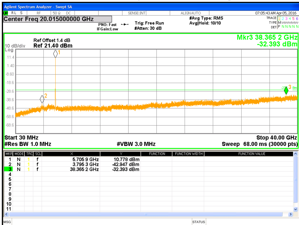
Figure 14: Undesirable Emission for 802.11a-6Mbps at 5700 MHz
