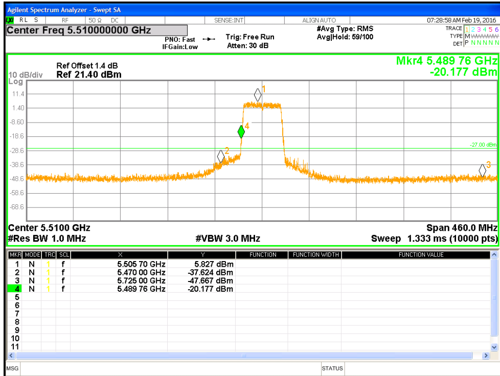
Figure 20: Measured Bandedge for HT40-MCS0 at 5510 MHz
