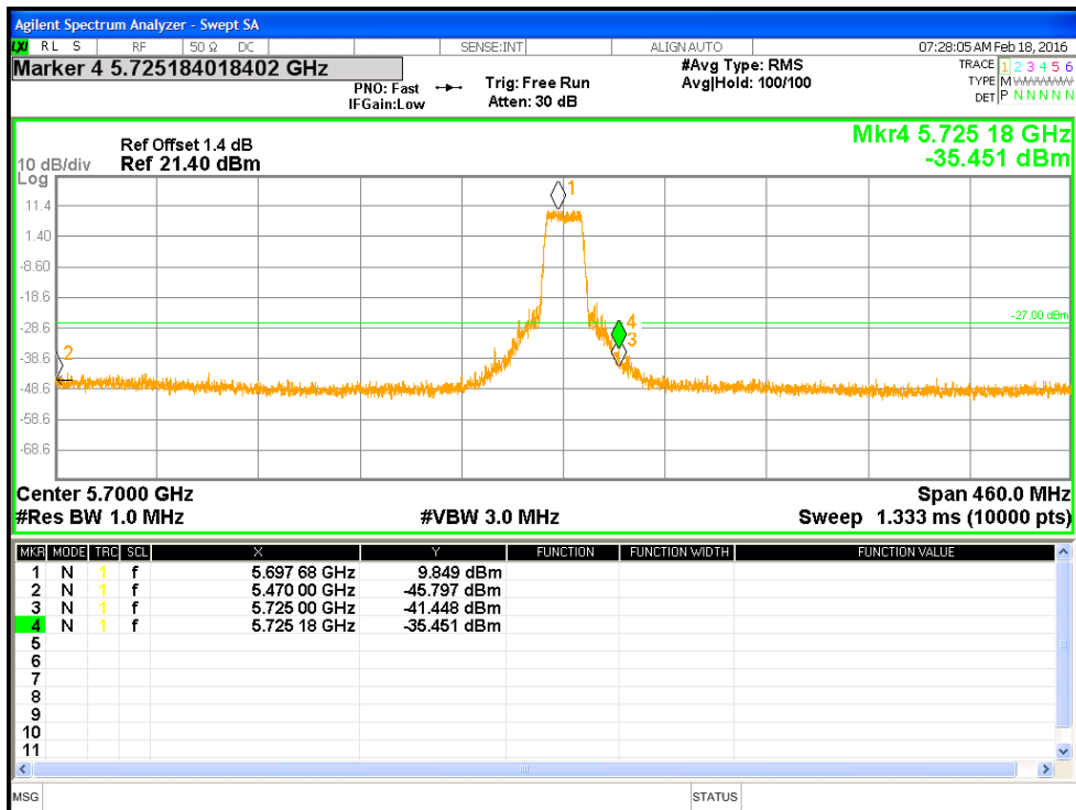
Figure 13: Measured Bandedge for 802.11a-6Mbps at 5700 MHz
