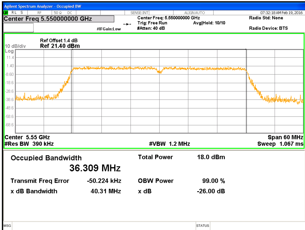
Figure 6: 26dB & 99% Occupied Bandwidth, 5550 MHz at HT40 MCS0
