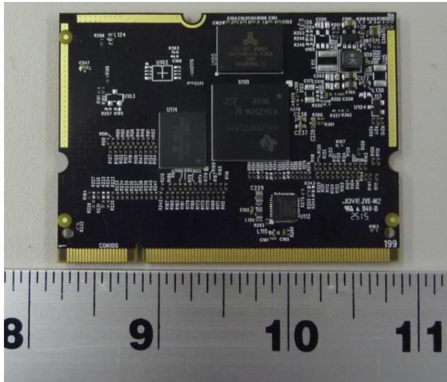
Figure 5: RF module (Bottom)
