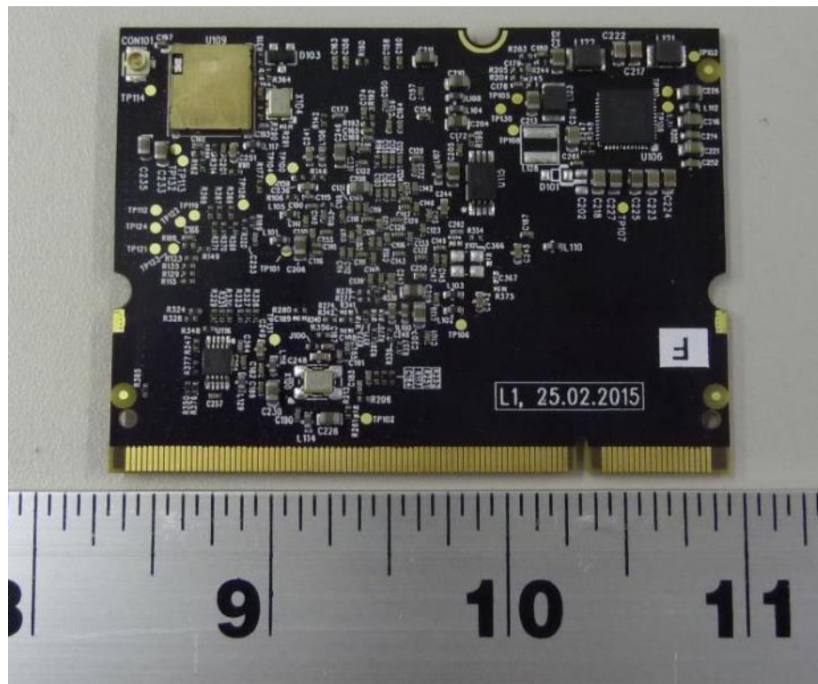
Figure 4: RF module (Top)
