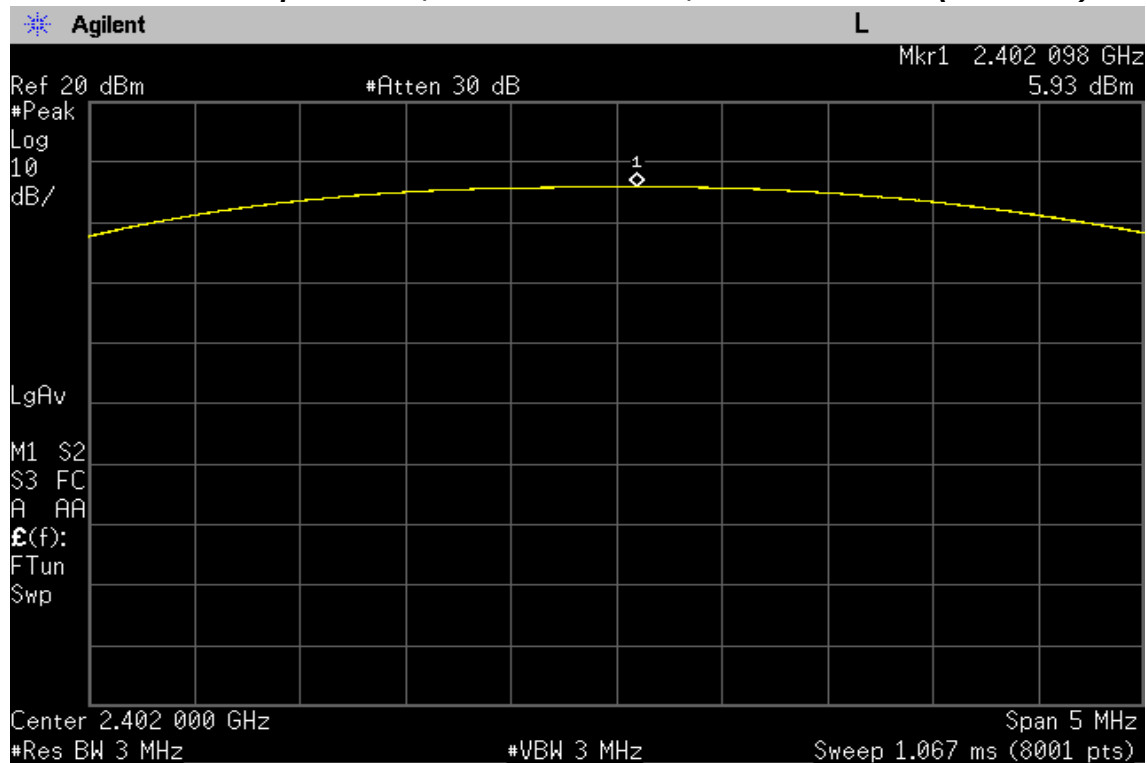
Maximum Peak Output Power, GFSK modulation, Lowest Channel (2402 MHz)
