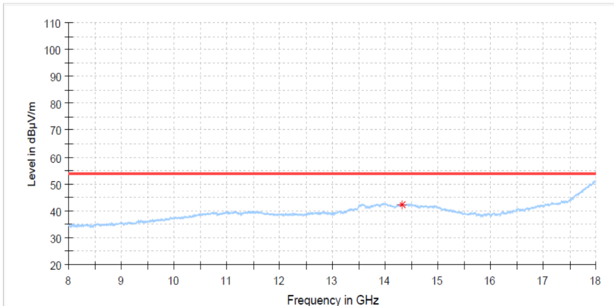
Lowest channel : 8 GHz to 18 GHz_Average
