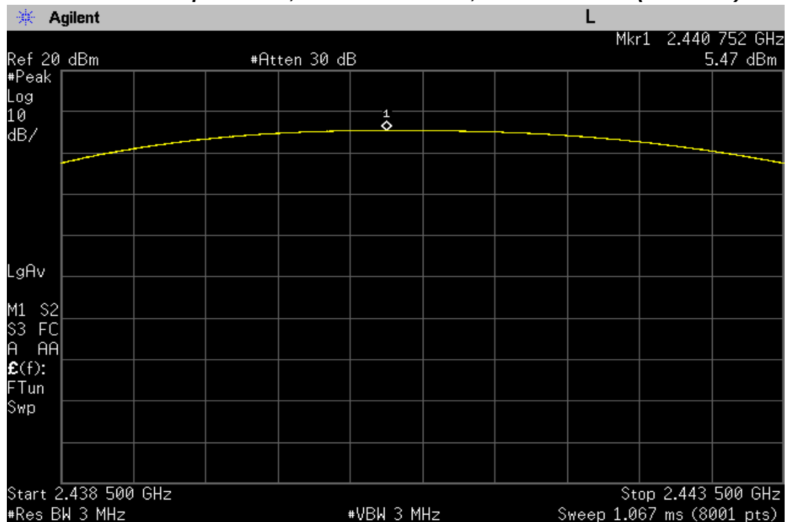
Maximum Peak Output Power, GFSK modulation, Middle Channel (2441 MHz)
