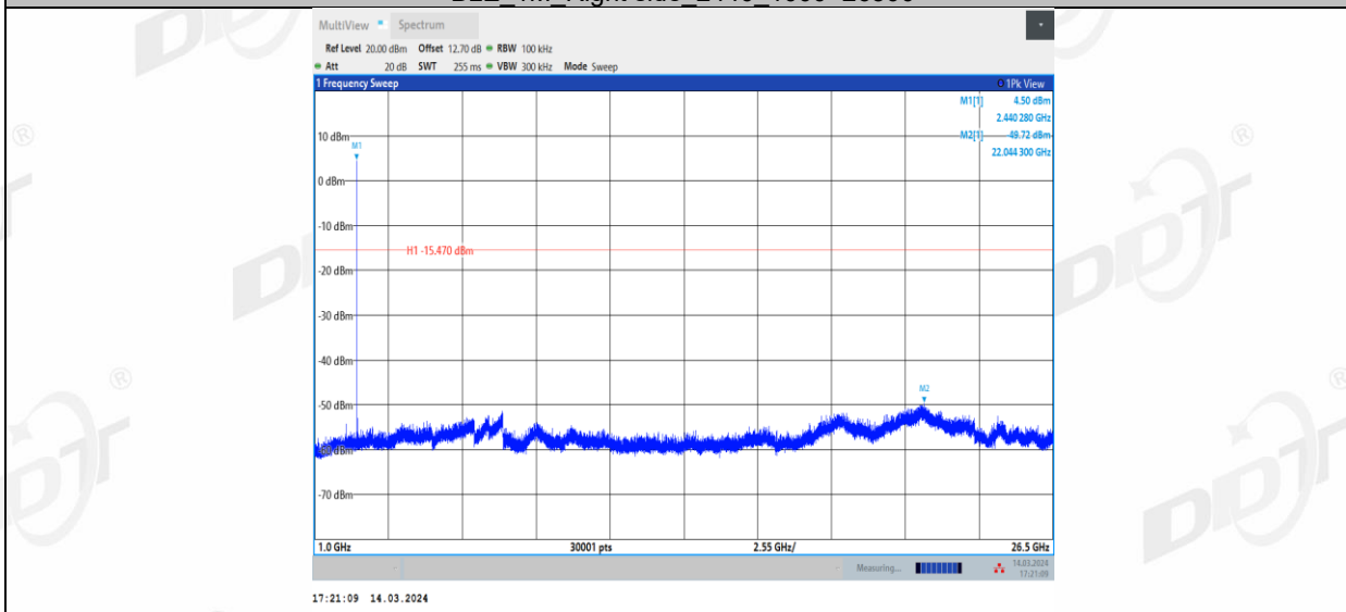
BLE_1M_Left side_2440_0~Reference
