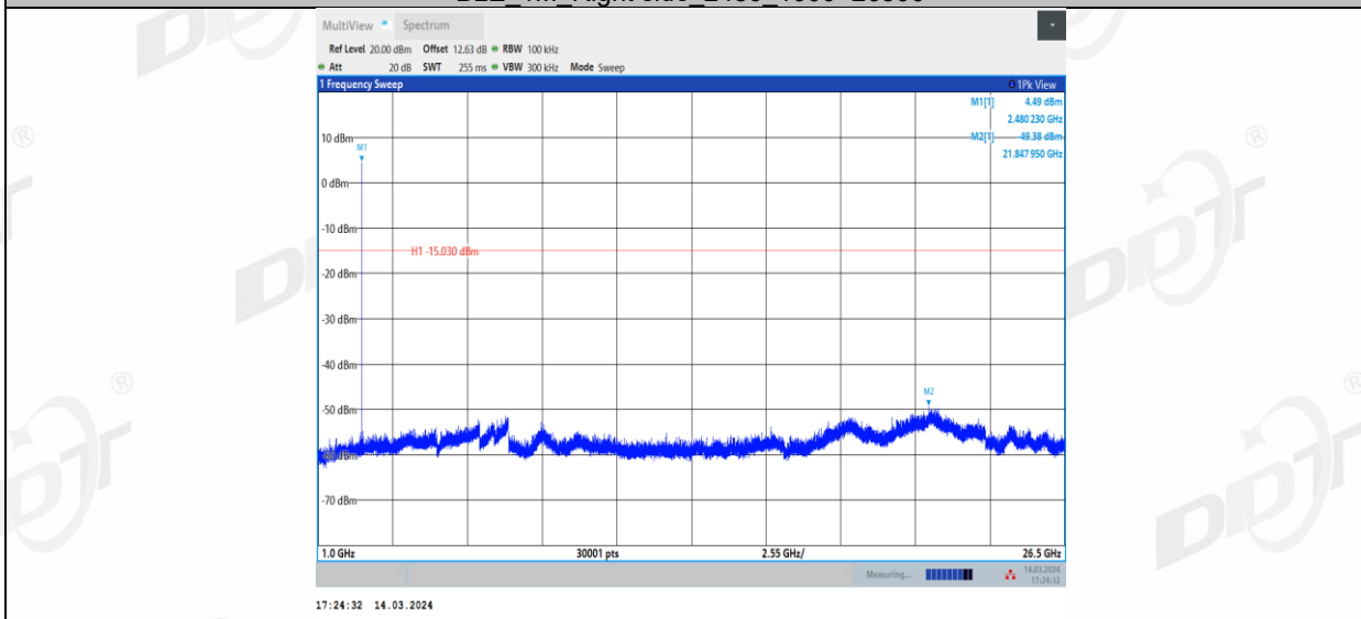
BLE_1M_Left side_2480_0~Reference
