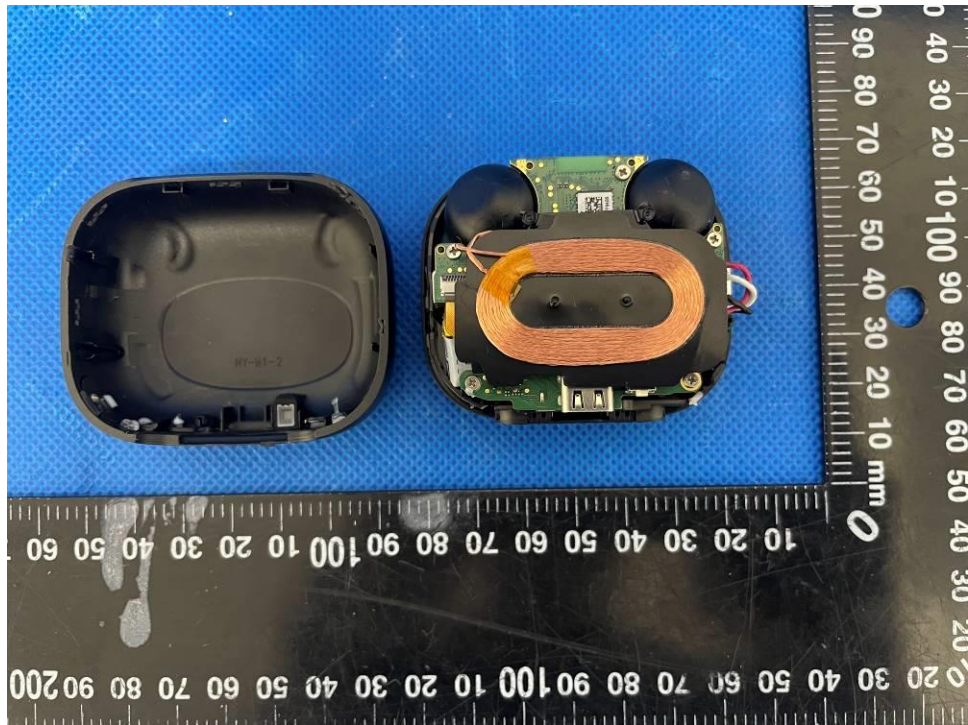
Figure 1 Internal view 1 of charging case
