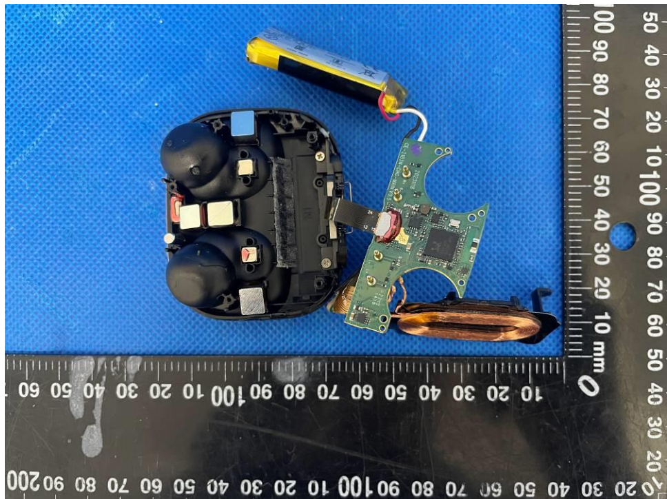
Figure 2 Internal view 2 of charging case
