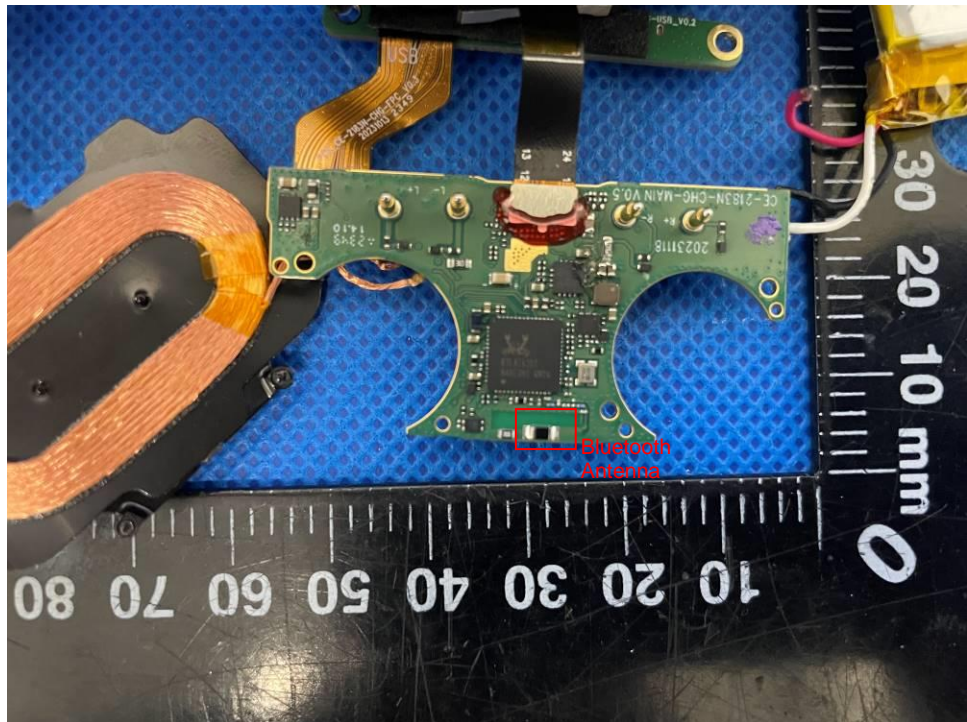
Figure 3 PCB view 1 of charging case
