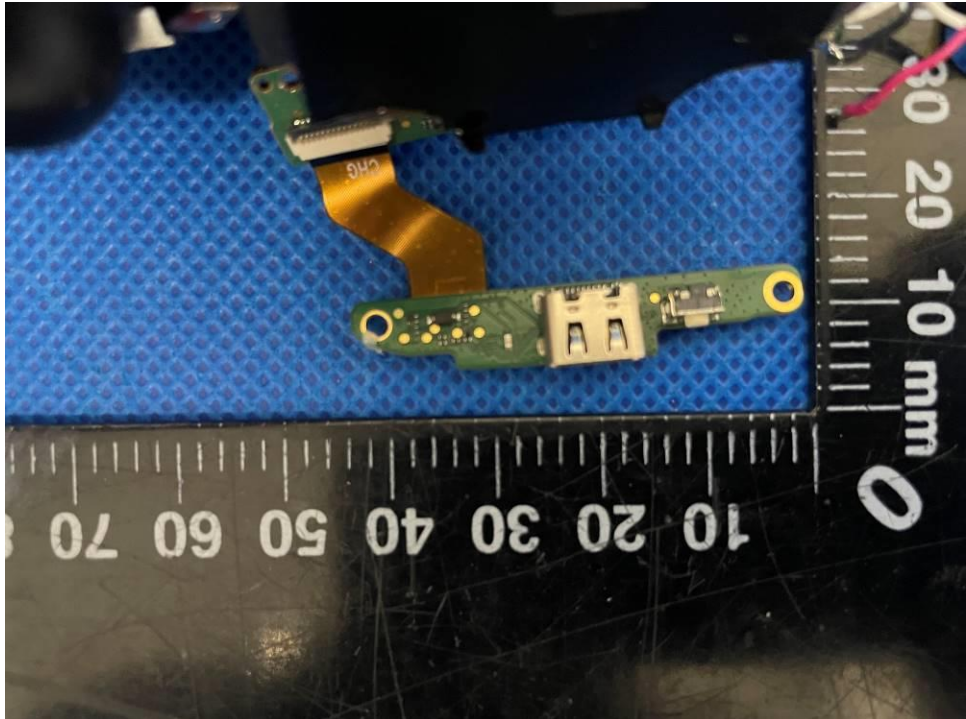
Figure 5 PCB view 3 of charging case
