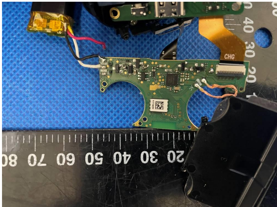
Figure 4 PCB view 2 of charging case
