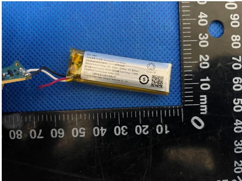
Figure 7 Battery view of charging case
