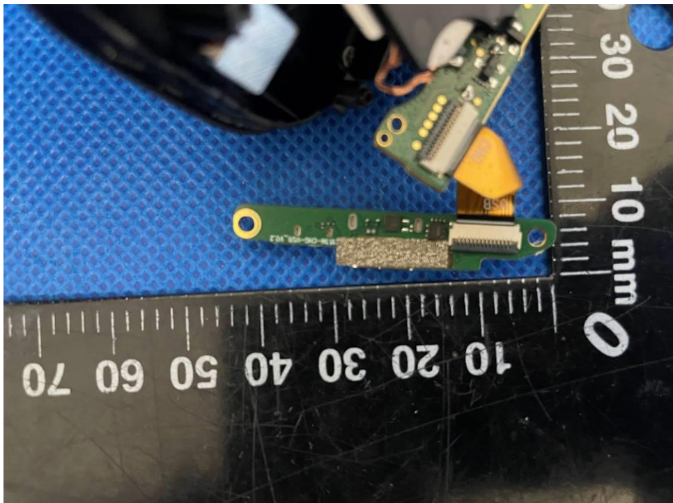
Figure 6 PCB view 4 of charging case
