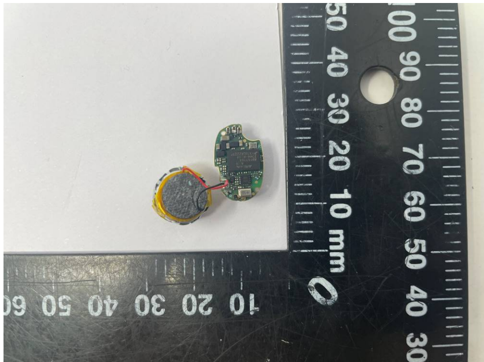
Figure 9 Internal view 4 of R earbud (HW Version: V0.4)
