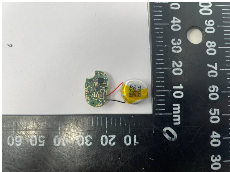
Figure 8 Internal view 3 of R earbud (HW Version: V0.3)
