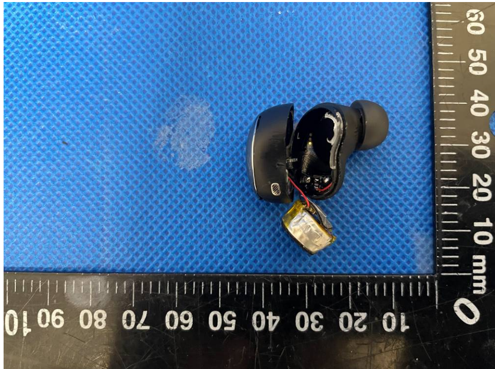
Figure 1 Internal view 1 of L earbud
