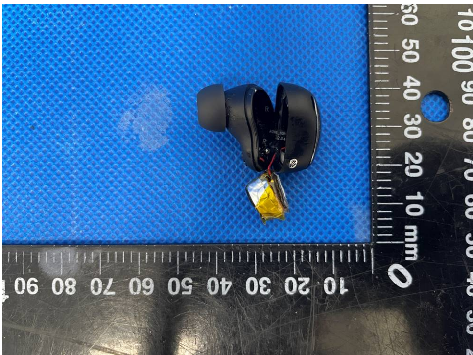
Figure 6 Internal view 1 of R earbud
