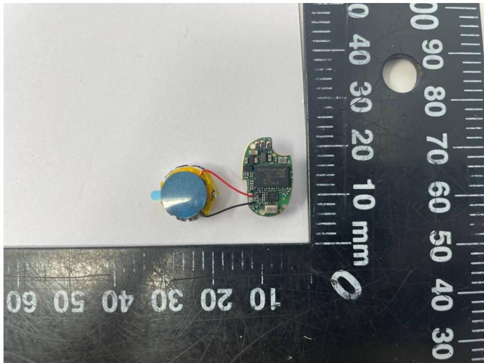
Figure 7 Internal view 2 of R earbud (HW Version: V0.3)
