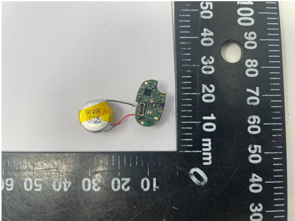
Figure 3 Internal view 3 of L earbud (HW Version: V0.3)
