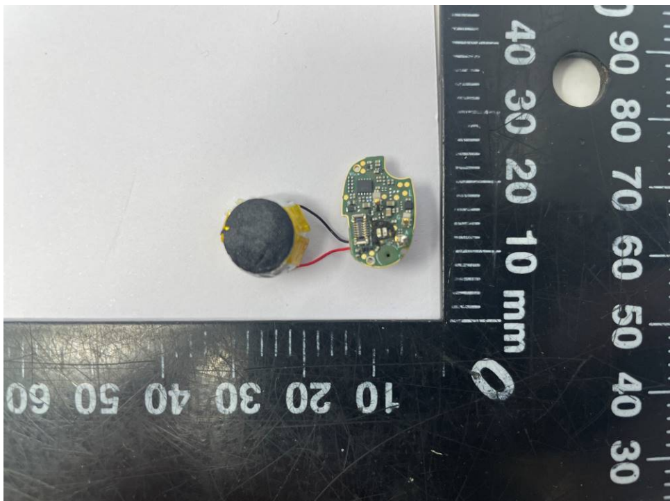
Figure 4 Internal view 4 of L earbud (HW Version: V0.4)
