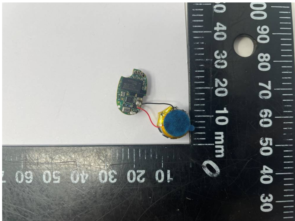
Figure 2 Internal view 2 of L earbud (HW Version: V0.3)
