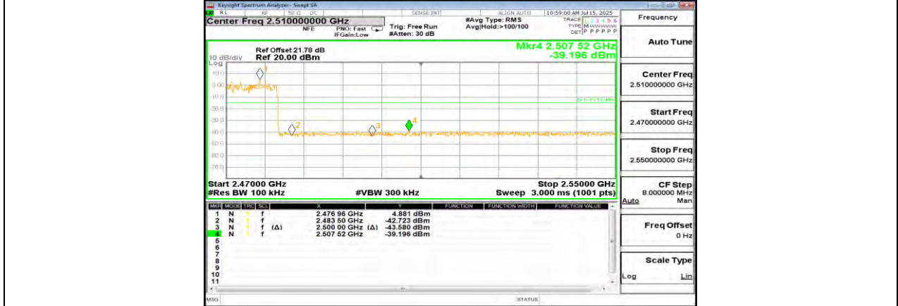
3DH5_Ant1_High_Hop_2480
