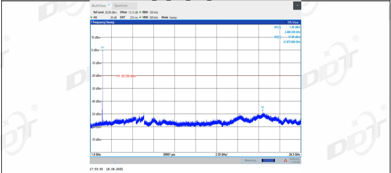
BLE_2M_Ant1_2402_0~Reference
