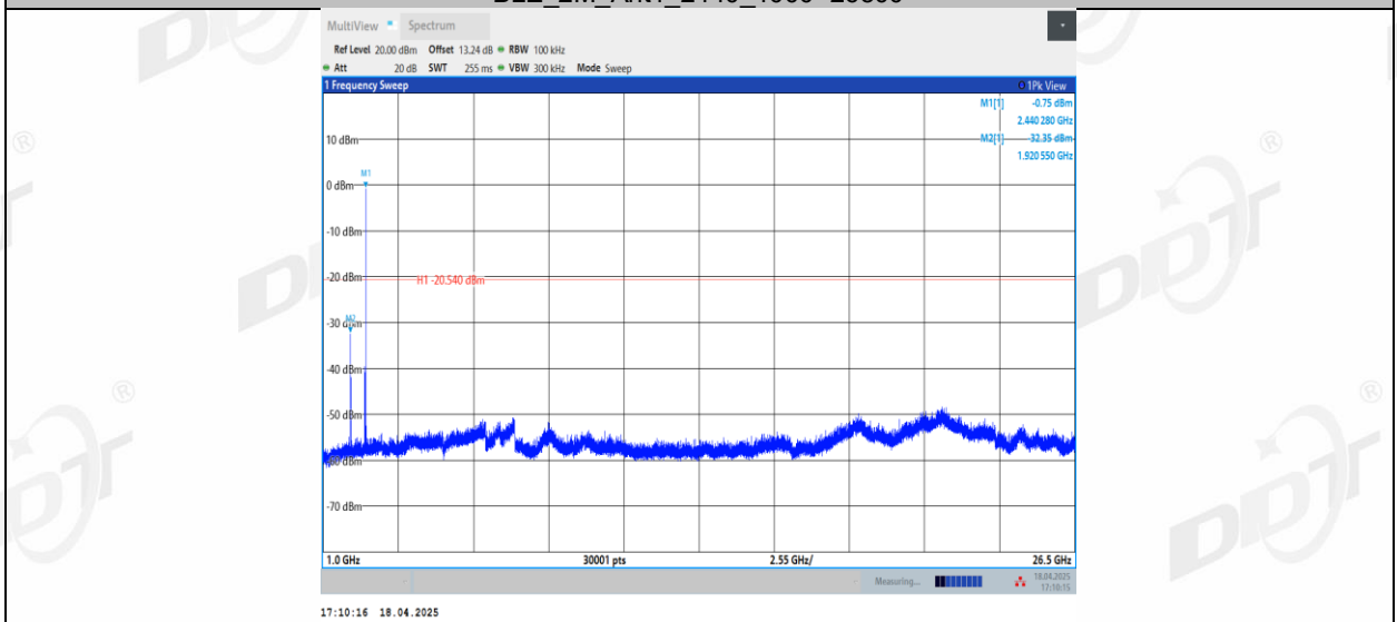
BLE_2M_Ant1_2480_0~Reference
