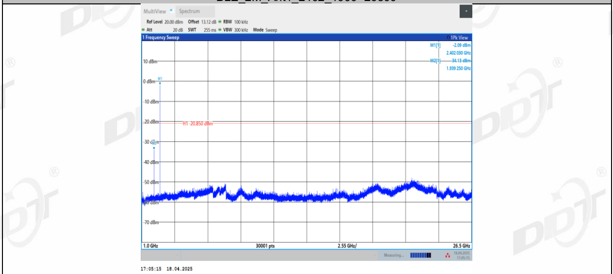
BLE_2M_Ant1_2440_0-Reference
