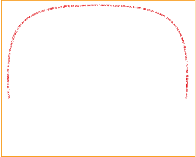
OPTION1 Compliance inner top cover IN-MOLD, depth, ref live beam3 /// materials: PC+ABS Finishing: glossy
