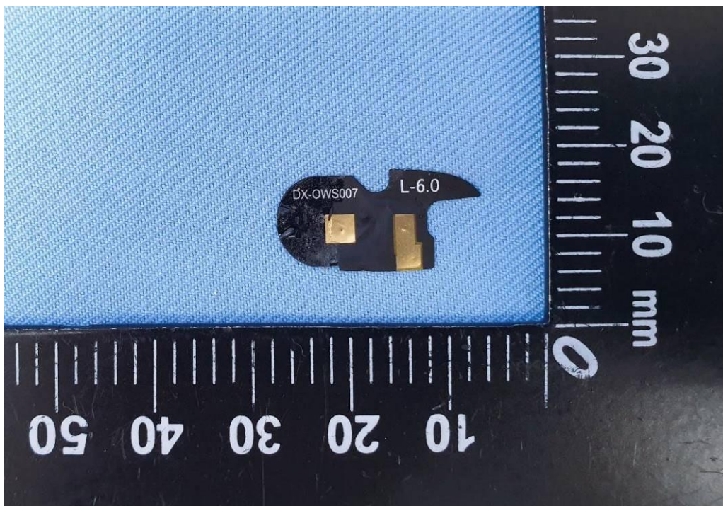
Figure 13 Bluetooth Antenna_Left earbud
