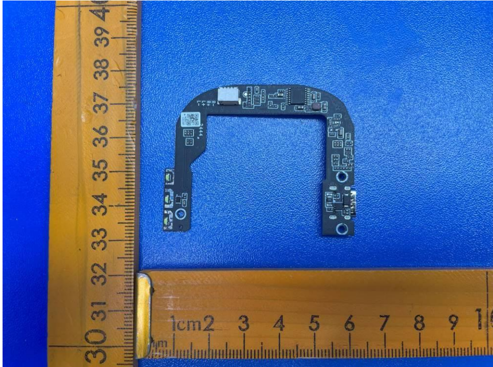
Figure 3 PCB view 1(Charging case)
