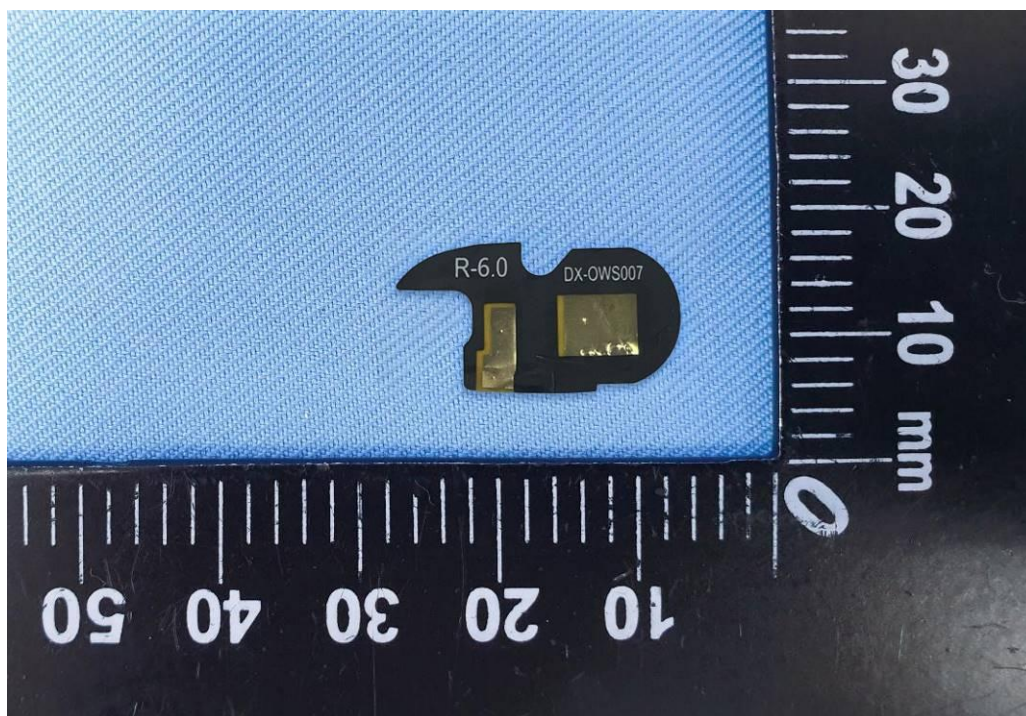
Figure 14 Bluetooth Antenna_Right earbud
