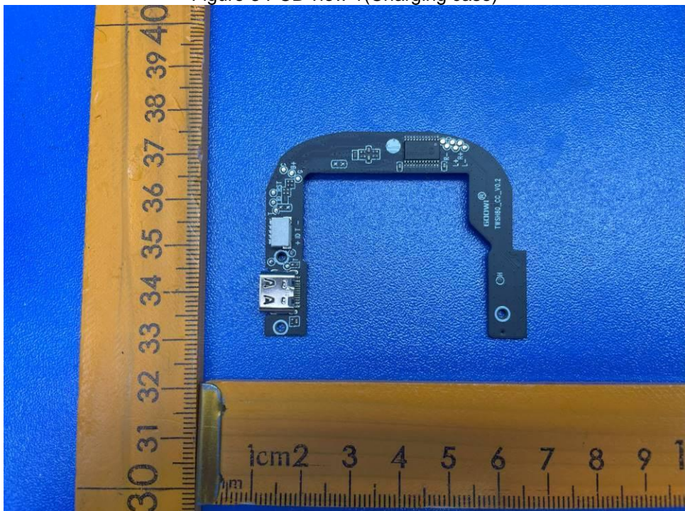
Figure 4 PCB view 2(Charging case)
