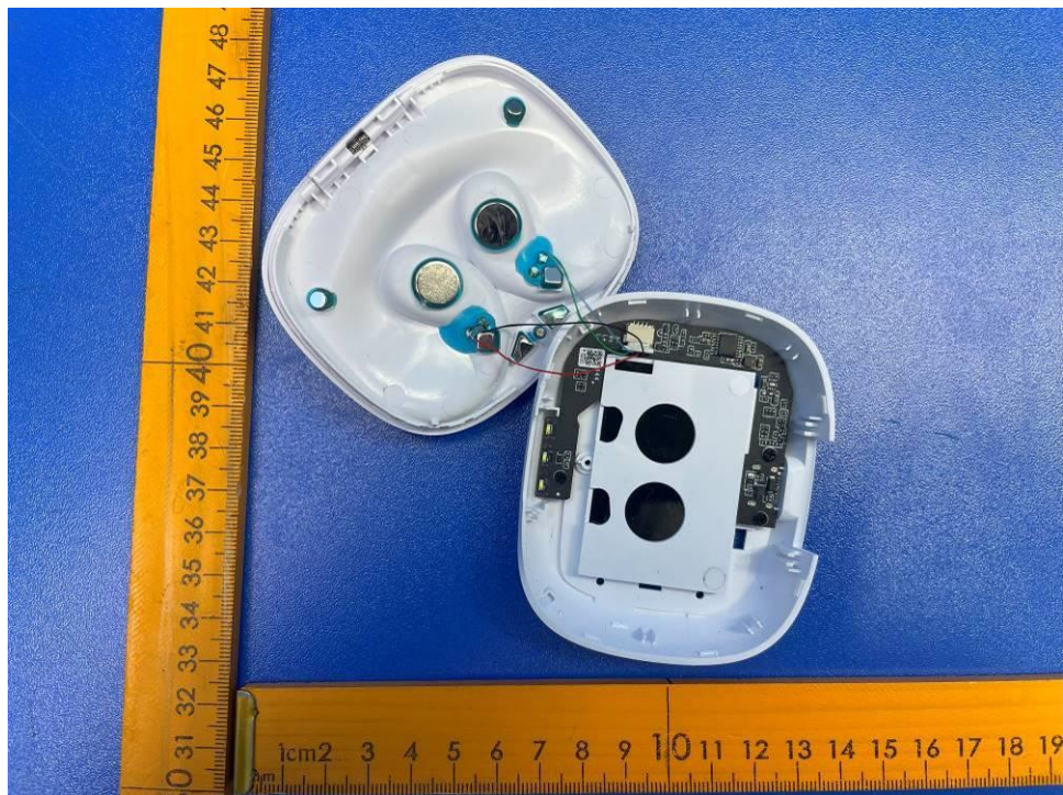
Figure 2 Internal view 2 (Charging case)
