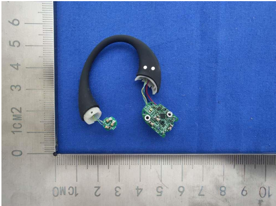
Figure 9 PCB view 2 (L earbud)
