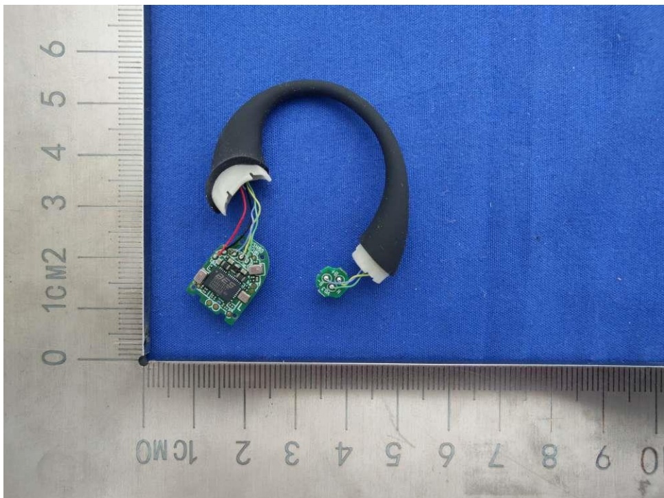
Figure 8 PCB view 1 (L earbud)
