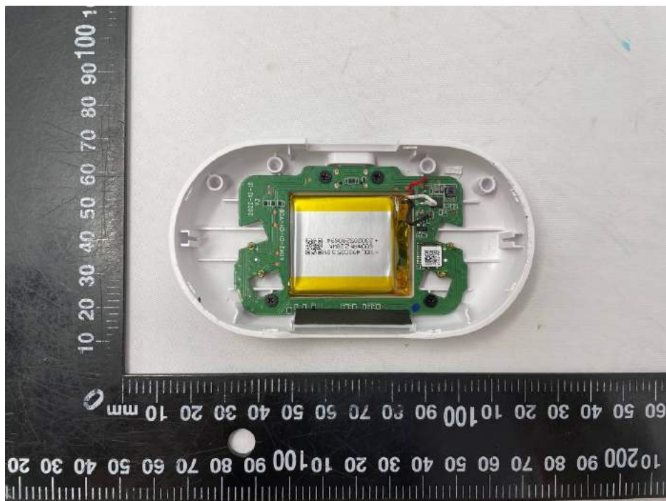
Figure 7: Internal view-2 (charging case)
