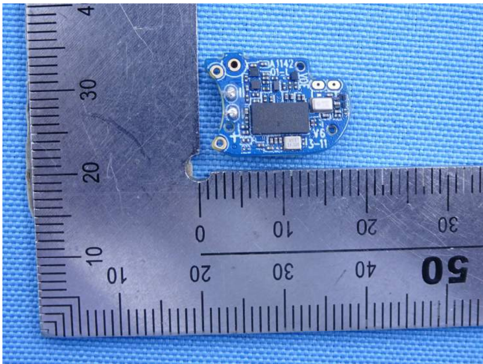
Figure 20: Main board bottom view (earbuds)
