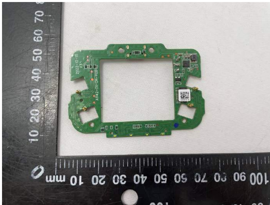
Figure 10: Main board top view (charging case)
