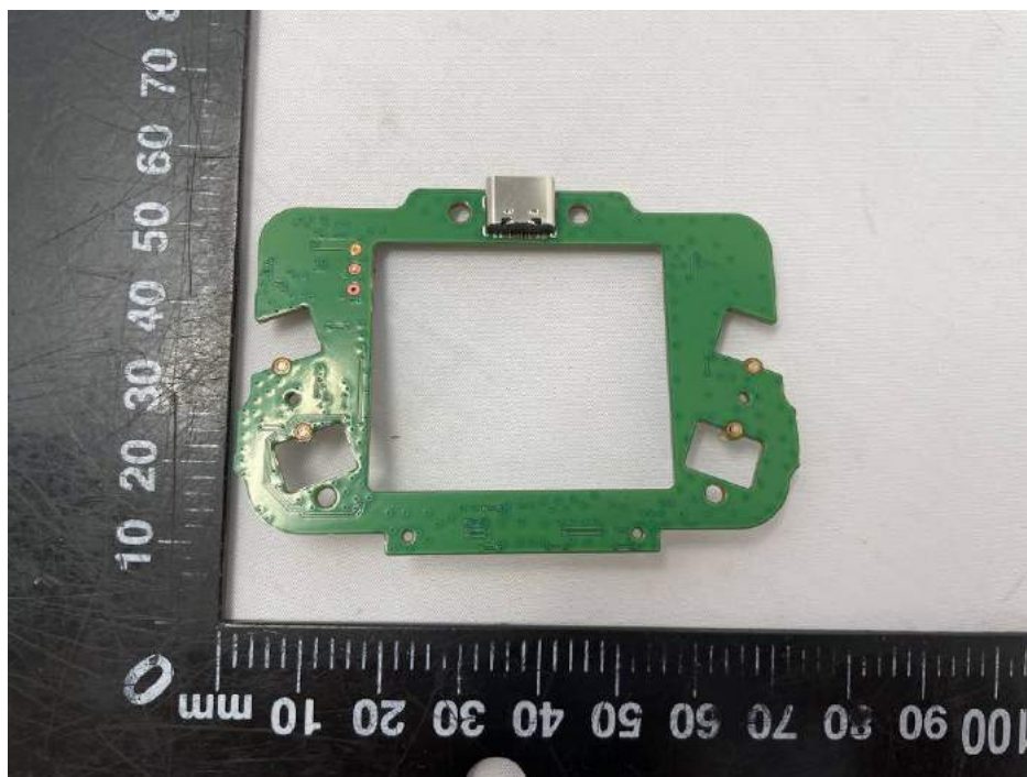
Figure 11: Main board bottom view (charging case)
