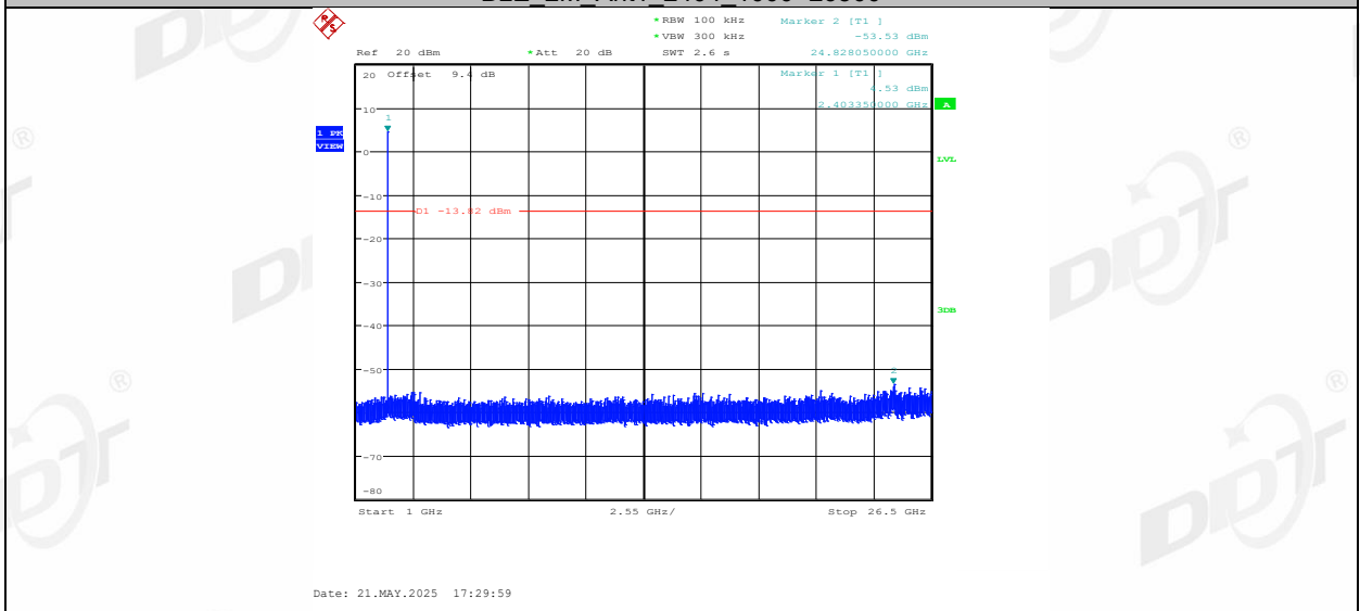
BLE_2M_Ant1_2440_0-Reference
