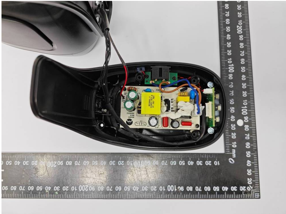
Figure 2. Internal view of PARTYLIGHT BEAM
