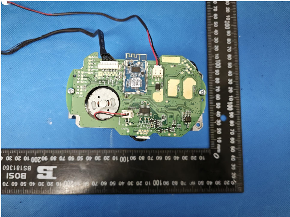
Figure 8. Internal view of PARTYLIGHT BEAM
