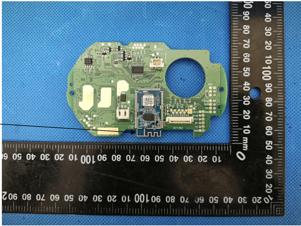
Figure 9. Front view of control PCB
