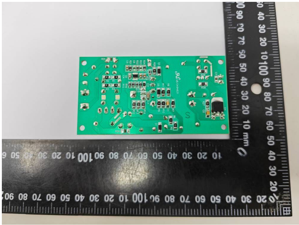
Figure 17. Back view of LED driver
