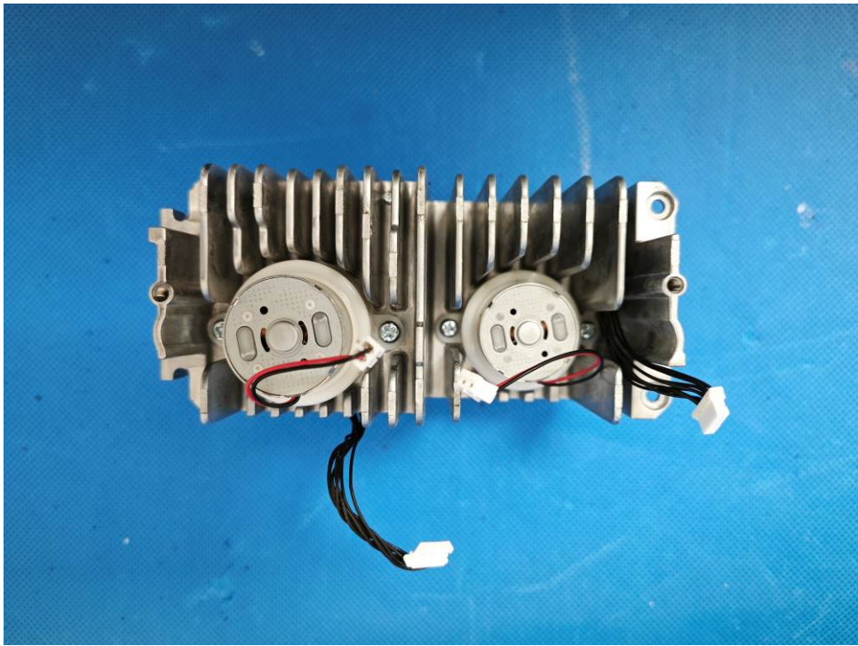
Figure 11. Internal view of PARTYLIGHT BEAM
