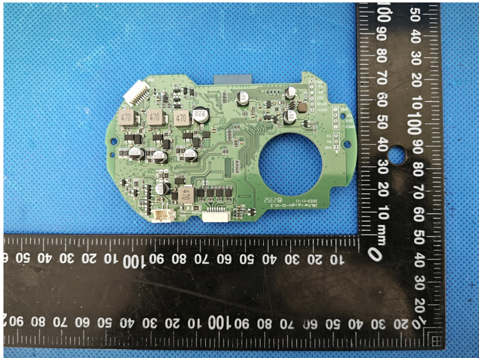
Figure 10. Back view of control PCB
