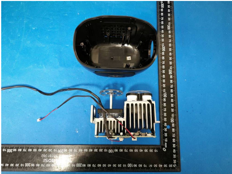
Figure 7. Internal view of PARTYLIGHT BEAM
