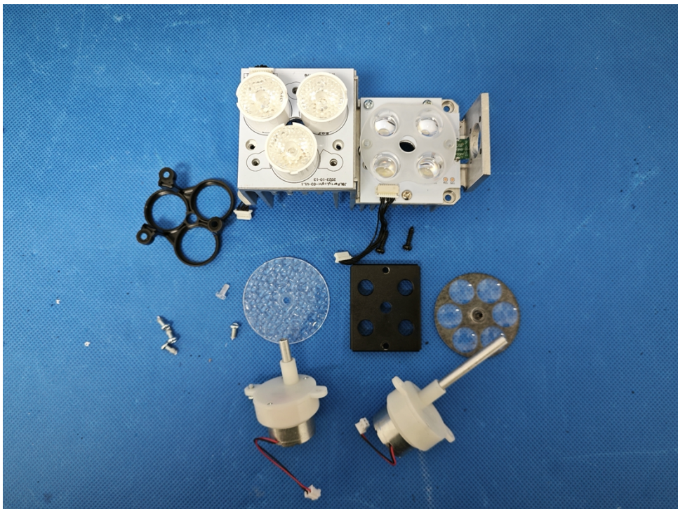
Figure 12. Internal view of PARTYLIGHT BEAM
