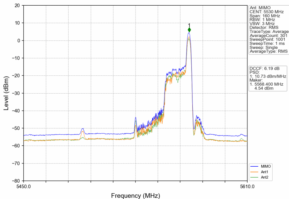
802.11ax(HEW80)_LCH_5530MHz_RU26_Right_MIMO_NTNV
