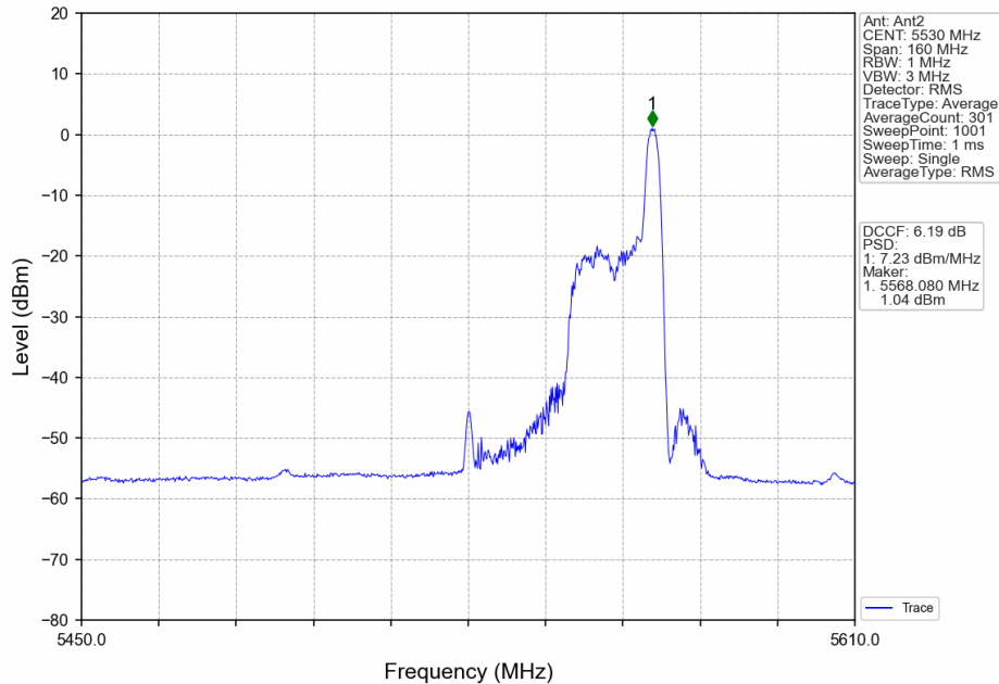
802.11ax(HEW80)_LCH_5530MHz_RU26_Right_MIMO_NTNV
