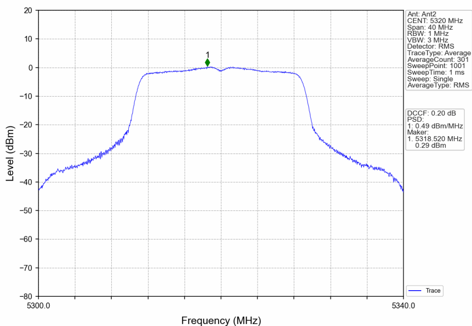
802.11ac(VHT20)_HCH_5320MHz_Ant2_NTNV
