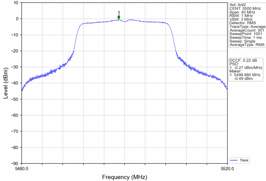
802.11ac(VHT20)_LCH_5500MHz_MIMO_NTNV
