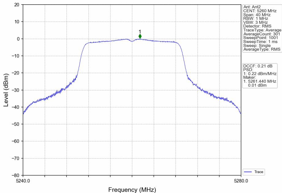
802.11ac(VHT20)_LCH_5260MHz_Ant2_NTNV
