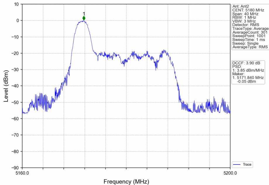
802.11ax(HEW20)_LCH_5180MHz_RU26_Left_MIMO_NTNV
