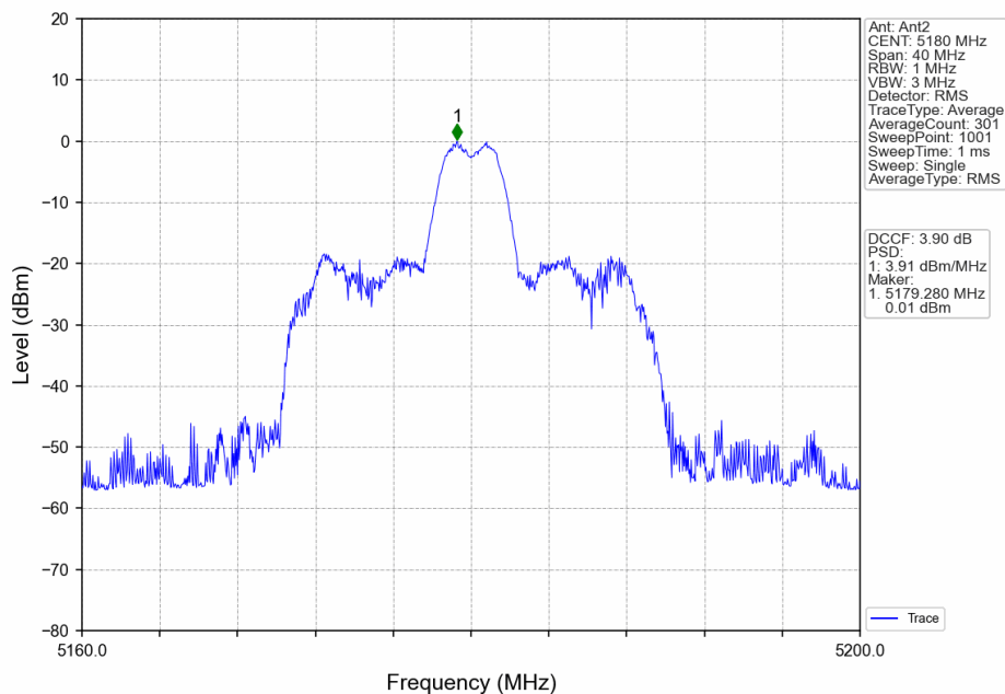
802.11ax(HEW20)_LCH_5180MHz_RU26_Mid_Ant2_NTNV
