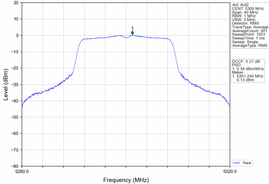
802.11ac(VHT20)_MCH_5300MHz_MIMO_NTNV
