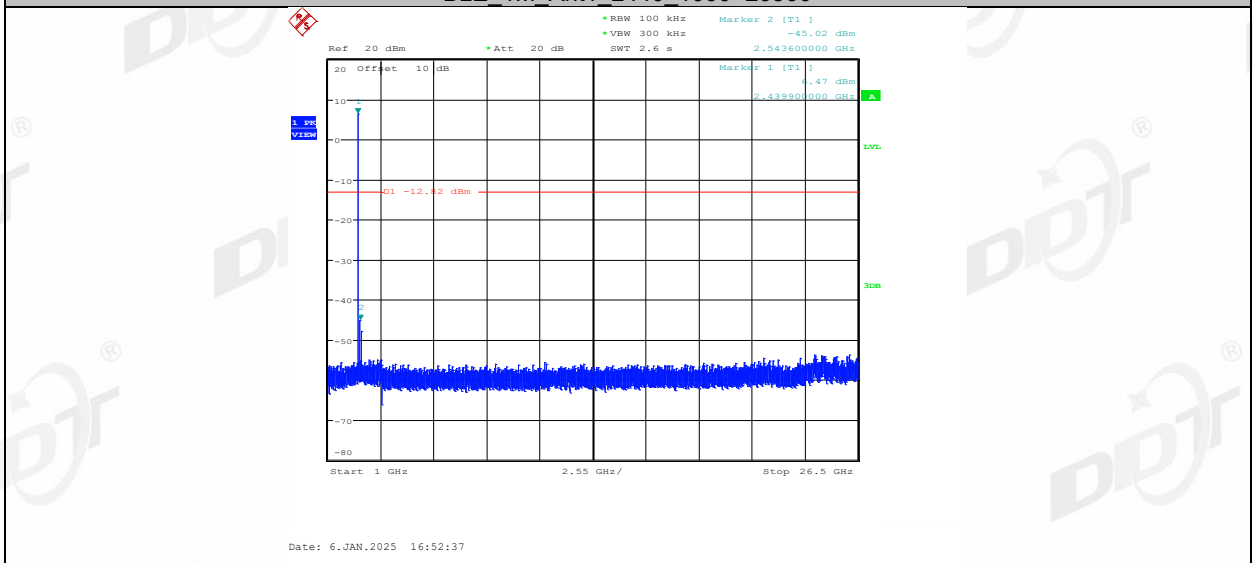
BLE_1M_Ant1_2480_0-Reference
