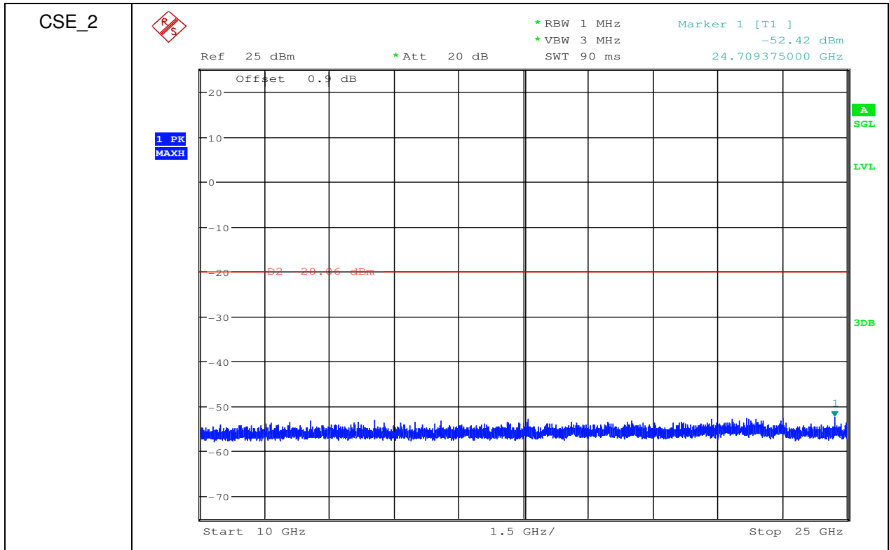
RF Conducted Spurious Emissions_11G_2412
