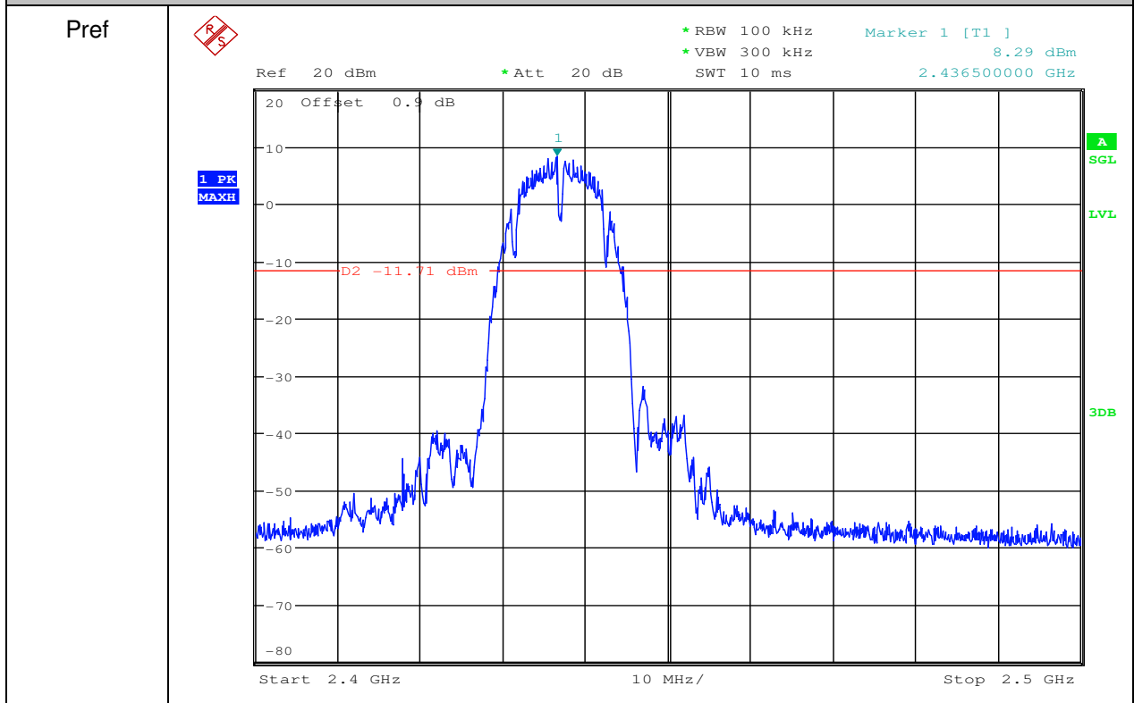
RF Conducted Spurious Emissions_11B_2437
