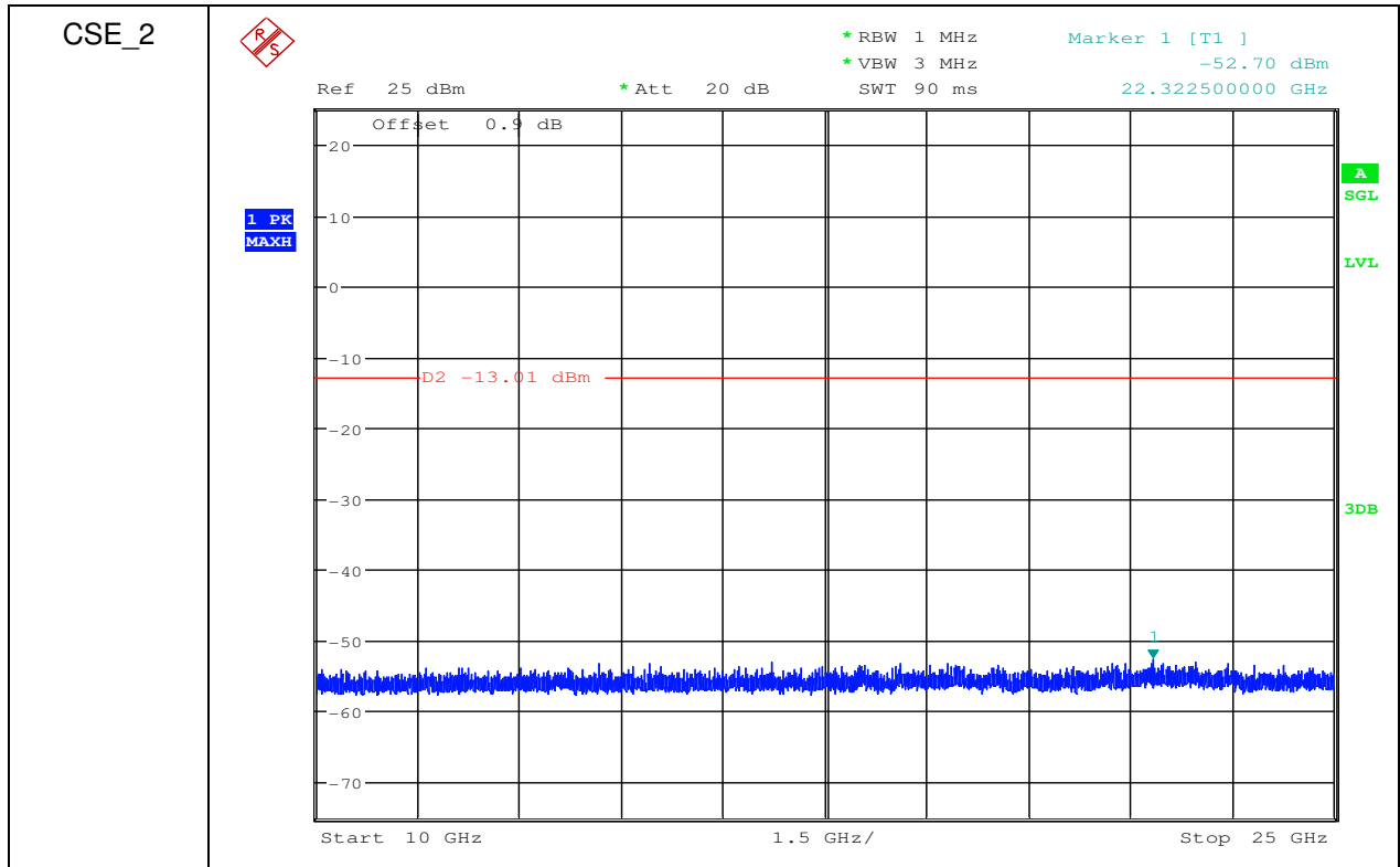
RF Conducted Spurious Emissions_11B_2462
