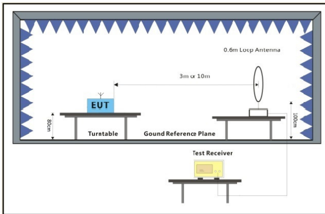
Below 30MHz
