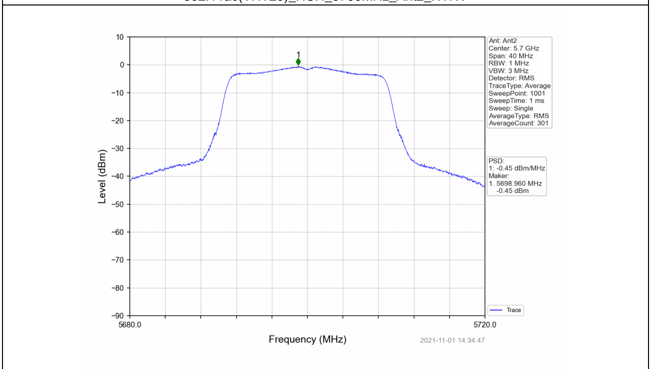
802.11ac(VHT20)_HCH_5700MHz_Ant2_NTNV
