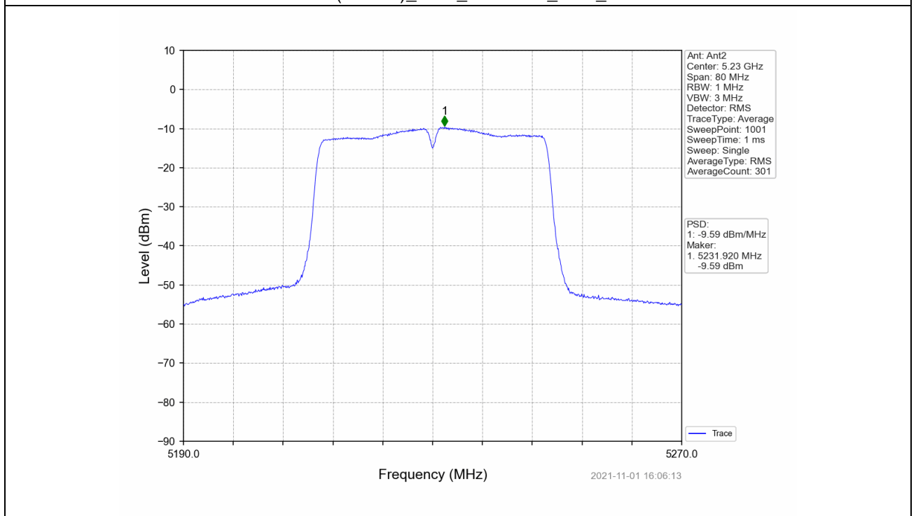
802.11ac(VHT40)_HCH_5230MHz_Ant2_NTNV
