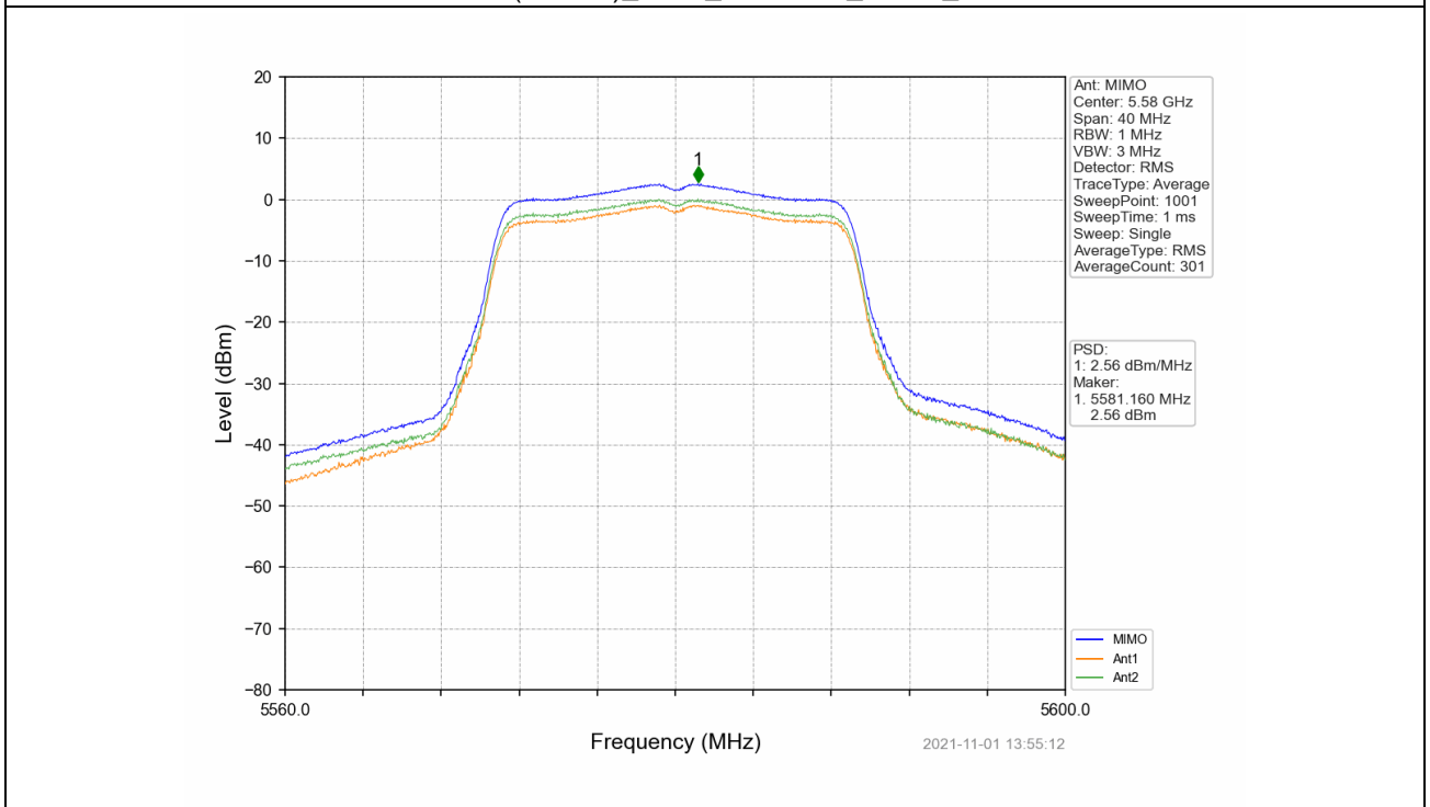
802.11ac(VHT20)_MCH_5580MHz_MIMO_NTNV
