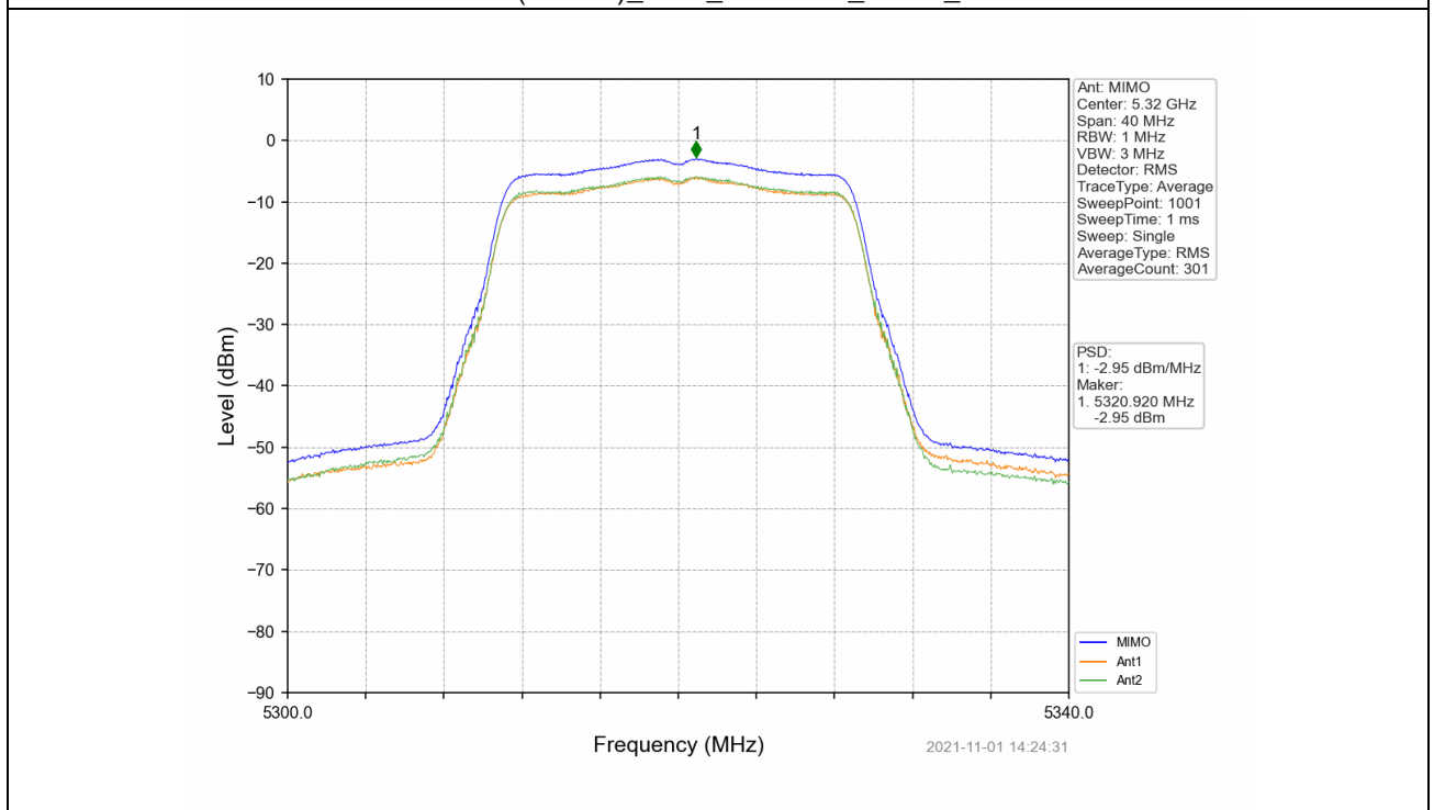
802.11ac(VHT20)_HCH_5320MHz_MIMO_NTNV
