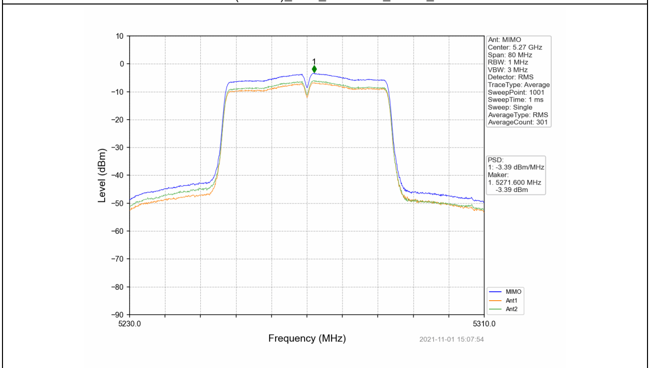
802.11ac(VHT40)_LCH_5270MHz_MIMO_NTNV
