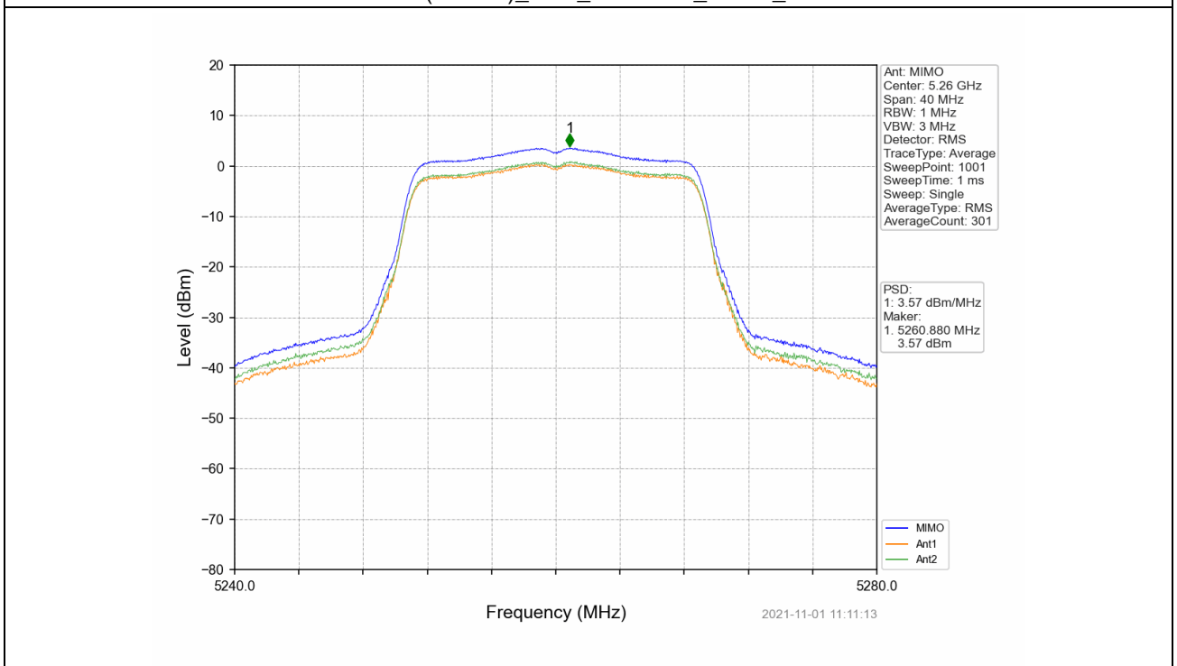
802.11ac(VHT20)_LCH_5260MHz_MIMO_NTNV
