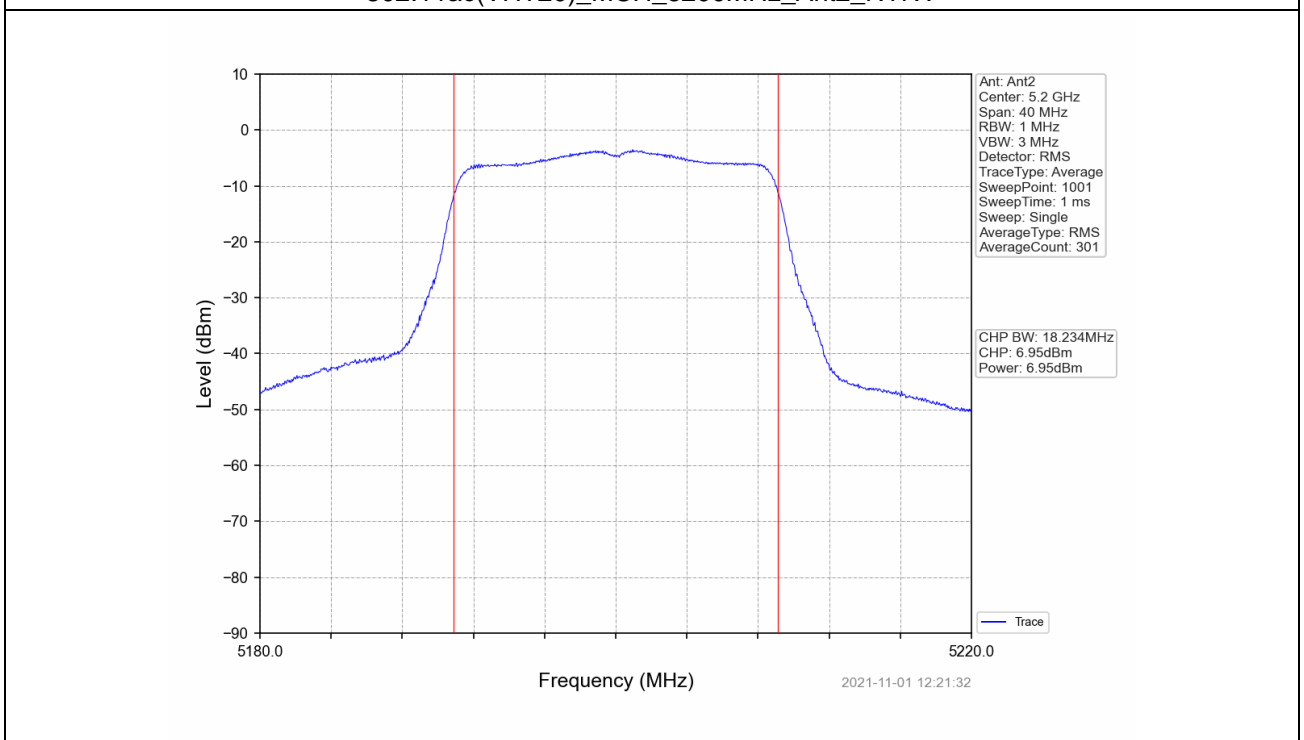
802.11ac(VHT20)_MCH_5200MHz_Ant2_NTNV
