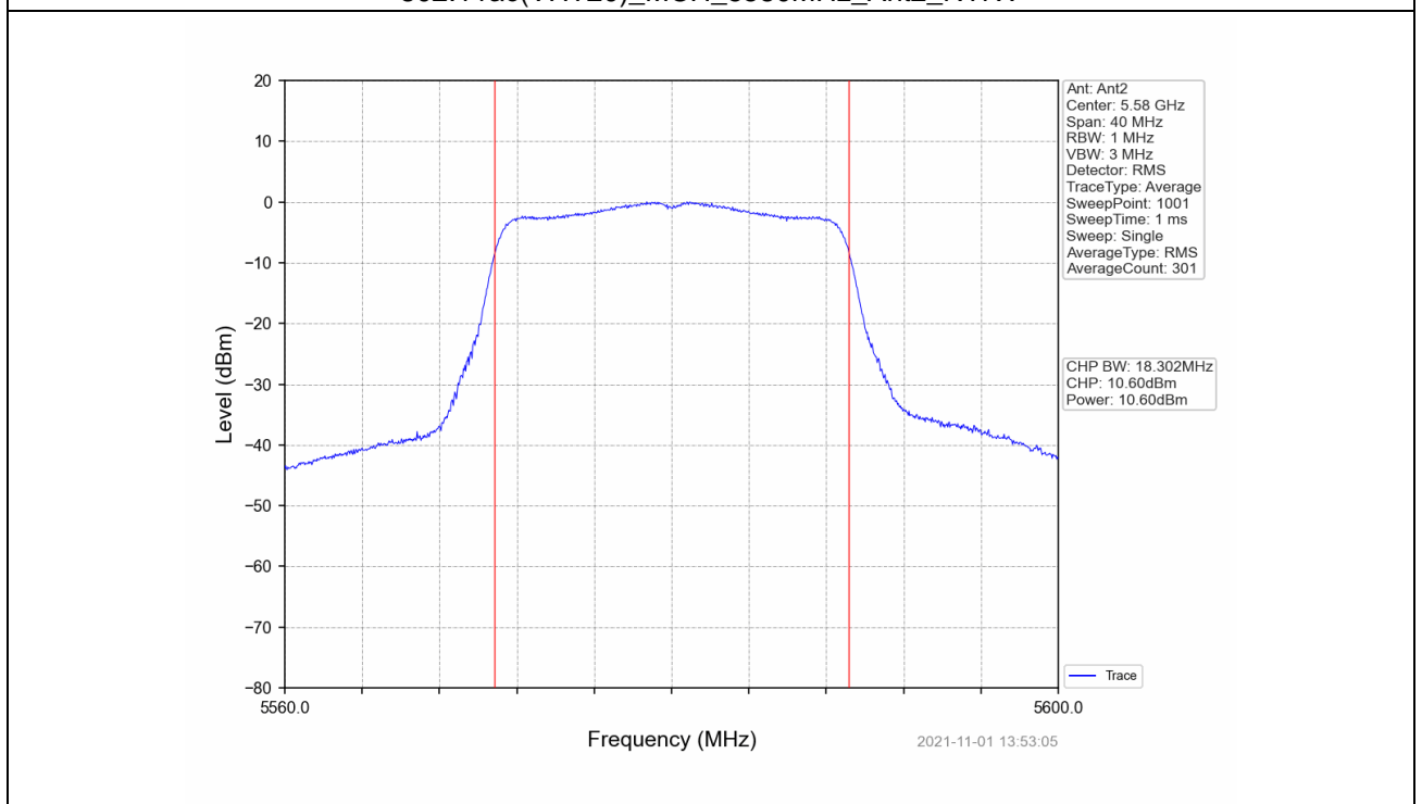
802.11ac(VHT20)_MCH_5580MHz_Ant2_NTNV
