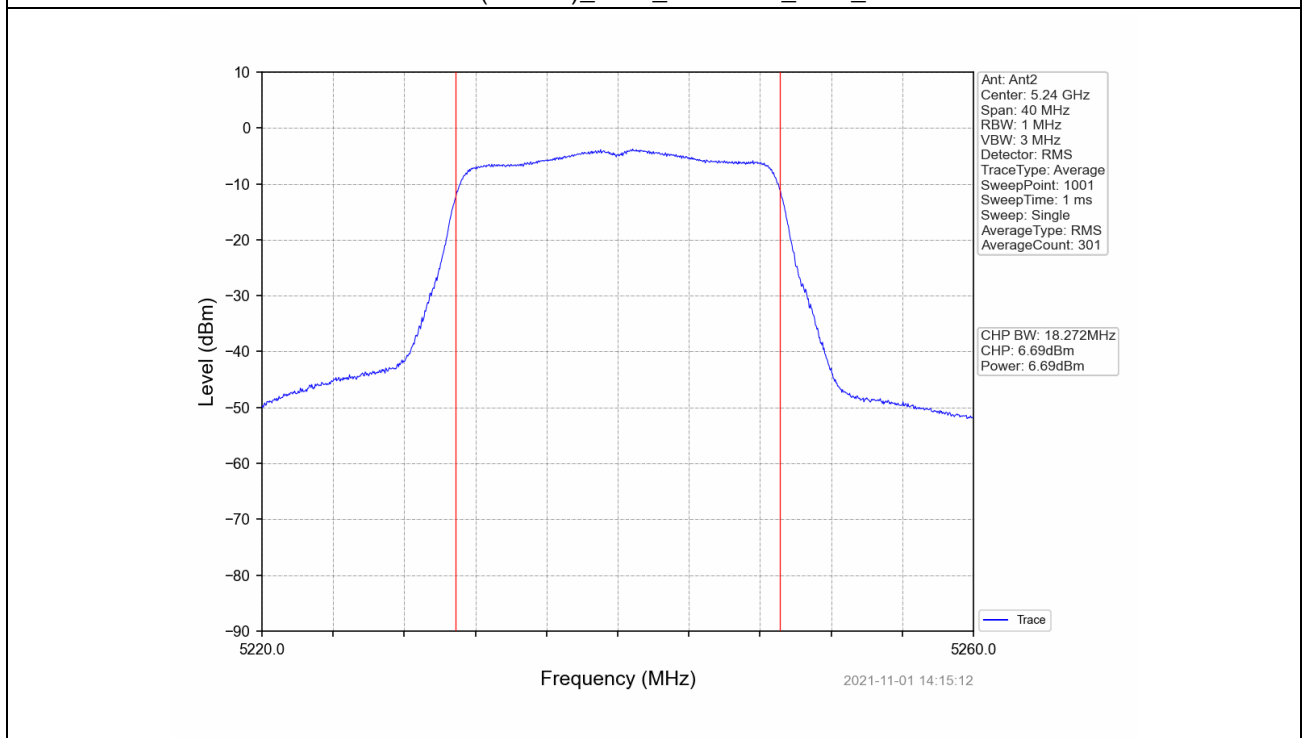
802.11ac(VHT20)_HCH_5240MHz_Ant2_NTNV
