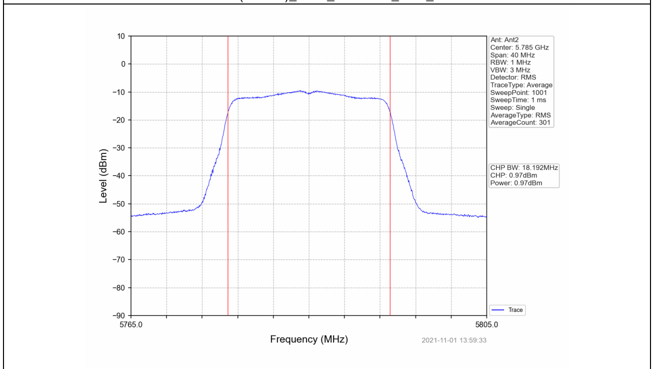
802.11ac(VHT20)_MCH_5785MHz_Ant2_NTNV
