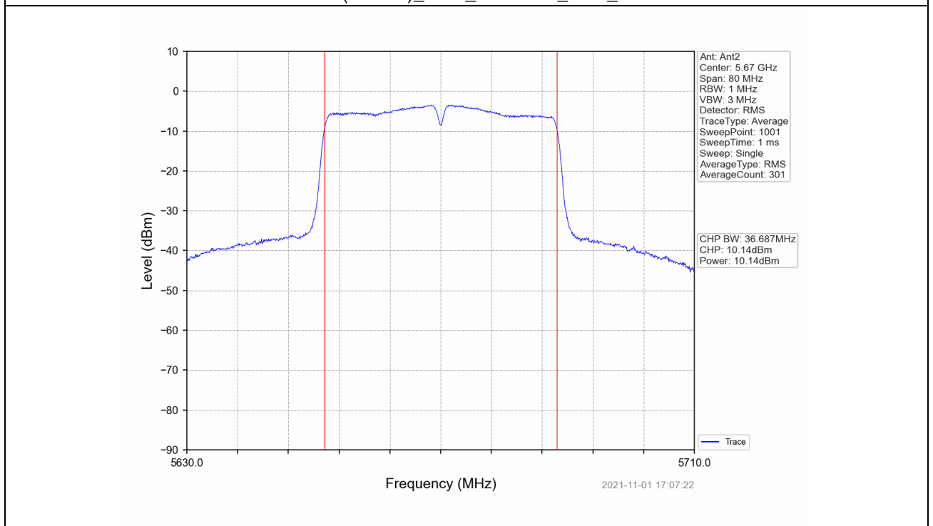
802.11ac(VHT40)_HCH_5670MHz_Ant2_NTNV
