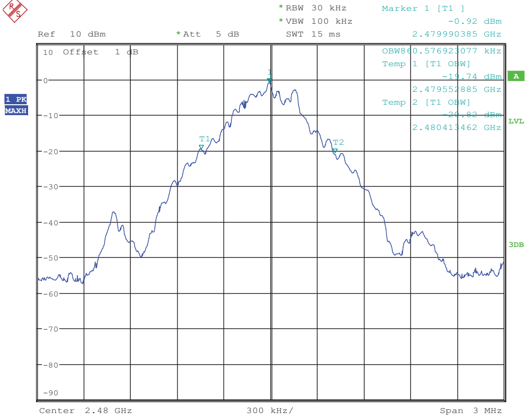
8-DPSK (99% bandwidth)
