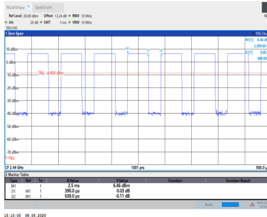
BLE_1M 2440MHz
