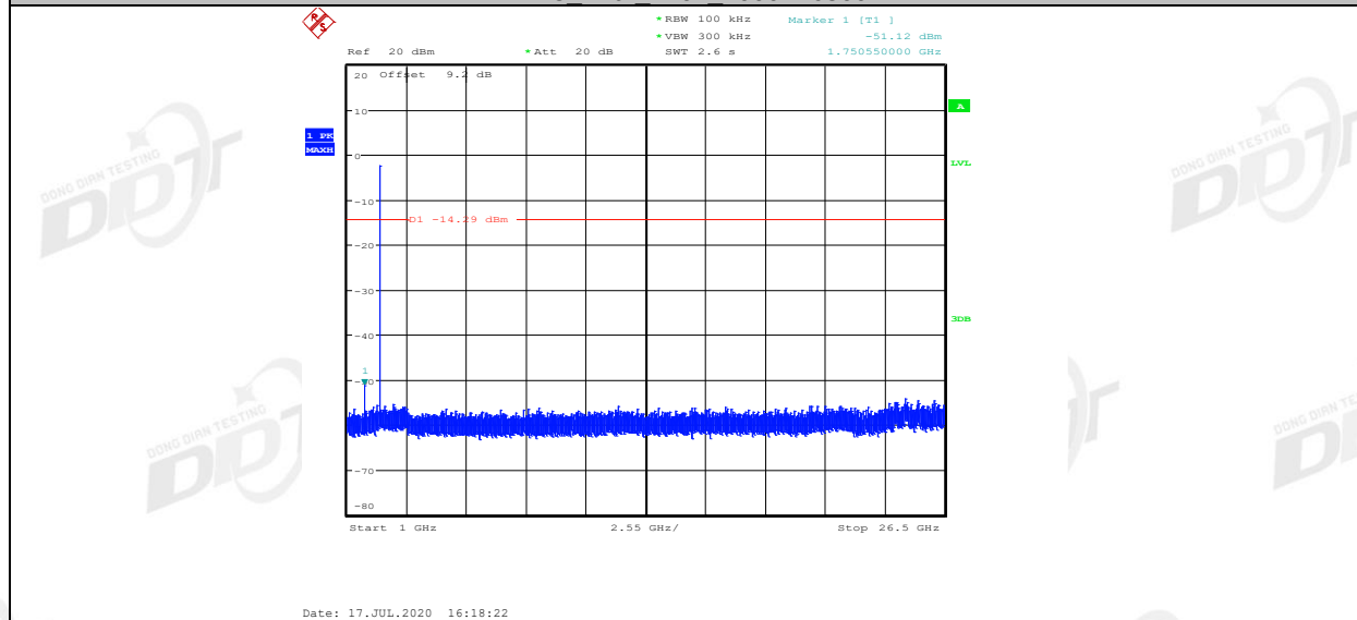
2DH5_Ant1_2441_0-Reference
