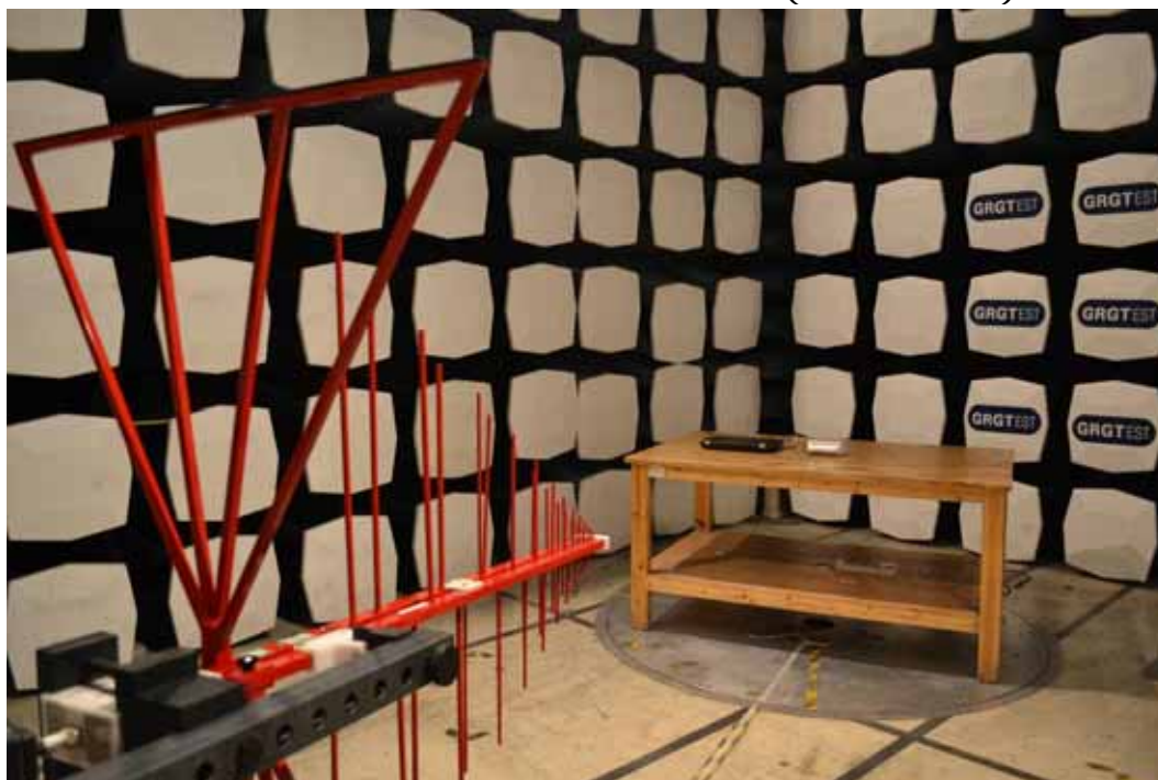
RADIATED SPURIOUS EMISSION TEST ( Below 1GHz )
