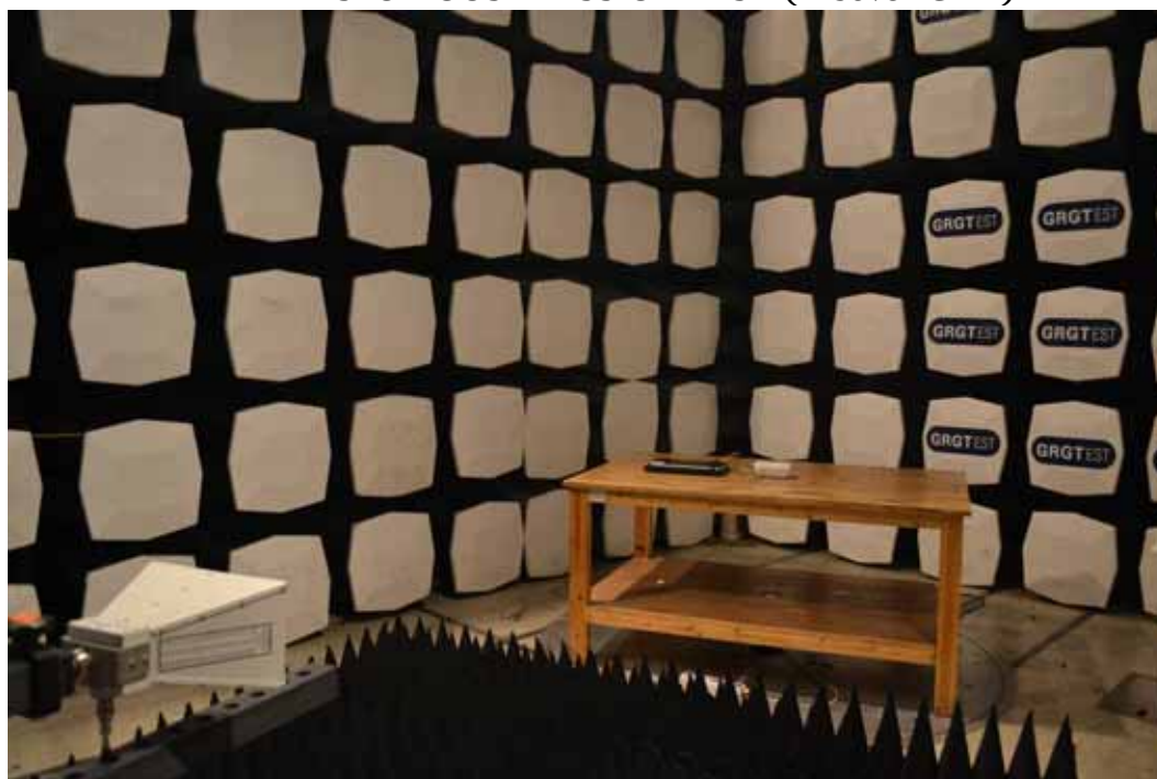
RADIATED SPURIOUS EMISSION TEST ( Above 1GHz )
