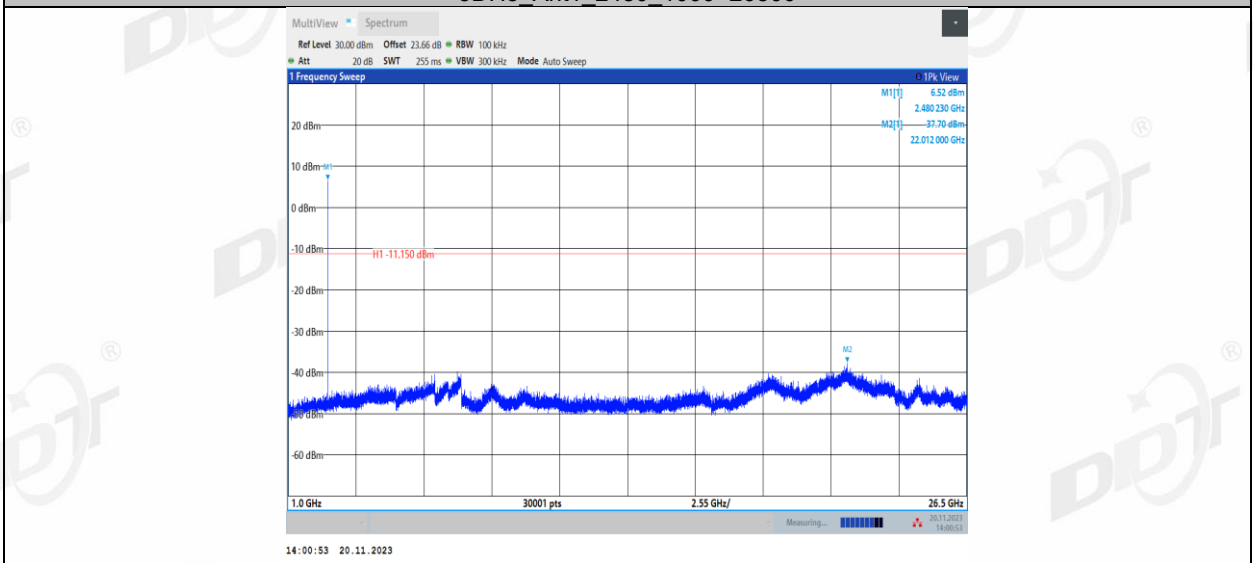
3DH5_Ant1_2480_1000~26500
