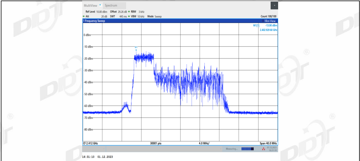
11AX20MIMO Ant1_2412_52Tone_RU38
