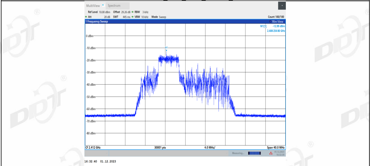
11AX20MIMO Ant1_2412_52Tone_RU39
