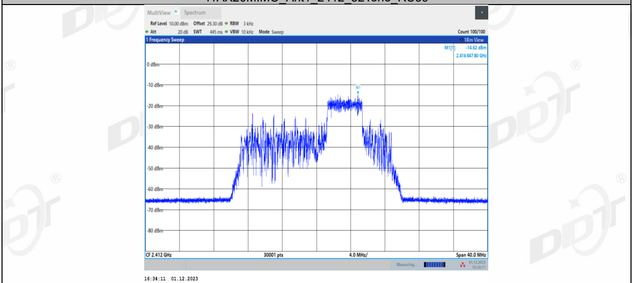
11AX20MIMO Ant1_2412_52Tone_RU40
