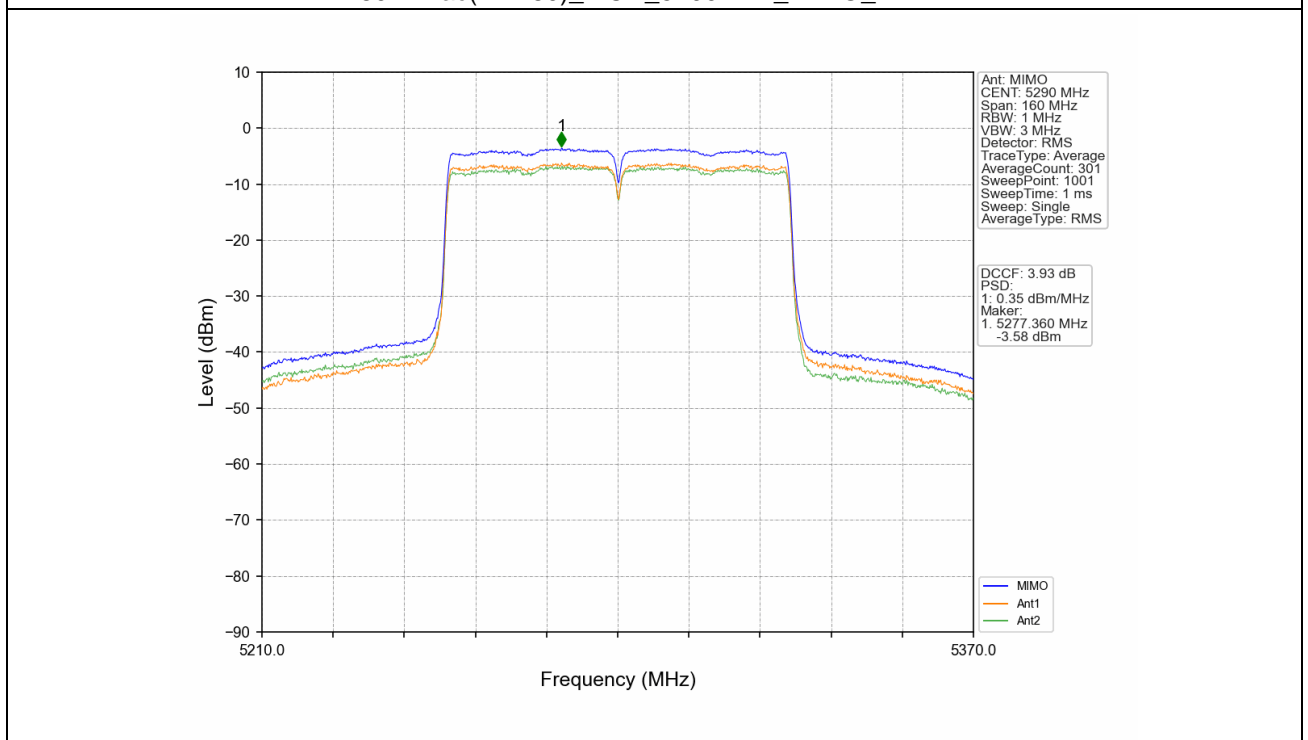
802.11ac(VHT80)_MCH_5290MHz_MIMO_NTNV
