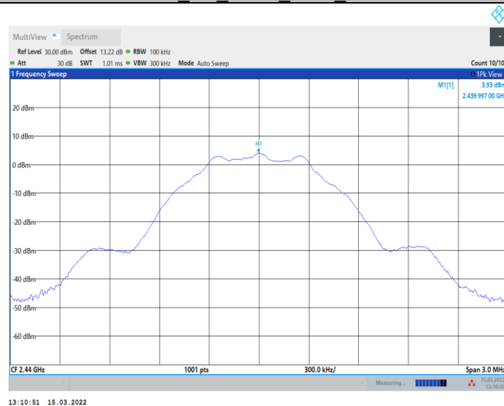
BLE_1M_ANT1_2440_30~1000
