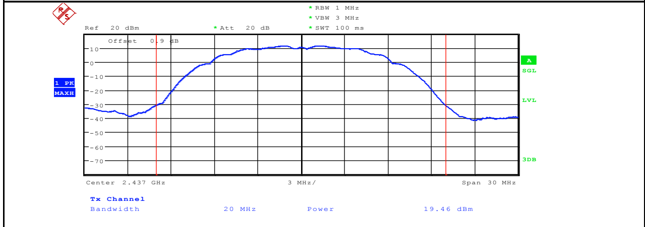
Maximum peak conducted output power_11B_2437
